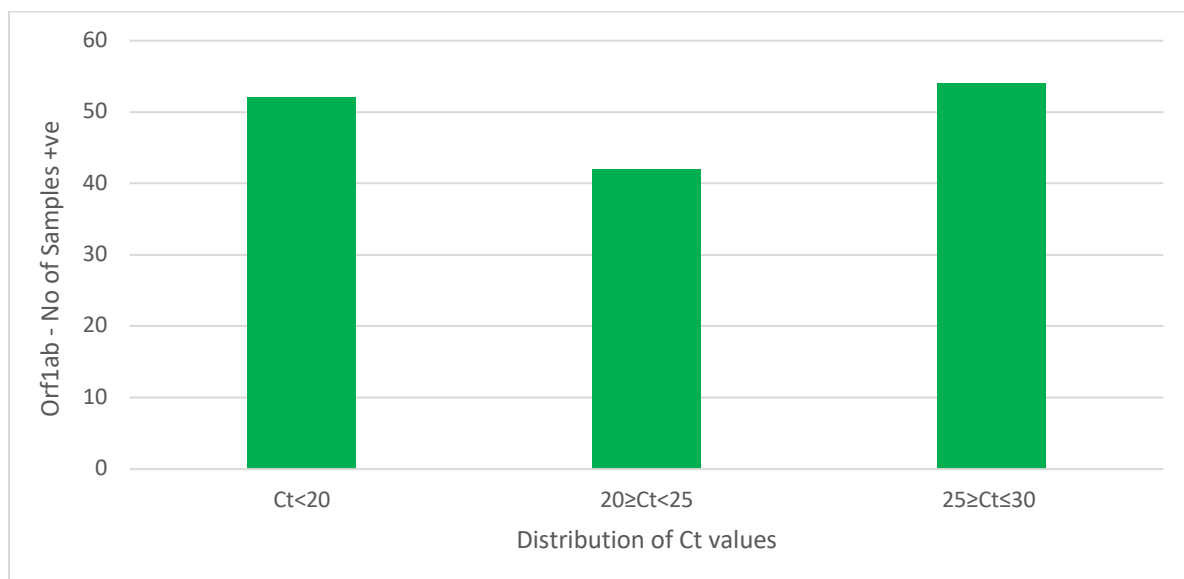
197 198 Figure 4. Distribution of TaqPath COVID-19 PCR Ct values for the Orf1ab gene. The Y-axis indicates the number 199 of samples SARS-CoV-2 positive for the Orf1ab gene. The X-axis is grouped into ranges for Ct values up to and 200 including 30. Abbreviations: Ct (Cycle threshold), Orf1ab (Open reading frame 1ab).
