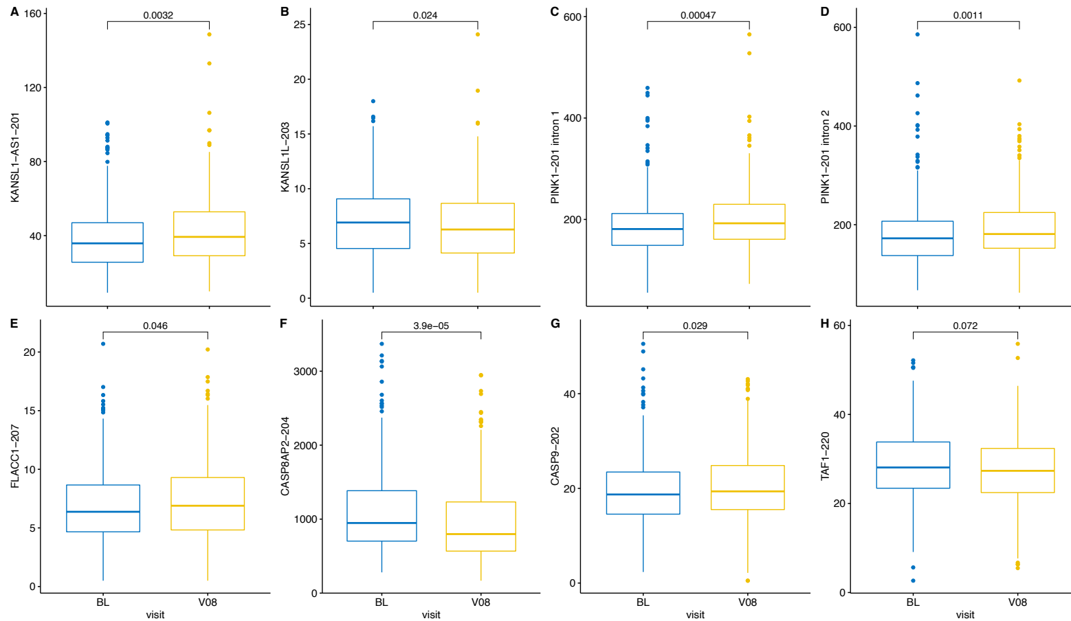
Figure 3. Longitudinal differential expression of the intronic transcripts in PD patients, BL compared to the V08 visit. The panels A, B, E, F, G, H reflect changes in the introns for different transcripts. Panels C and D illustrate changes for PINK1-201 transcripts, introns 1 and 2.
