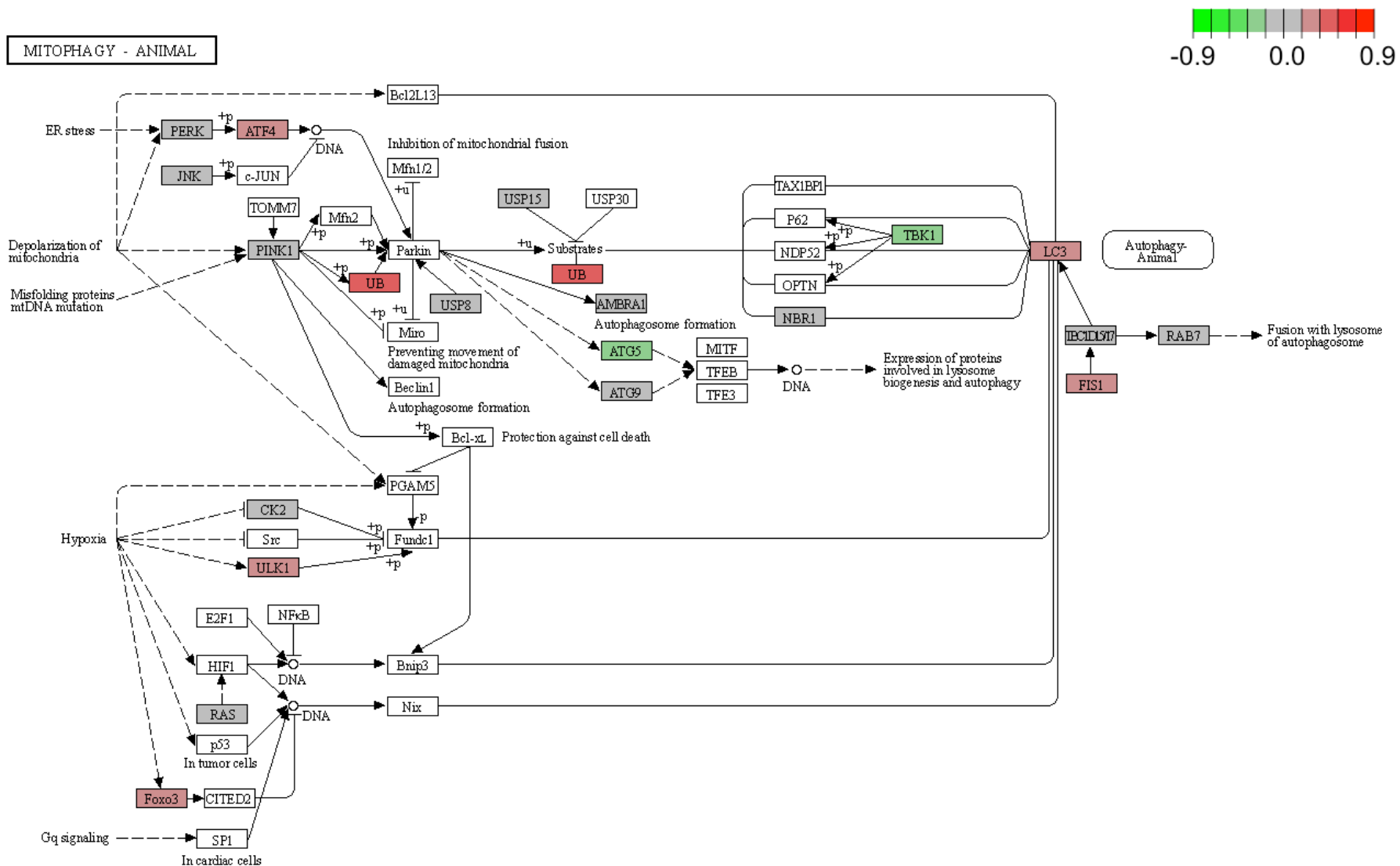
Figure 11. KEGG mitophagy pathway. Longitudinal blood intronic transcriptome profile of Parkinson disease mapped significantly to the mitophagy pathway. Mapped genes are in red, green, or grey colours.
