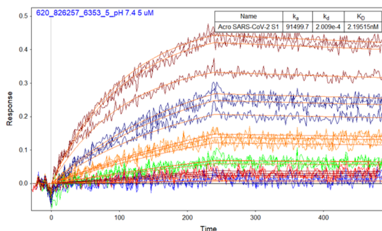
Figure 1. SPRi sensorgrams for triplicate spots of Affimer® candidate 620_826257 with injections of 100 nM – 3 nM SARS-CoV-2 S1 protein, overlaid with 1:1 Langmuir fits estimating Association rate constant ( k_a ) ( M^{-1} s^{-1} ), Dissociation rate constant ( k_d ) ( s^{-1} ), and Equilibrium dissociation constant ( K_D ) (nM).
