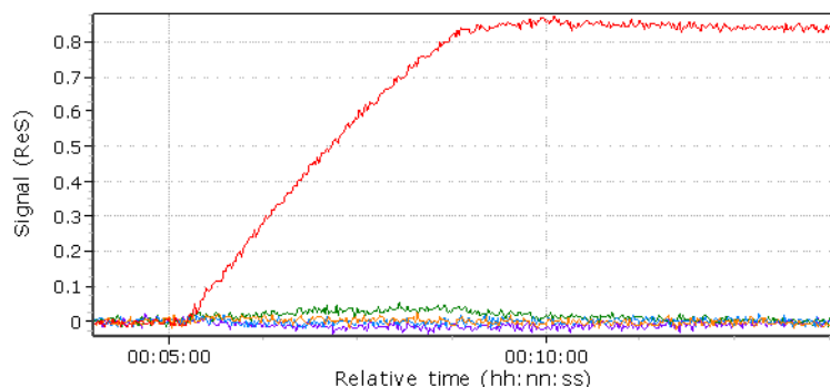
Figure 2. SPi sensorgrams for Affimer® candidate 620_826257 with injections of 50 nM SARS-CoV-2 S1 and other related human coronavirus S1 proteins: MERS-CoV S1, HCoV-HKU1 S1, SARS-CoV S1, HCoV-229E S1.
