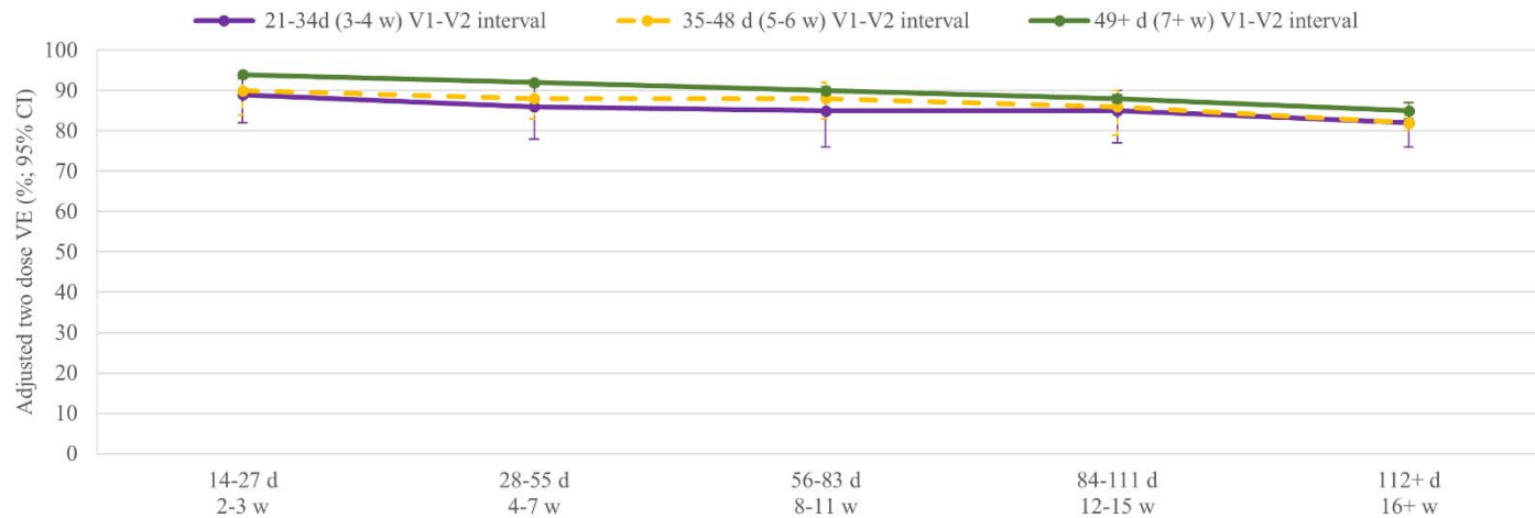
Figure 6. Adjusted two-dose vaccine effectiveness against infection by interval between doses and time since second dose, BNT162b2, \geq 18 -year-olds, British Columbia and Quebec, Canada
