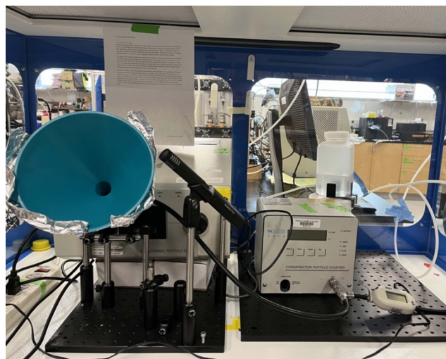
Figure 1: Experimental setup to measure the concentration of respiratory particles emitted while speaking.
