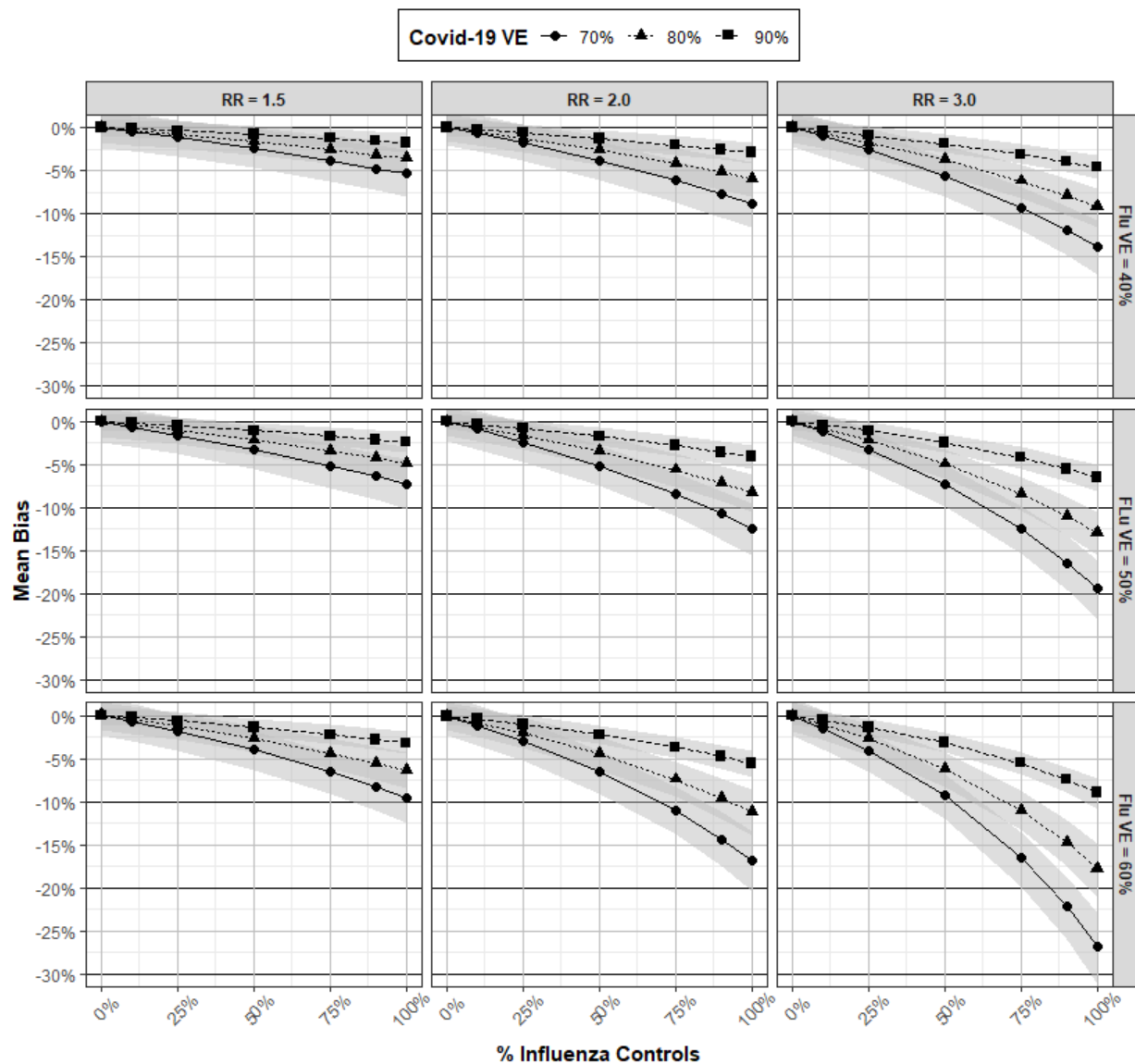
Figure 2. Mean bias and 95% confidence intervals (CI) in COVID-19 vaccine effectiveness (VE) estimates derived from a test-negative study with influenza controls under varying scenarios of RR_{covid\ vx|flu\ vx} , VE_{flu} , VE_{covid} , and P_{controls} .
