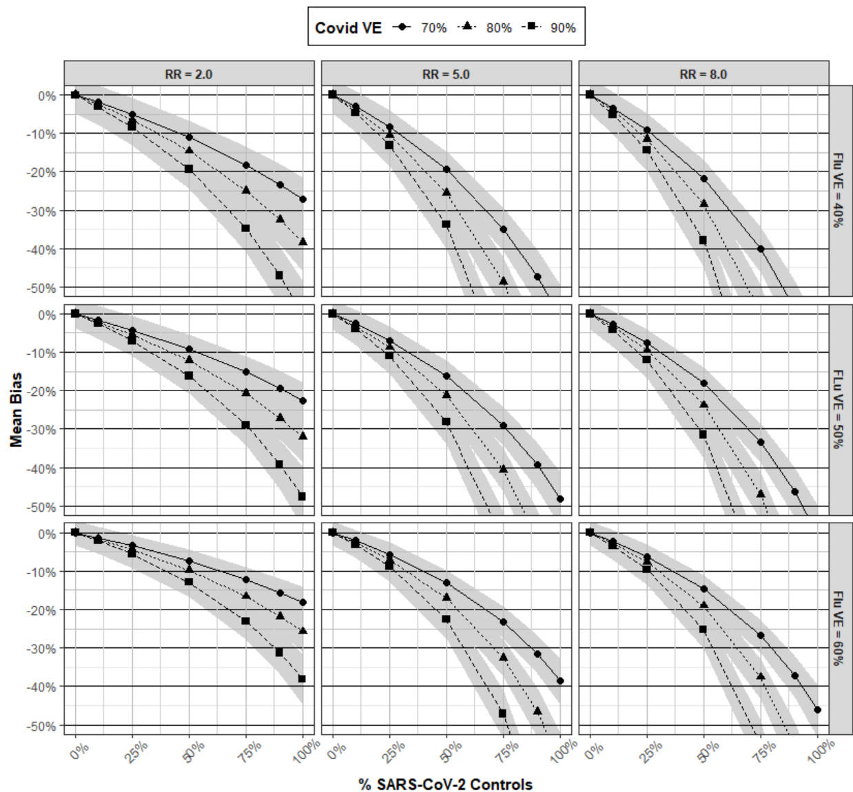
Figure 3. Mean bias and 95% confidence intervals (CI) in influenza vaccine effectiveness (VE) estimates derived from a test-negative study with SARS-CoV-2 controls under varying scenarios of RR_{flu\ vx|covid\ vx} , VE_{flu} , VE_{covid} , and P_{controls} .
