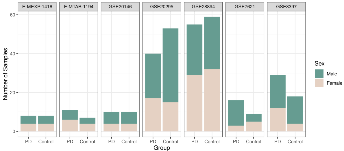
Figure 2. Number of samples per study, divided by sex and experimental group (PD – Parkinson's Disease samples).
