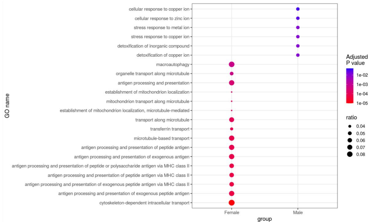
Figure 4. Summary dot plot of GO Biological Processes meta-analysis results. Only those significant functions with a highest differential effect are shown (top 16 functions in females by adjusted p-value and the only 6 significant functions in males).
