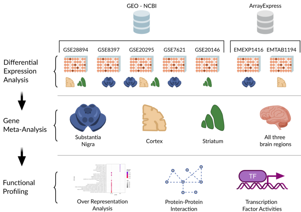
Figure 6. Workflow and analysis design. All studies were retrieved from GEO-NCBI and ArrayExpress data repositories. After data exploration and preprocessing, differential expression analysis (DEA) was performed on each selected study, getting as many contrasts as brain regions contained and an additional contrast for the whole set of samples. DEA results were combined in four different gene meta-analyses: SN, CT, ST and all regions combined. Finally, several functional profiling methodologies were applied to characterize SN meta-analysis results.
