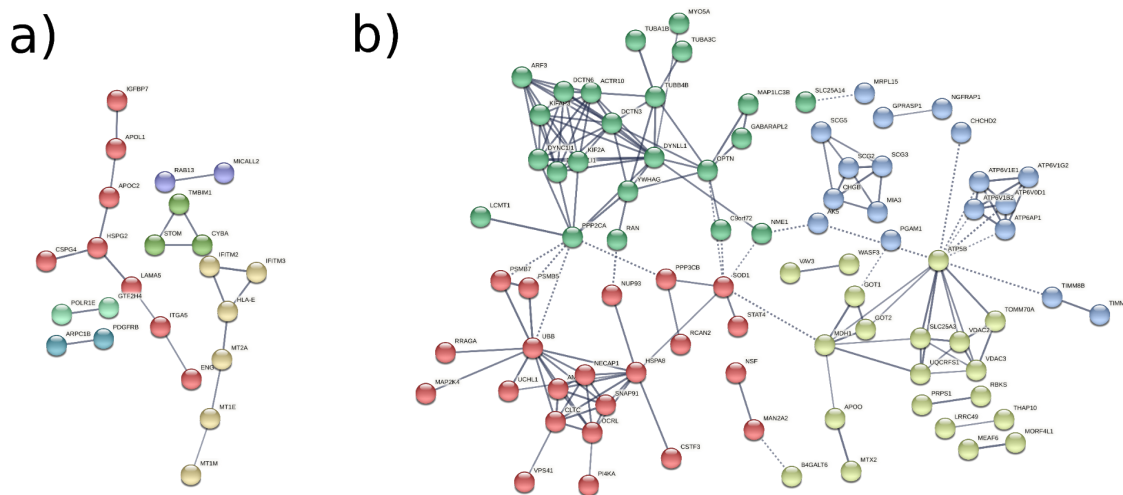
Figure 5. Protein-protein interaction (PPI) networks calculated from significant genes in SN meta-analysis. Only network edges with an interaction score greater than 0.7 are represented. a) PPI network generated from over-expressed genes in males (link). b) PPI network generated from over-expressed genes in females (link).
