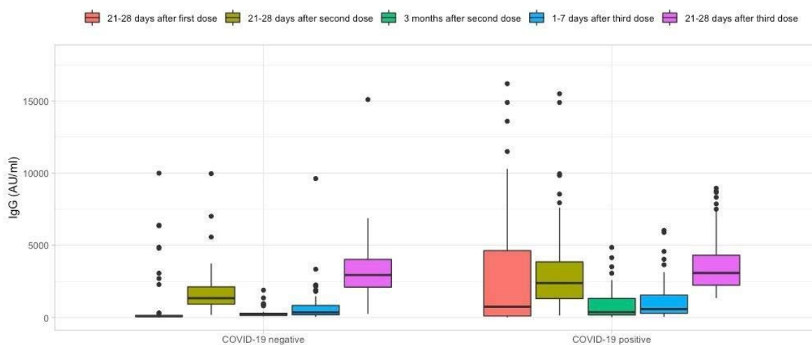
Figure 1. Box plot scheme of the quantitative SARS-CoV-2 spike 1-2 IgG antibody titers by SARS-CoV-2 history.
