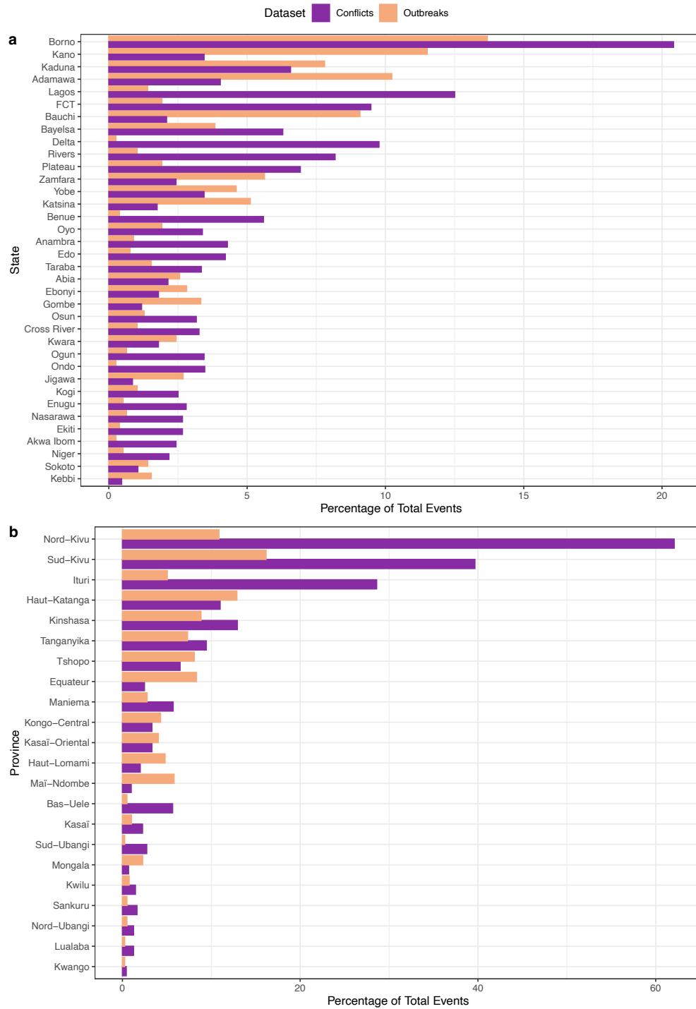
162 Figure 2. Percentage of events in each dataset including conflict and outbreaks. For a , Nigeria 163 and b , the Democratic Republic of Congo by administrative level 1. FCT - Federal Capital 164 Territory.
