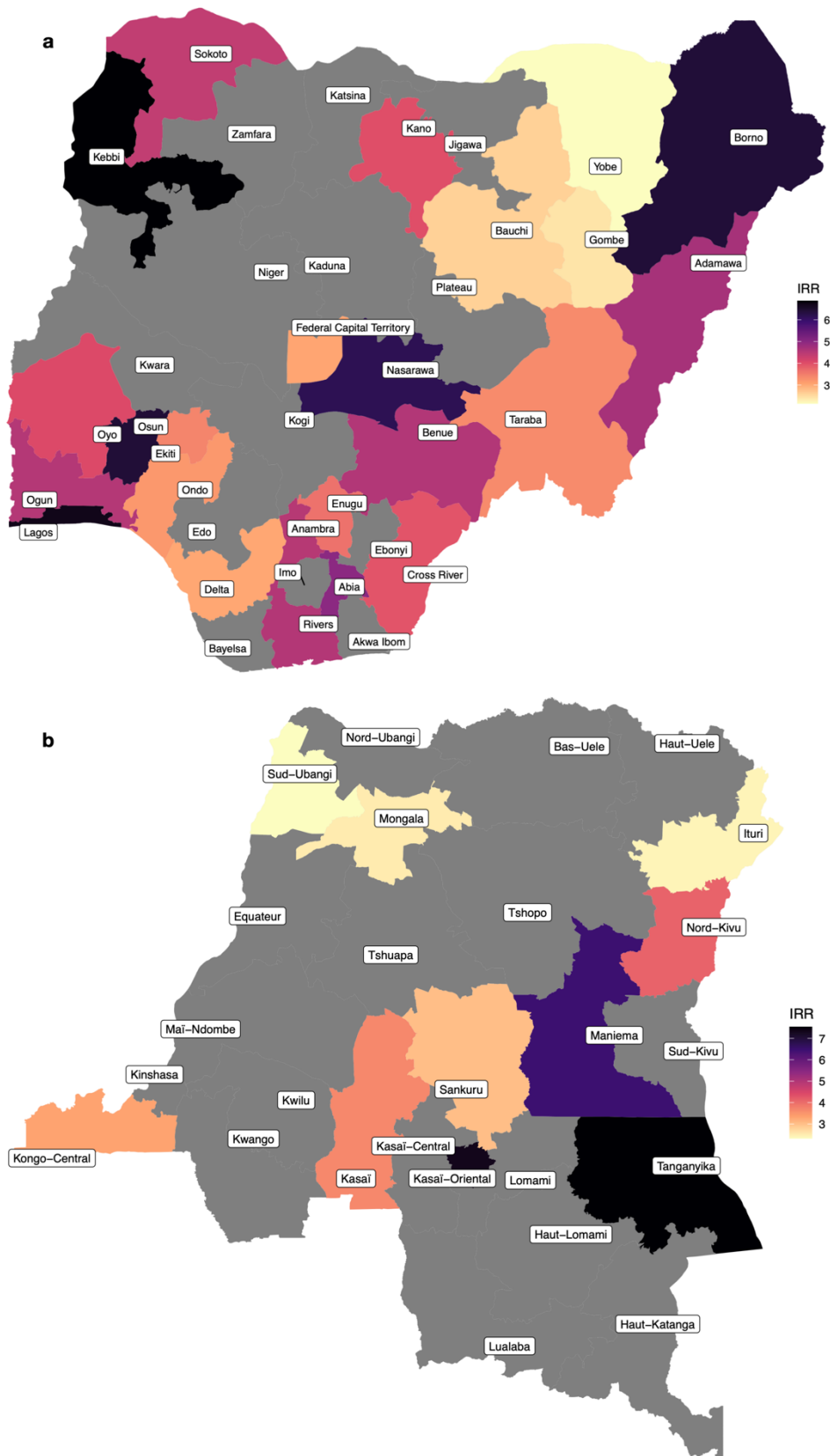
197 Figure 4. Incidence rate ratio (IRR) for the effect of exposure to conflict within one week of 198 the event and cholera at a sub-national level. For a, Nigeria and b, the Democratic Republic of 199 Congo. Only results that were significant at the threshold p < 0.05 are plotted here.
