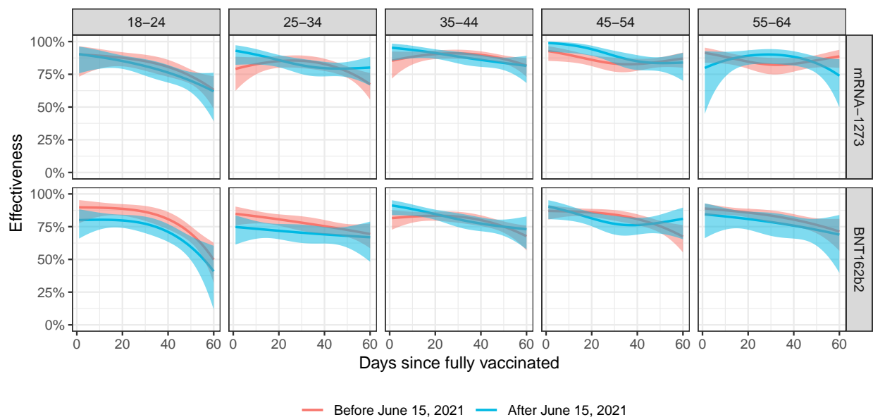
Figure S2: Time varying effectiveness estimates by age group and vaccine manufacturer before and after arrival of the Delta variant. The ribbons represent point-wise 99% confidence intervals.
