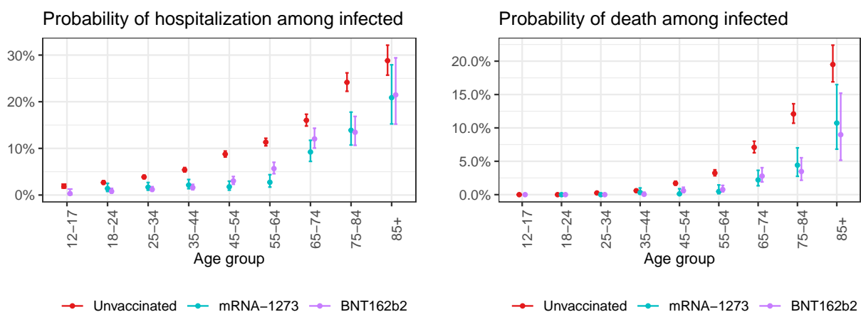
Figure 4: Estimated probability of hospitalizations and deaths from COVID-19 among individuals infected with SARS-CoV-2 with 95% confidence intervals. Two vaccinated groups are compared to unvaccinated with the different vaccination manufacturers denoted with color. Note that not all hospitalizations are reported to the BioPortal database.
