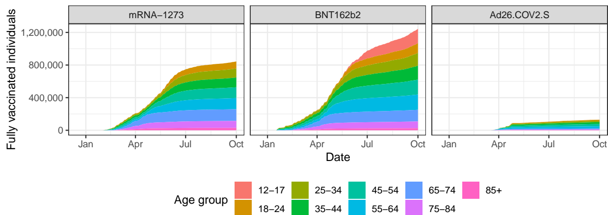
Figure S1: Total number of fully vaccinated individuals by age group and vaccine manufacturer. Each pane represents a vaccine manufacturer and colors represent the different age groups.
