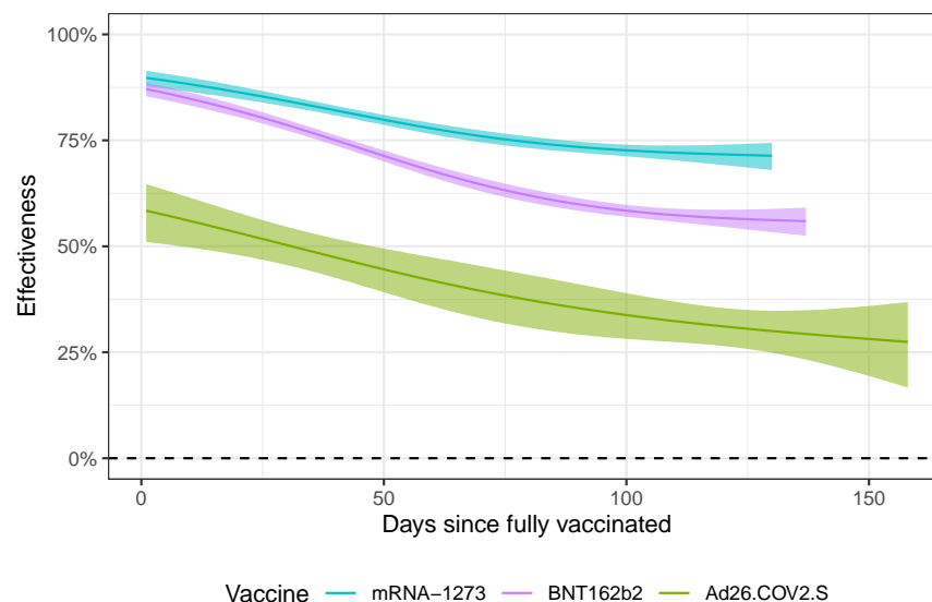
Figure 3: Vaccine effectiveness through time. The estimated effectiveness is plotted against days since the individuals were fully vaccinated. The ribbons represent point-wise 99% confidence intervals. The different vaccine manufacturers are denoted in different colors.
