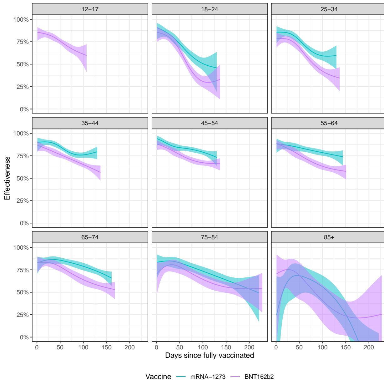
Figure S3: Waning effectiveness against infection by age group and vaccine manufacturer (colors). The ribbons represent point-wise 99% confidence intervals.
