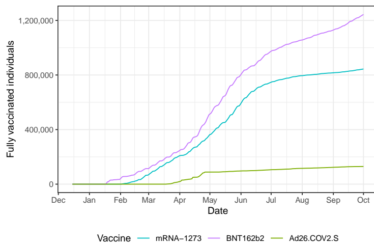
Figure 1: Total number of fully vaccinated individuals per day by vaccine manufacturer (represented with different colors).
