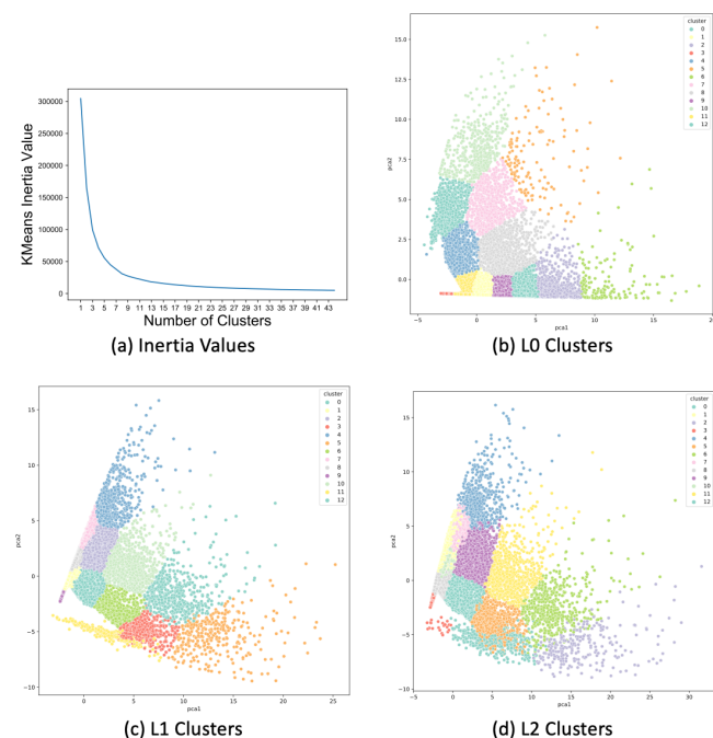
Figure 4. K-means inertia scores and clustering
