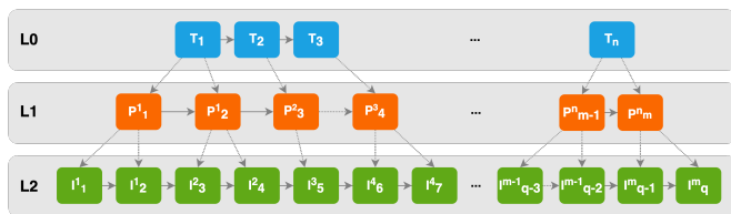
Figure 1. Illustration of Hi-RISE ( H ierarchical R epresentation of I ntervention S equences). L0 represents the sequence of provider types ( T_1 \dots T_n ), L1 represents the sequences of actual provider encounters ( P_1^1 \dots P_m^m ), and L2 represents sequences of interventions ( I_1^1 \dots I_q^m ).
