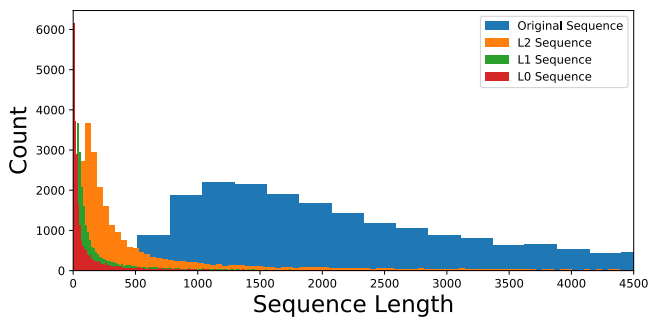
Figure 3. Histograms of sequence lengths of the original intervention sequence and Hi-RISE’s L0, L1, and L2 sequence representations.
