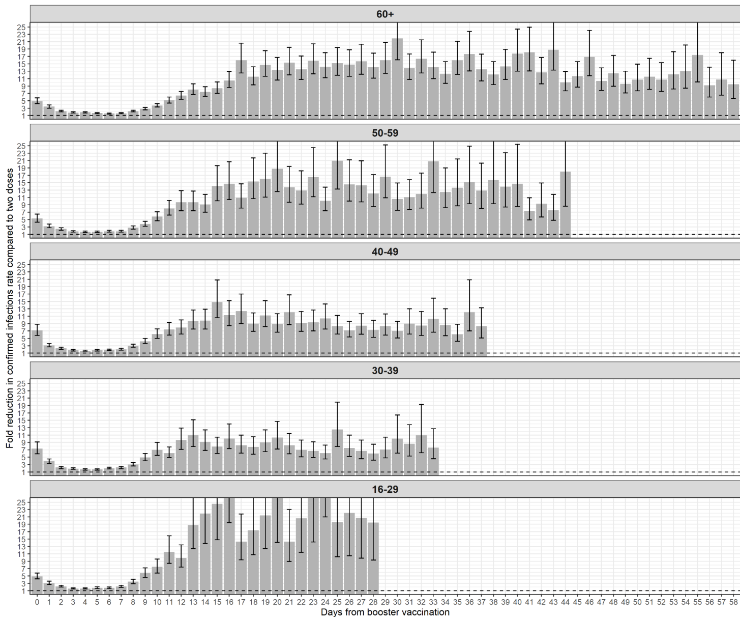
Figure 2. The fold reduction in the rate of confirmed infections in the booster group compared to the nonbooster group as a function of the number of days following the booster dose (day 0 = day receiving the booster dose), for the different age groups. The dashed line represents no added protection by the booster dose. Error bars are 95% confidence intervals not corrected for multiplicity.
