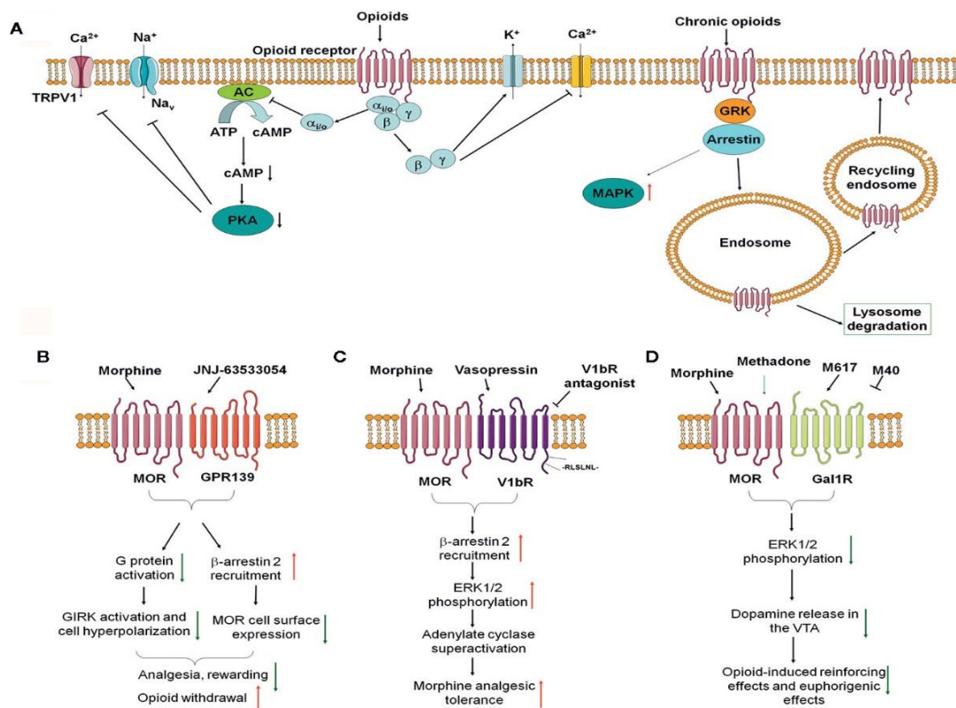
Figure 1. Opioid Receptor Signaling. (Zhang et al., 2020)
