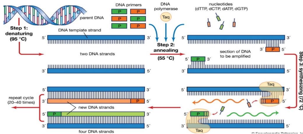
Figure 6. Polymerase Chain Reaction (Britannica, 2019)
