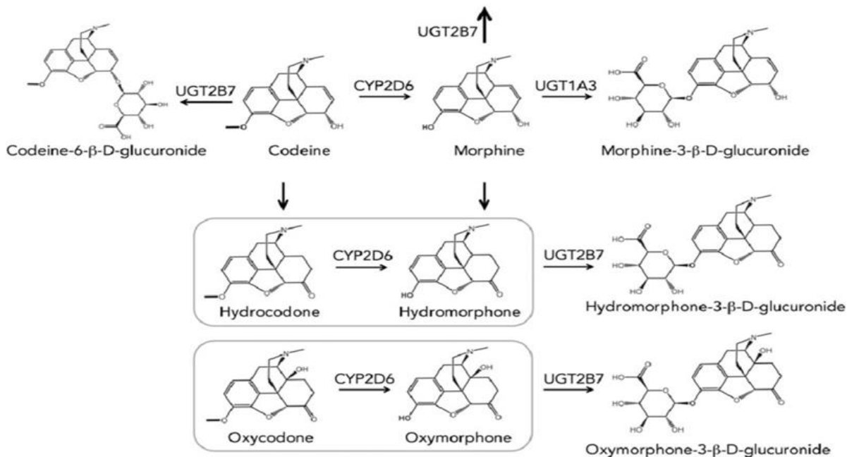
Figure 3. Opioid Degradation by CYP2D6 (Marinova et al., 2016)
