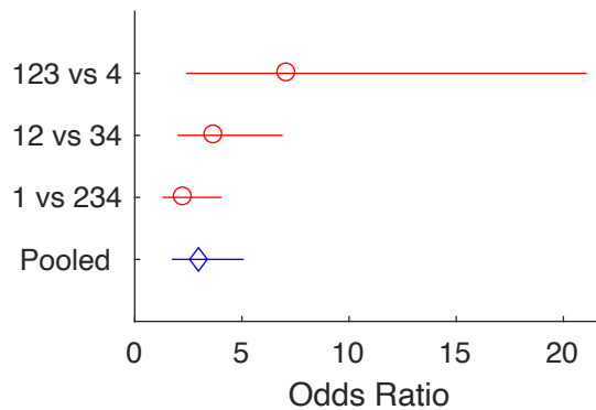
Figure 2: Odds ratios for binary vs. pooled ordinal logistic regression. Predicted odds ratios (with 95% confidence interval) are displayed for the three possible binary logistic regressions, compared to the pooled odds ratio from ordinal logistic regression. The pooled odds ratio of 2.97 is contained within the 95% confidence interval for each binary logistic regression, indicating that the pooled odds ratio assumption does not appear to be violated.
