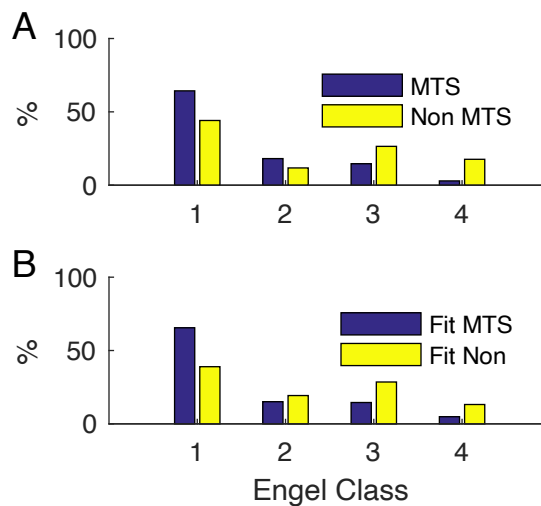
Figure 1: Results of ordinal logistic regression. (A) Observed percentages of Engel outcomes I-IV stratified by presence or absence of mesial temporal sclerosis (MTS), pooled from 8 studies. (B) Predicted percentages of Engel I-IV stratified by MTS or not, using ordinal logistic regression. The pooled odds ratio assumption means the predicted difference in Engel I for MTS or not (65% vs. 39%) is slightly higher than observed (64 vs. 44%), but the predicted difference for Engel IV for MTS or not (5% vs. 13%) is smaller than observed (3% vs. 18%).
