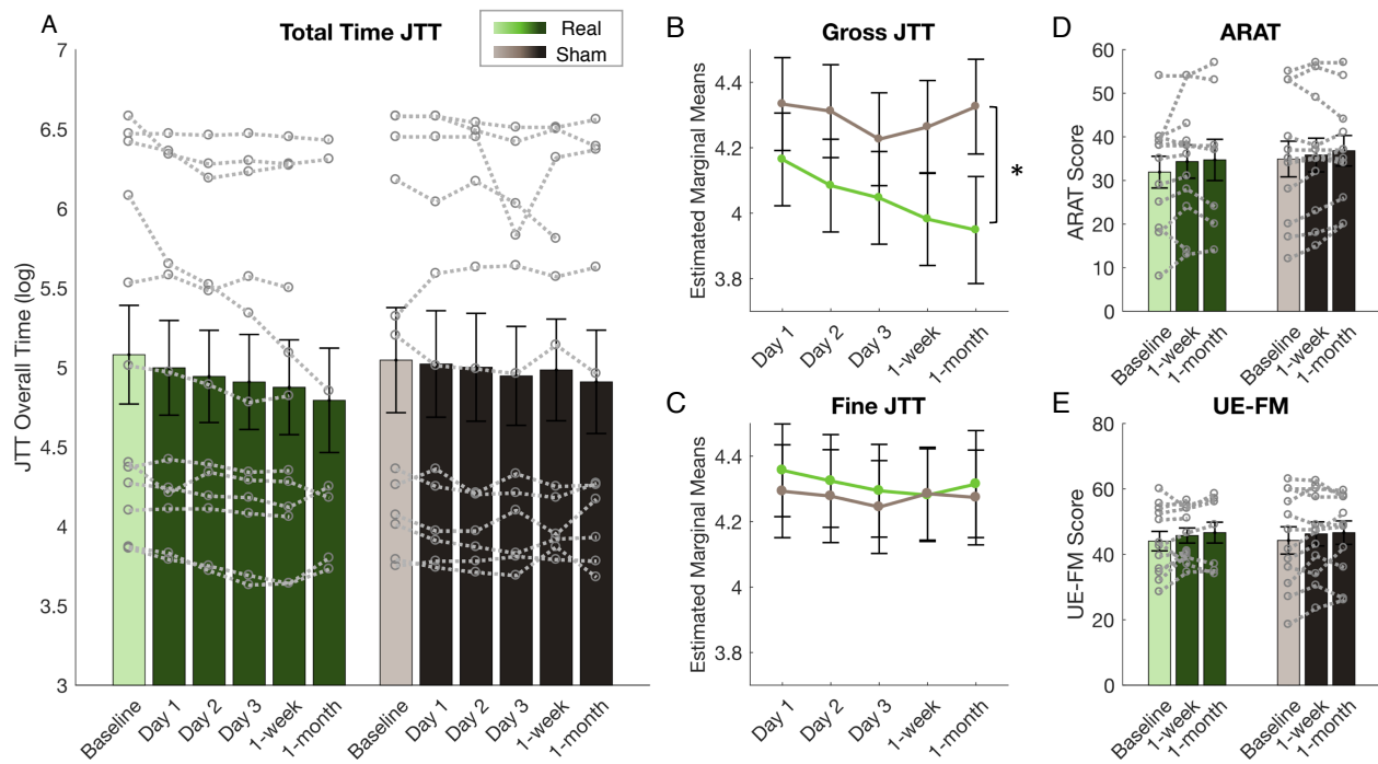
Figure 3: Participants in Real group improve on Gross motor performance (JTT) compared to Sham. (A)
