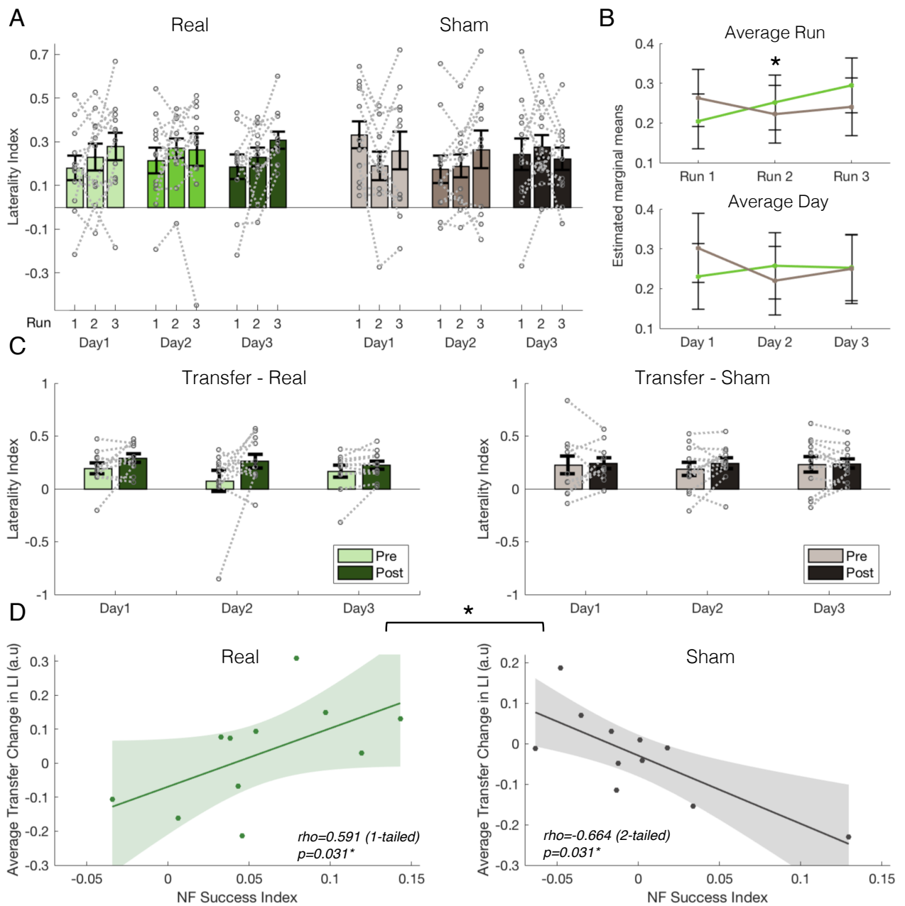
Figure 2: NF learning occurs within training days and better learning is associated with transfer success. (A)
