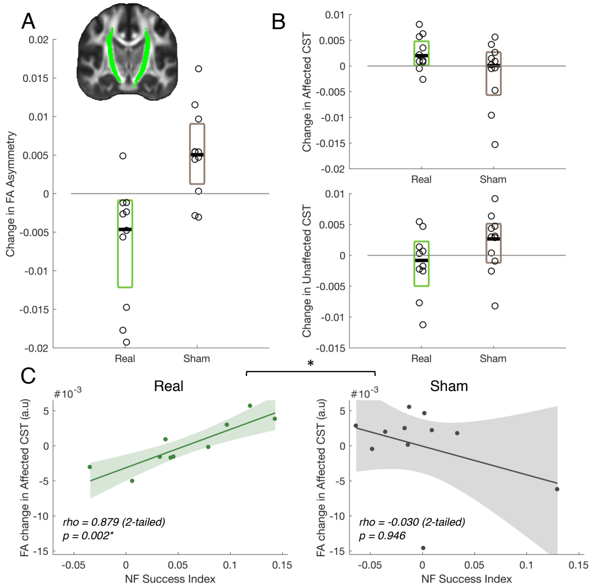
Figure 4: FA Asymmetry of CSTs is reduced after Real NF training. (A) The Real group (n=10) had lower FA asymmetry in the CSTs (shown in inset) after NF training compared to the Sham group (n=11). Change in FA asymmetry between baseline and 1-week follow-up is plotted for the Real (green) and the Sham (grey) group. The black line represents median change, colored boxes represent 95% confidence intervals and individual participant data points are shown with open circles. (B) The same information is shown for FA change between baseline and 1-week follow-up in the affected (top) and unaffected (bottom) CSTs. (C) Neurofeedback success was positively correlated with FA change in the stroke affected hemisphere in the Real group, whereas no correlation was found in the Sham group with the two correlations being significantly different from each other ( p = 0.004 ). * p < 0.05
