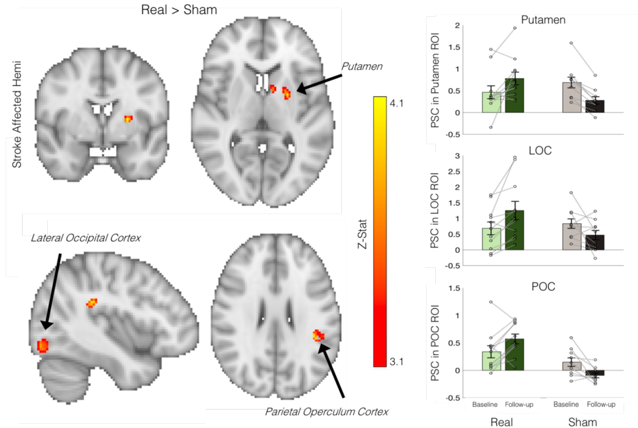
Figure 5: Increased activity in brain regions associated with NF learning. Changes in brain activity before and after NF or Sham training were assessed during a controlled visuomotor squeeze task. Three significant clusters were found where the Real group had greater change in activity following NF than the Sham group (Real>Sham, voxelwise GLM, p < 0.05 , corrected), located in the putamen, lateral occipital cortex (LOC) and the parietal operculum cortex (POC) of the unaffected hemisphere. For visualization purposes, the mean percent signal change (PSC) of the significant clusters is plotted on the right, as well as the data from individual participants (represented by open circles). Error bars represent s.e.m.
