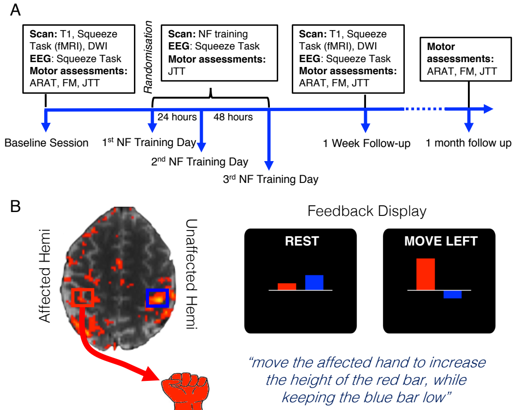
Figure 1: Study design and timeline. (A) Participants attended three NF training sessions separated by 24 and 48 hours, a baseline session and two follow-up sessions at 1-week and 1-month post NF training. (B) Left: Regions of interest (ROIs) used for NF training were defined during a functional localizer. ROIs (red and blue squares) were centered on peak activity in M1 during movements of both hands. Right: During NF training, only the stroke-affected hand was moved and participants viewed two bars on the screen. The red bar represented activity in the stroke affected hemisphere and the blue bar represented activity in the unaffected hemisphere. During movement blocks, participants were instructed to make movements with their stroke affected hand to increase the size of the red bar, while keeping the blue bar as low as possible.
