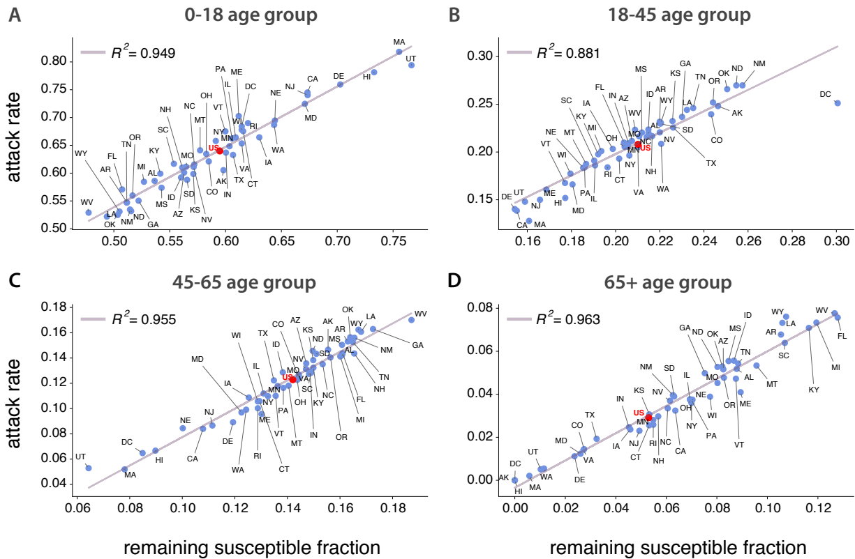
FIG. 6. Scatter plot of attack rates during the second outbreak versus the remaining susceptible fraction for every US state. Top-left (A): 0-18 years old group. Top-right (B): 18-45 years old group. Bottom-left (C): 45-65 years old group. Bottom-right (D): over 65 years old group. Results also shown for a simulation of the epidemic for the whole country as if it were a single age-structured population (red dot). These high correlations show also the relevant role of age structure in the disease propagation.
