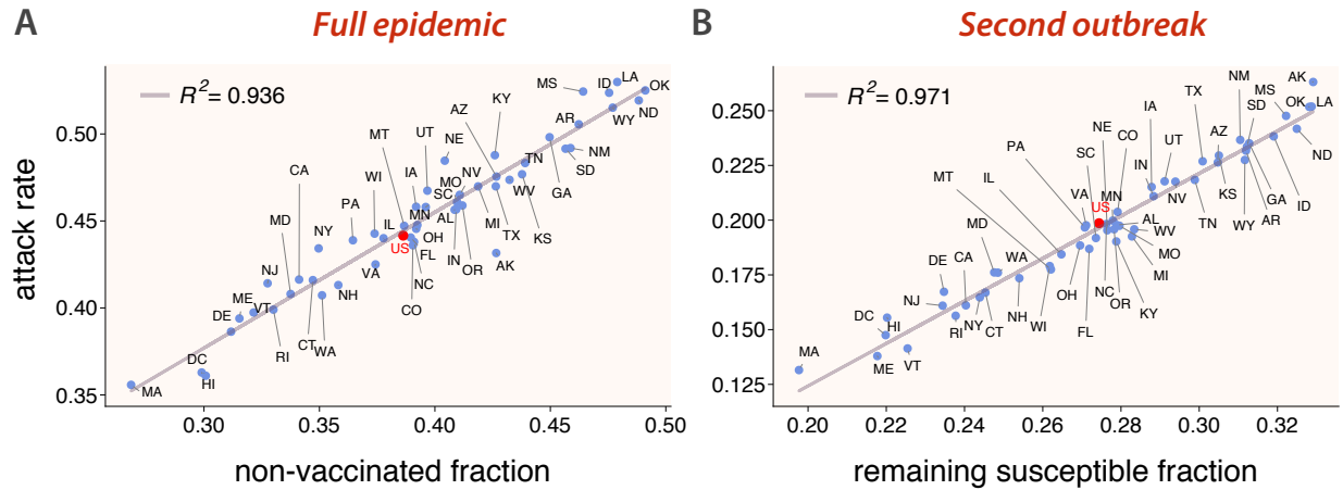
FIG. 3. Scatter plot of attack rates after the full epidemic (first outbreak with R_0 = 1.5 and the second one with R_0 = 6 ) versus the non-vaccinated fraction of individuals (A), and attack rates of the second outbreak ( R_0 = 6 ) versus the remaining susceptible fraction after the first outbreak (B) for every US state. The red dot corresponds a simulation on a population representing the whole country. It is clearly seen that higher hesitancy translates into higher attack rates.
