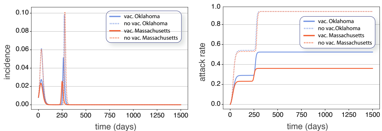
FIG. 2. Comparison of peak incidences and final epidemic sizes for the states of Oklahoma (OK), which has the highest vaccine hesitancy, and Massachusetts (MA), where the vaccine hesitancy is the lowest according to surveys [39]. Continuous trajectories (blue and red) represent the simulation with vaccination campaign, whereas dotted trajectories represent the simulation without introducing the vaccination campaign. All simulations started with a fully susceptible population.
