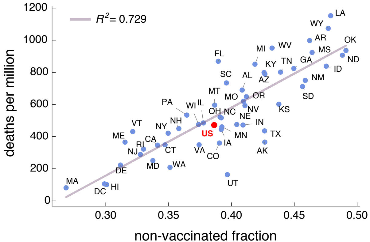
FIG. 5. Scatter plot of deaths per million during the second outbreak versus the non-vaccinated fraction at the end of the first outbreak for every US state. Results also shown for a simulation of the epidemic for the whole country as if it were a single age-structured population (red dot). The model does not include deaths as part of the dynamics, but they can be estimated by applying the infection fatality rate to the final fraction of individuals in the removed compartment for each age class (eq. (5)).
