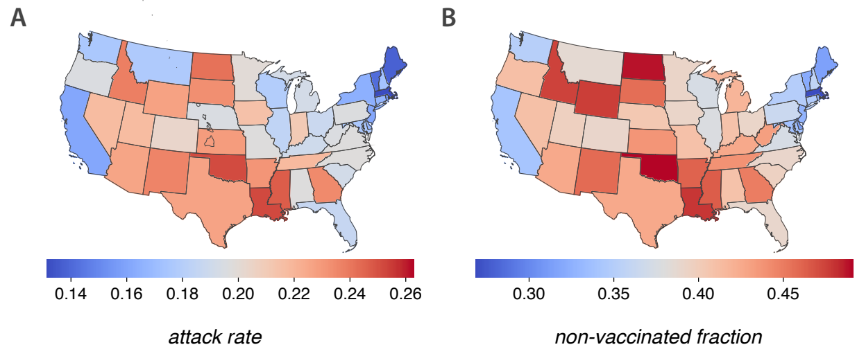
FIG. 4. Representation on the US map of the attack rates of every state after the end of the epidemic trajectory proposed in this paper (A), and the fraction of non-vaccinated individuals (B). Some spatial clustering can be appreciated along the country, even though in the simulations all states are completely isolated.
