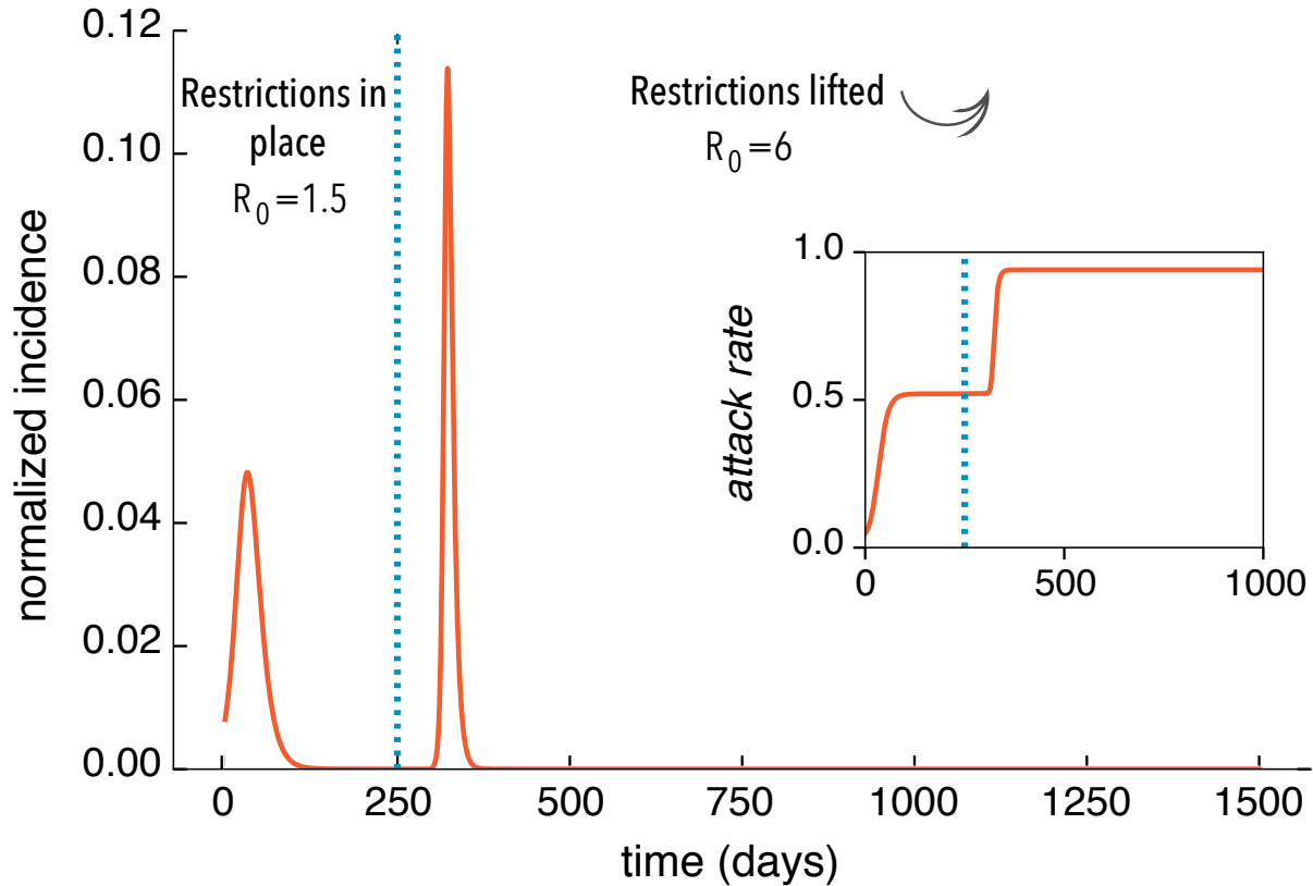
FIG. 1. Proposed baseline scenario: following the first wave of the epidemic, part of the population acquires natural immunity. Then, we simulate the propagation of a mitigated outbreak due to the presence of some restrictions, social distancing and prophylaxis measures, leading to a slower propagation of the original variant of the disease ( R_0 = 1.5 ). After the outbreak extinguishes a back-to-normal situation is assumed and all prevention measures are lifted. Then, an outbreak is seeded again with a higher basic reproductive number, R_0 = 6 . On top of this baseline scenario, we will introduce a vaccination campaign during the first outbreak and explore the impact of vaccination hesitancy on the second outbreak.
