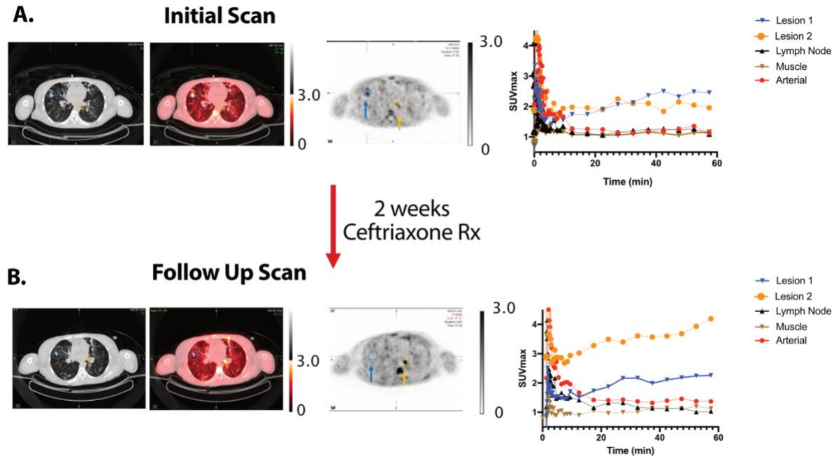
Figure 4. Time activity curves and bacterial heterogeneity. [ ^{11}\text{C} ]-TMP PET/CT images were acquired of a woman in her 40's with an acute exacerbation of cystic fibrosis before A ) and after treatment with 2 weeks of intravenous ceftriaxone B ) Regions of interest were drawn around two separate pulmonary airspace opacities. In addition, reference regions were also drawn around a reference lymph node, paraspinal musculature, and within the aorta. Comparing the PET/CT images before and after treatment, the visible changes in relative [ ^{11}\text{C} ]-TMP uptake in lesion 1 versus lesion 2 demonstrate the bacterial heterogeneity and an apparent new infection with S. aureus based on sputum cultures. Patient received 487 MBq and 780 MBq of [ ^{11}\text{C} ]-TMP at the first and second time points, respectively.
