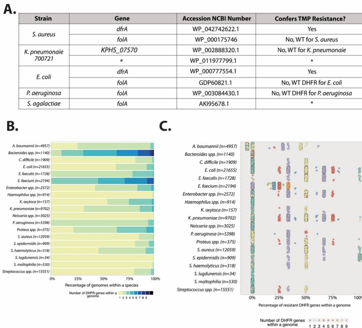
Figure 2. Whole genome sequencing characterization of lab and clinical isolates strains and bioinformatic analysis of clinically relevant bacteria. A) Table of DHFR open reading frames showing that most strains carried a DHFR copy known to bind TMP. * Denotes no literature found on these DHFR genes B) Proportion of clinically relevant bacterial strains from the NCBI RefSeq database with the indicated number of DHFR genes per genome. C) Resistance characterization of DHFR genes in relevant bacterial strains from NCBI RefSeq database. Each dot represents a strain.
