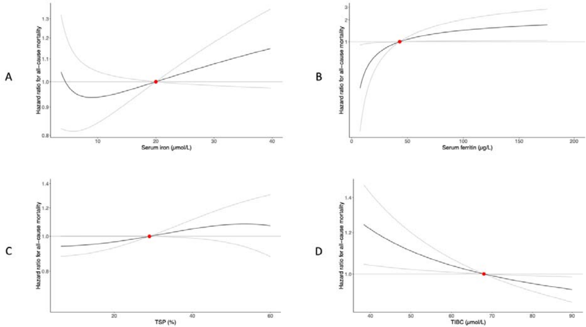
Figure 2: Non- linear Mendelian randomization: Dose-response curves (black) between iron traits and all-cause mortality in HUNT (gray lines give 95% confidence interval). The x-axis gives A: serum iron levels ( \mu\text{mol/L} ), B: serum ferritin ( \mu\text{g/L} ), C: transferrin saturation (%) and D: total iron binding capacity (TIBC) ( \mu\text{mol/L} ). The y-axis gives the hazard ratios for all-cause mortality with respect to the reference values (red dot), which represent the established target values (iron, TIBC, TSP) 51 or median value (ferritin) for the traits. The curve gradients represent the localized average causal effect at each point.
