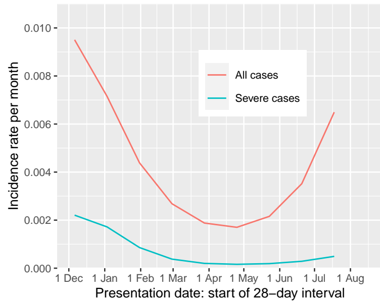
Fig 1. Fitted values for monthly incidence of any case and severe case in the shielding cohort, based on Poisson regression with spline terms for calendar time
