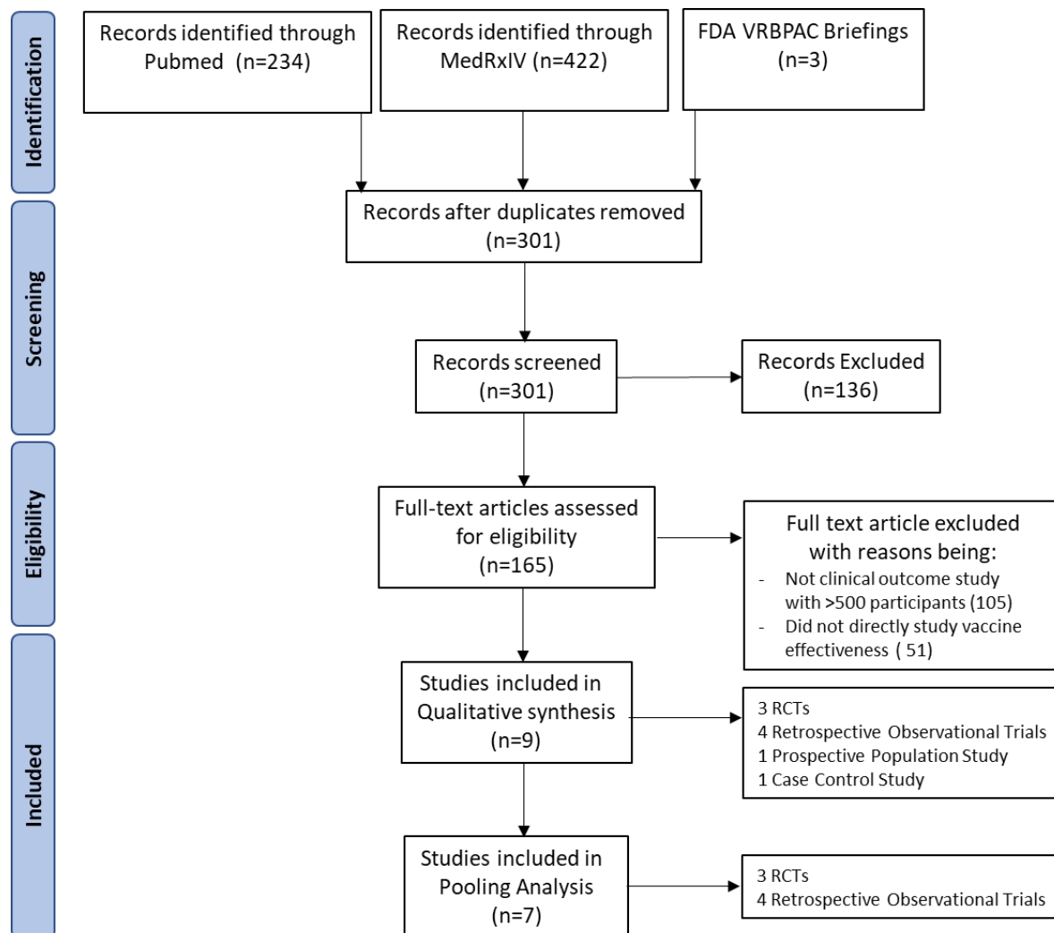
Figure 1. PRISMA flowchart
