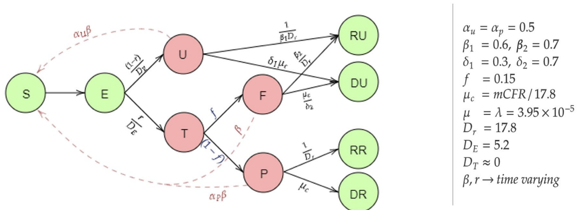
Figure S1: Schematic diagram for the SEIR-fansy model with imperfect testing and misclassification.
