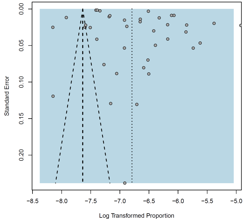
Figure 6. Funnel plot for examination of publication bias across included studies.
