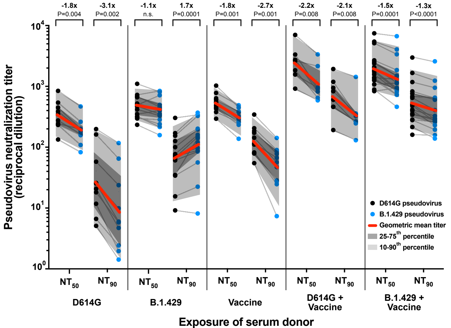
Figure 1. Plot of 50% and 90% pseudovirus neutralization titers (NT 50 and NT 90 ) of serum samples obtained from donors with the indicated infection and/or vaccination exposures. Grey lines connect neutralization titer values for D614G (black dots) and B.1.429 (blue dots) pseudoviruses within each individual serum sample. Geometric mean neutralization titers for each serum group are marked with red lines and fold-change in NT 50 and NT 90 between D614G and B.1.429 pseudoviruses is shown along with P-value. Dark grey shading marks the interquartile range of titer values in each group and light grey shading marks the 10 th -90 th percentile of the range. P-values were calculated with a Wilcoxon matched-pairs signed-rank test.
