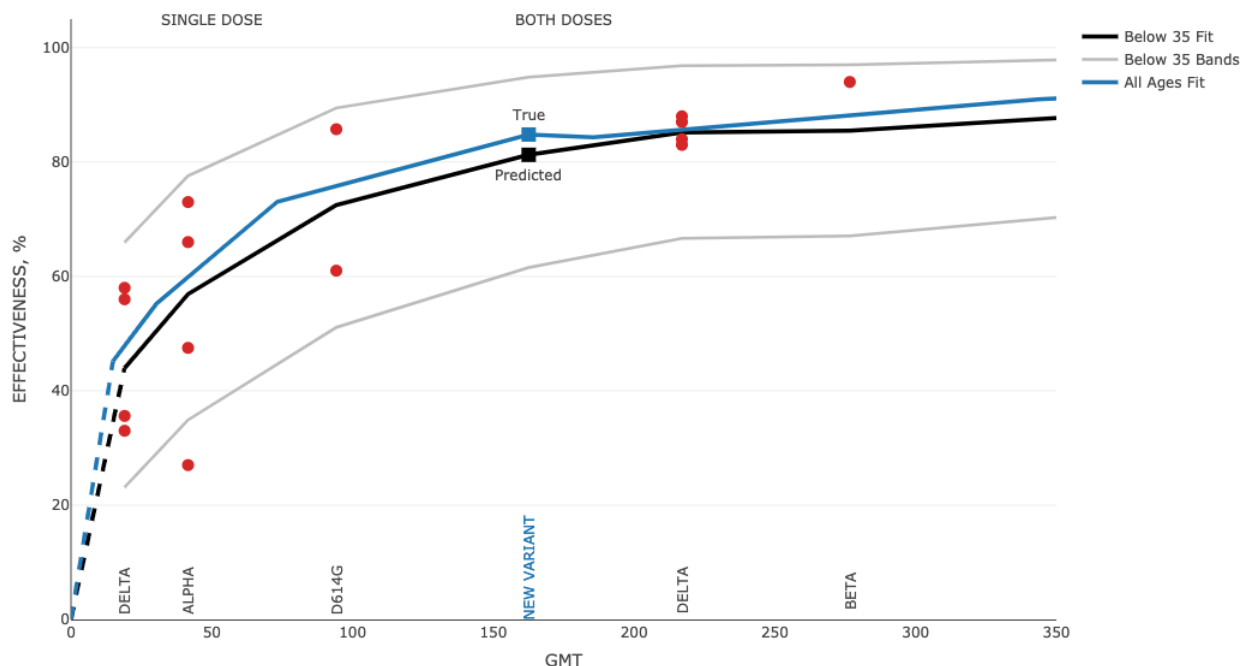
Figure 18: Cautious prediction for Comirnaty. Observations were fitted to the below 35 age group; the all-ages fit is shown for comparison. Effectiveness for a new variant was predicted for all-age titres but assuming the below-35 fit.
