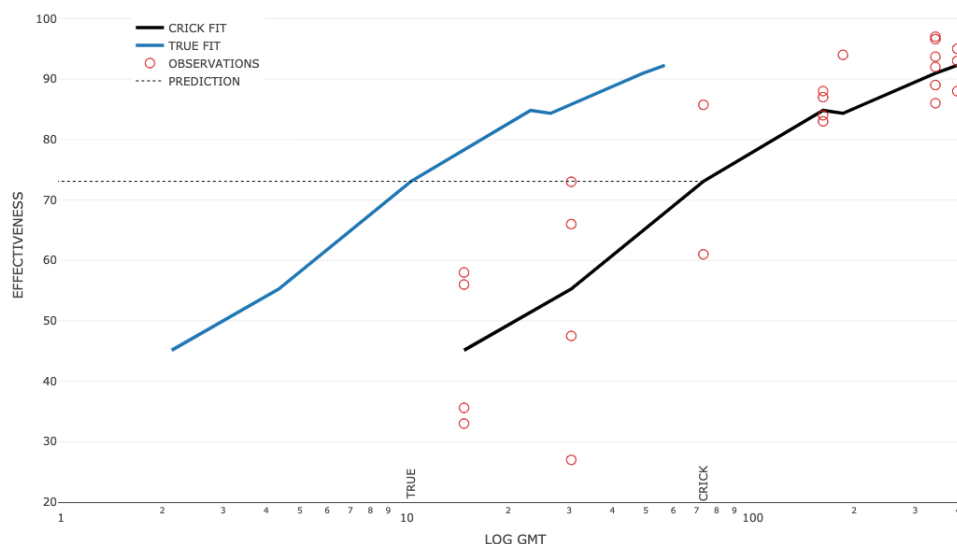
Figure 16: True distributions of titres are a constant multiple of Crick distributions
