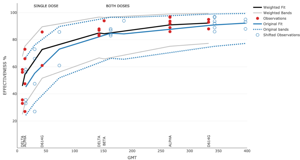
Figure 15: Model fits using age-weighted versus unweighted (original) neutralising titres from the Crick study with Comirnaty. The observations are plotted versus weighted and unweighted GMT per dose/variant. The variant labels are for weighted distributions.
