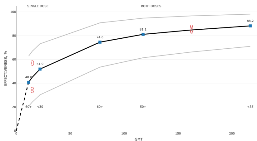
Figure 2: Predicted effectiveness of Comirnaty against the Delta variant for the indicated age groups. The model fit, the same as in Figure 1, for all ages was used for this prediction. The effectiveness observations were against Delta in all-age groups.
