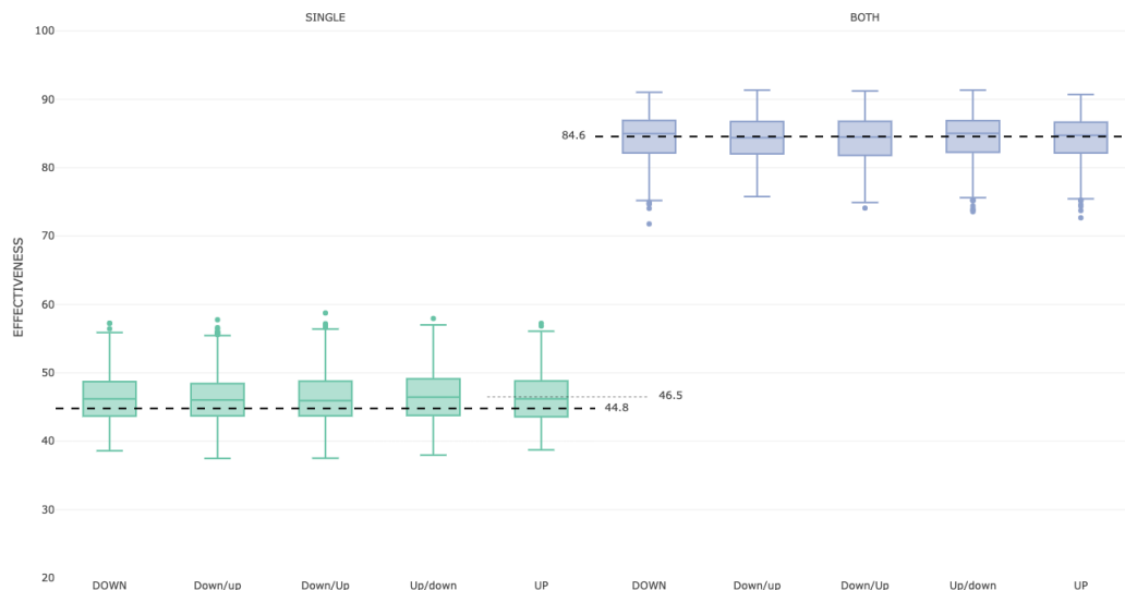
Figure 17: Robustness of effectiveness predictions against Delta for the Comirnaty vaccine. Crick study population versus Shifted Age-Weighted "true" distributions per dose. Box plots show effectiveness values evaluated for the Delta variant at a model fitting all effectiveness observations to the simulated true titres. The thick dashed lines show predictions from the unweighted Crick neutralisation data fitted to the effectiveness observations without Delta. The thin dashed line shows prediction using age-weighted Crick data. (After both doses, weighted and unweighted predictions were almost equal.)
