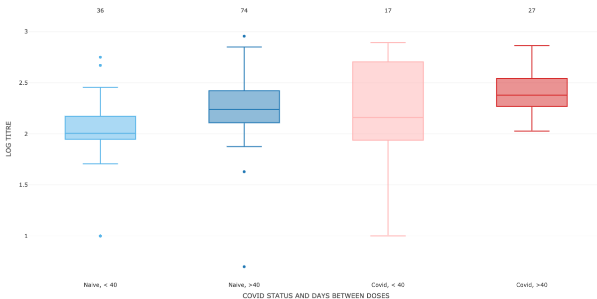
Figure 10: Two-dose Comirnaty cohort participants were grouped by Prior Covid-19 symptoms and Shorter versus Longer dosing interval. The log 10 titres are shown for the Delta variant. The group sizes are indicated. The mean ages per group, from left to right, were 43.4, 42.7, 43.2 and 43.7.
