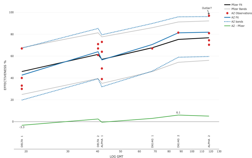
(a) Vaxzevria model fitted with a potential outlier, which is the two-dose effectiveness against Alpha from Pouwels et al. (2021).
