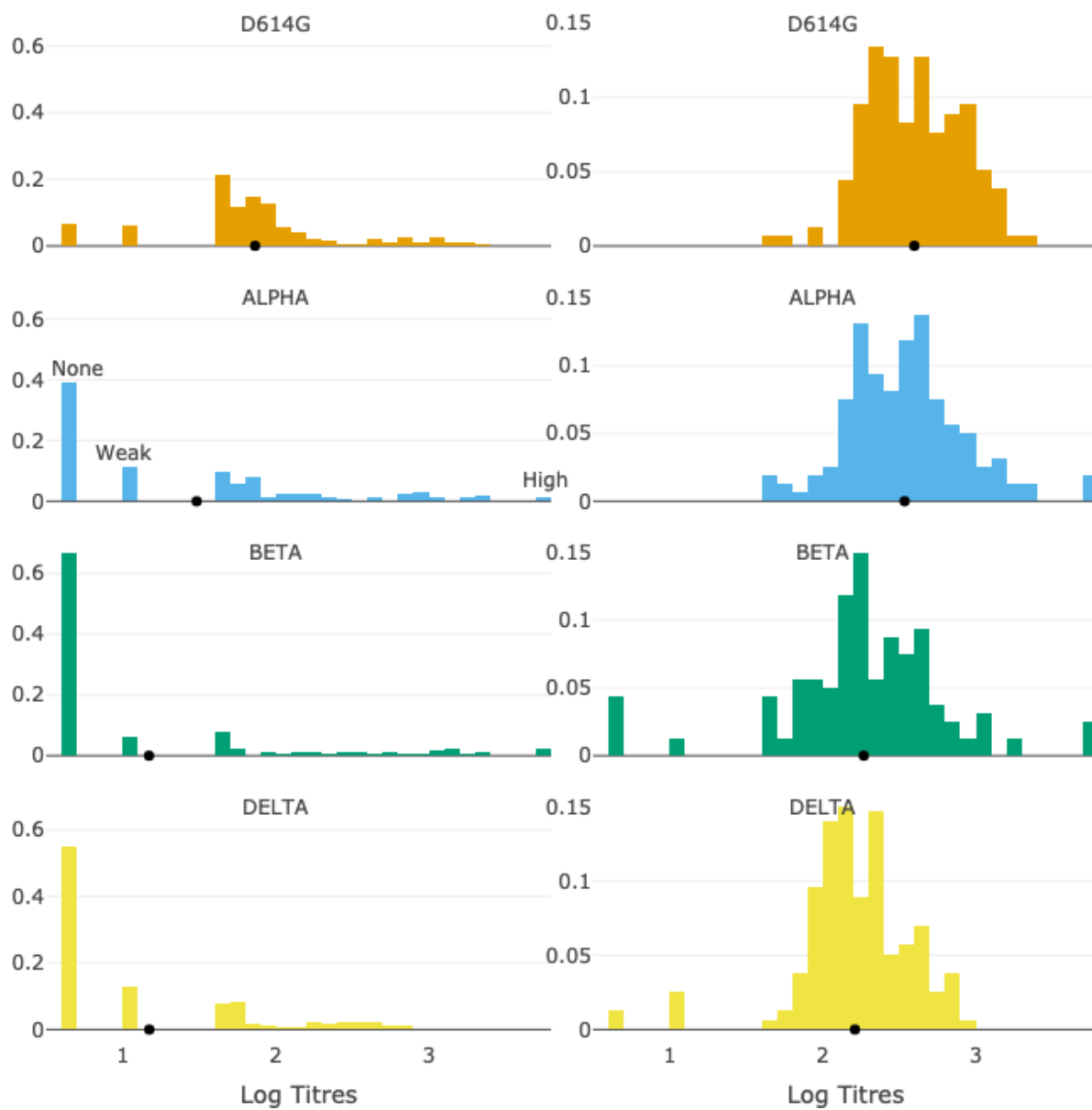
Figure 7: Distributions of log 10 titres after one (Left) and two (Right) Comirnaty doses. Detection thresholds are illustrated for Alpha after one dose: "None", recorded as 5, means no signal; "Weak", recorded as 10, means a signal below 40; "High", at 5120, means a signal above 2560. Sources: Wall et al. (2021b).
