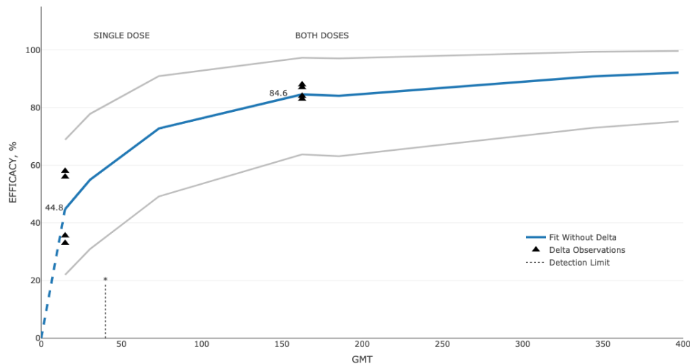
Figure 3: Predicted effectiveness of Comirnaty against the Delta variant. The model was fitted using the effectiveness and neutralisation data on all the variants except the indicated variant. Prediction was evaluated at the neutralisation titres of the variant.
