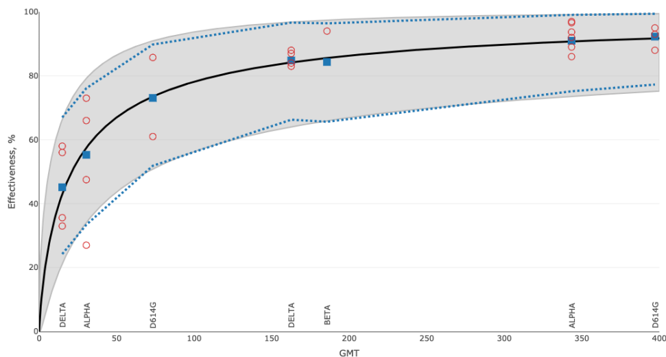
Figure 9: Simplified versus standard model fits for Comirnaty. Simplified fit and prediction bands are shown in a black line and grey shading. The standard model fit and prediction bands are shown in blue squares and dashed lines.
