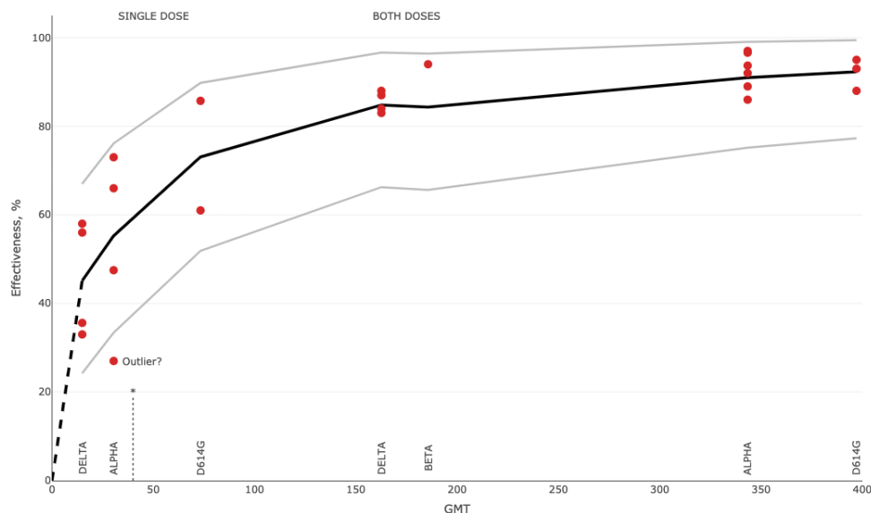
Figure 1: Model fitting observed symptomatic effectiveness of Comirnaty. Each group of observations corresponds to the variant indicated and is plotted against the geometric mean titre from the corresponding Crick sample. The 95% prediction bands are shown. The dotted line indicates the lower quantification threshold at GMT = 40 . The dashed line extends the model fit beyond the data range towards zero.
