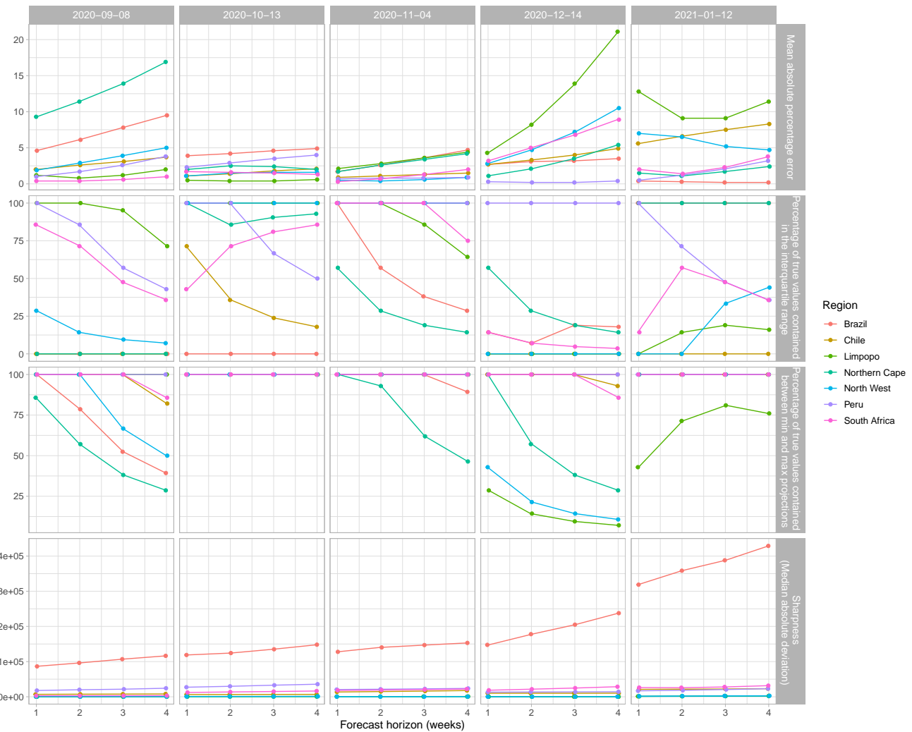
Figure 4. Model performance at each calibration time point.
