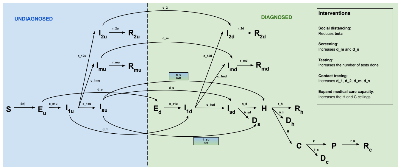
Figure 1. Schematic diagram of the disease transmission model. The capital letters represent different health states and the arrows represent transitions between the states. The letters above the arrows represents the rates of the transitions.
