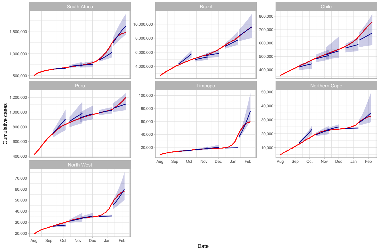
Figure 2. Cumulative COVID-19 confirmed cases together with forecasts and prediction intervals for different regions and origins (five time points) from September 2020 to January 2021. The red lines indicate the observed data and the blue lines indicate the projected mean cumulative cases. The shaded area indicates the minimum and maximum range.
