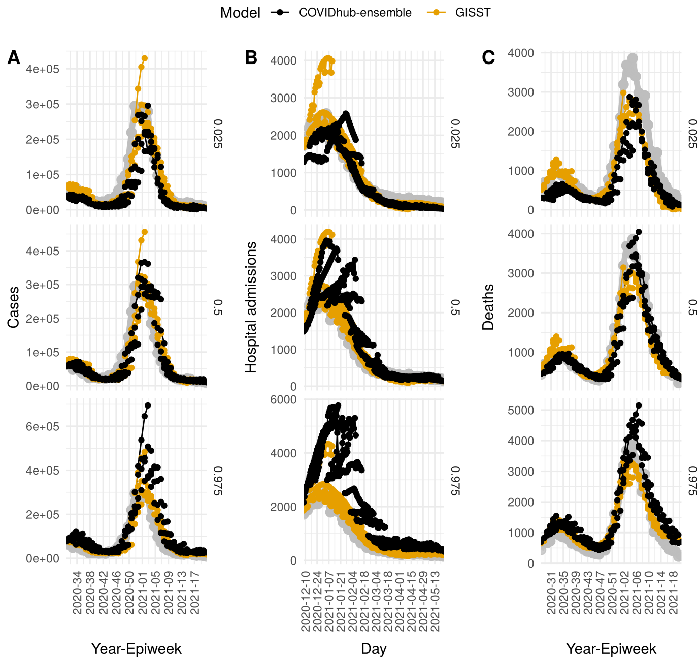
Fig 9. Forecast trajectories and target time series for cases (A), hospital admissions (B), and deaths (C). The panel labels at right are quantiles of the forecast. The target time series is plotted in grey. The performance penalty for underpredicting the true values is proportional to the quantile value, and the performance penalty for overprediction is proportional to 1 less the quantile value. Lines are drawn between forecasts of different horizons from a single forecast date.
