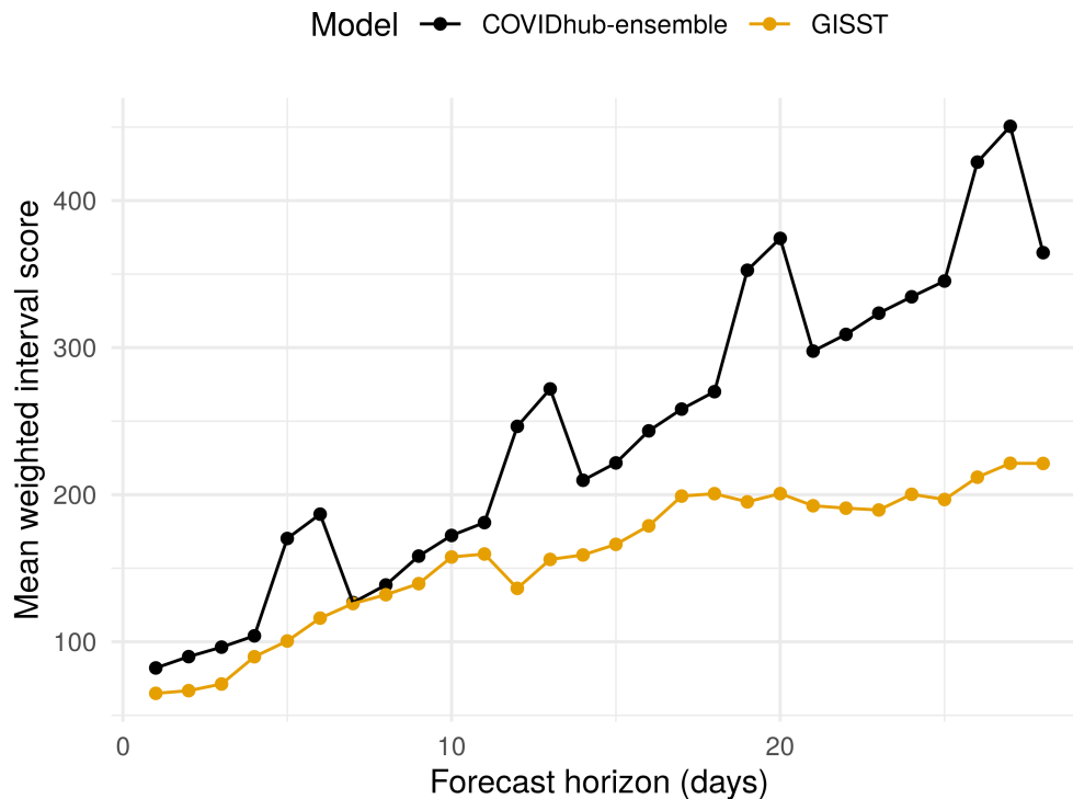
Fig 10. Overall performance of short-term forecasts of hospital admissions. Lower scores indicate better performance. The GISST forecasts score better than the COVIDhub Ensemble forecasts at all horizons. However, the difference in scores is slight at the 7 and 8 day horizons.
