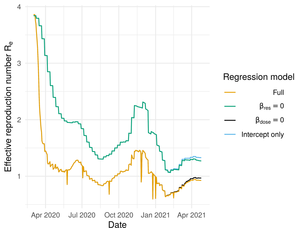
Fig 7. Effective reproduction number of fitted model for California. The model is fitted to data available on April 26, 2021. The full model corresponds to plugging \beta_t from equation 4 into \mathcal{R}_e = (\beta_t/\gamma)(X(t)/N) . We also plot \mathcal{R}_e with a \beta calculated by setting the effects of one or both of the covariates from their estimated values to zero to show their effects.
