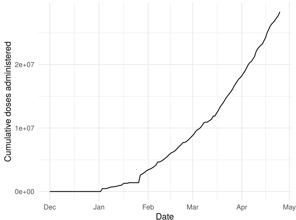
Fig 4. COVID-19 vaccination doses administered in California over time. This time series was used to estimate the effect of vaccination on reducing average susceptibility.
