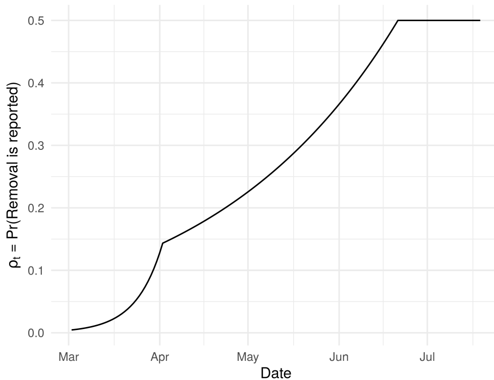
Fig 6. Estimate of the case reporting parameter \rho_t in California. This parameter is assumed to stay at 0.5 for dates beyond the last date plotted. See Tables 1 and 2 for the precise role of this parameter in our model.
