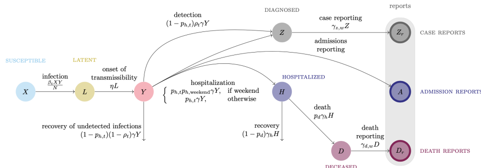
Fig 5. Flow diagram of differential equations for expected values of state variables
