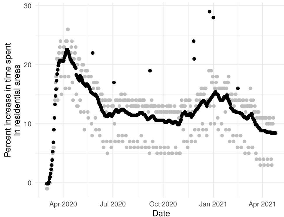
Fig 3. Indicators of the time spent at home. Grey points are the original data provided by Google of the amount of time people in California spent in residential areas relative to a pre-COVID-19 period. Black points are an example time series of the derived version which we use as a predictor of exposure in our model. Holiday effects in the original data are retained but weekly periodicity is removed. Consequently, the black and grey points coincide on the eight holidays considered in this time window. In other words, the value of this indicator on holidays is visible as the height of the black points separated from the main series of black points.
