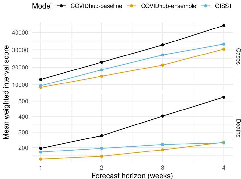
Fig 8. Overall performance of short-term forecasts of cases and deaths. Lower scores indicate better performance. The GISST forecast consistently outperforms the COVID-19 Forecast Hub Baseline forecast and performs relatively best for 4-week ahead death forecasts.
