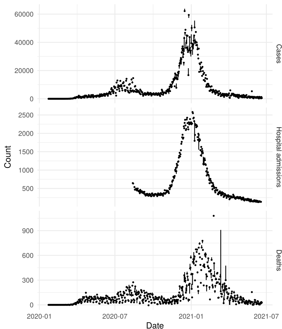
Fig 2. Time series of forecasting targets and range of revisions. Points are the California time series of COVID-19 indicators which our model is designed to forecast in the version of the data used to fit our model, which was the version available on June 21, 2021. The vertical line range gives the range of values that each observation had in all versions of the data used to fit our model, which were the versions of the data available on Mondays from June 29, 2020 to April 26, 2021.
