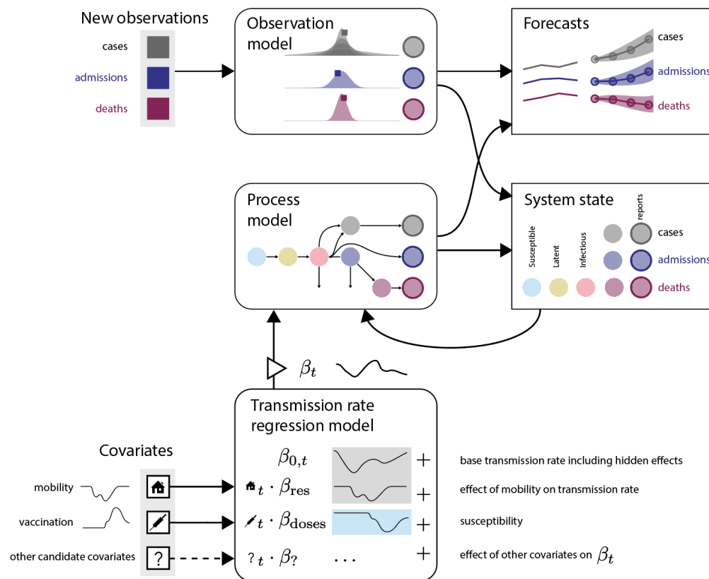
Fig 1. Graphical summary of the GISST concept for our modeling and forecasting infectious diseases. The main features are time-dependent parameters to accommodate the non-stationarity of COVID-19 dynamics, a regression model to incorporate data on covariates of transmission, and the integration of a compartmental epidemiological process model into a Gaussian state-space model for cases, hospital admissions, and deaths.
