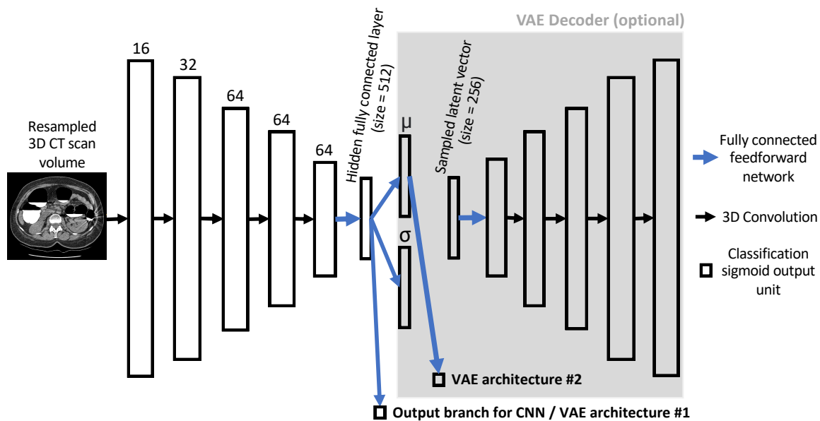
Figure 1. The architectures employed. The CNN architecture consists of five CNN layers followed by two fully connected layers. Optionally a VAE decoder may be attached to the CNN to encourage the CNN to obtain good high level features. If the VAE is attached, one can experiment with attaching the classification output to the vector of latent means (architecture 2)
