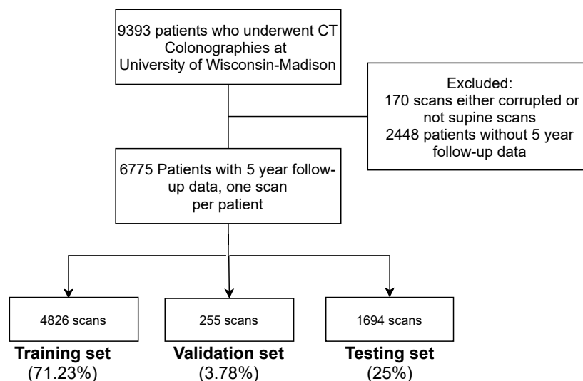
Figure 2. Patient flow chart showing how the patient cohort was selected and split into train, validation, and test sets for five year survival prediction.
