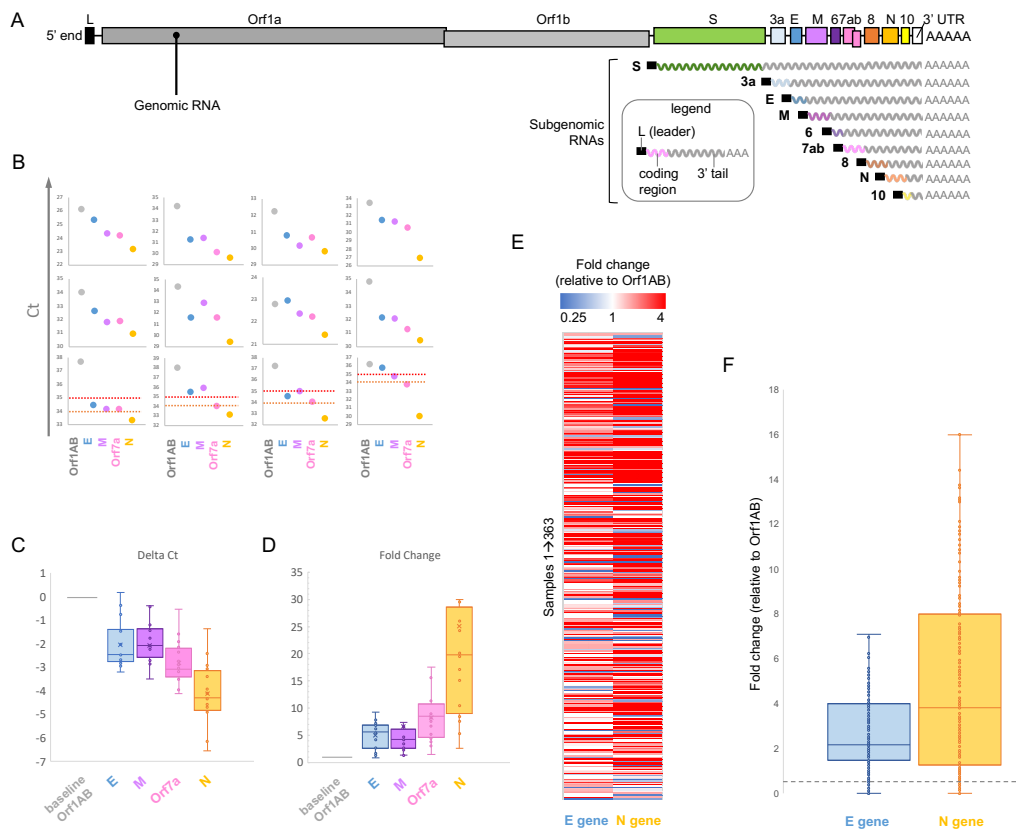
102 Figure 1 legend. A. SARS-CoV-2 genome and transcriptome organization. The transcripts expressed 103 as subgenomic mRNAs are indicated. Note the enrichment in viral RNA as genes are positioned closer 104 to the 3' end. Also note the position of the main target genes used in qRT-PCR diagnostics (orf1ab, E, 105 M and N) relative to the 3' end of the viral genome. B. Ct values of orf1ab, E, M, orf7a and N genes 106 in clinical samples previously validates as positive. Ct cutoffs of 34 and 35 are indicated in the 4 lower 107 individual panels by orange and red lines, respectively. C. Box plots showing Delta Ct values of E, 108 M, orf7a and N genes relative to the orf1ab. D. Box plots showing fold change in gene expression of 109 E, M, orf7a and N genes relative to the orf1ab. E. Heat map showing fold change in E and N gene 110 expression relative to orf1ab in 363 positive clinical samples. F. Box plot showing fold change in E 111 and N gene expression relative to orf1ab in samples used for the retrospective analysis. The gray 112 discontinuous line indicates the orf1ab baseline. Note the gradual increase in gene expression for E 113 and N genes.
