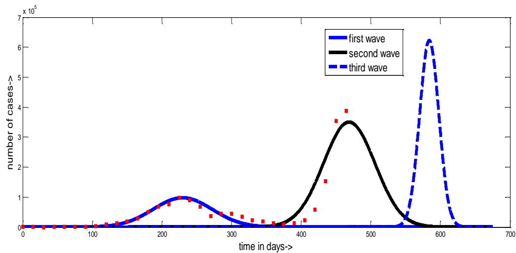
Fig. 3 Predicted and Actual COVID-19 Waves of India
