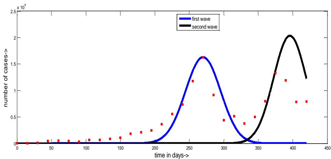
Fig. 1 Predicted and Actual COVID-19 Waves of Ukraine
