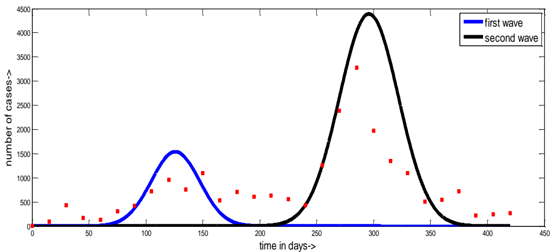
Fig. 2 Predicted and Actual COVID-19 Waves of Panama
