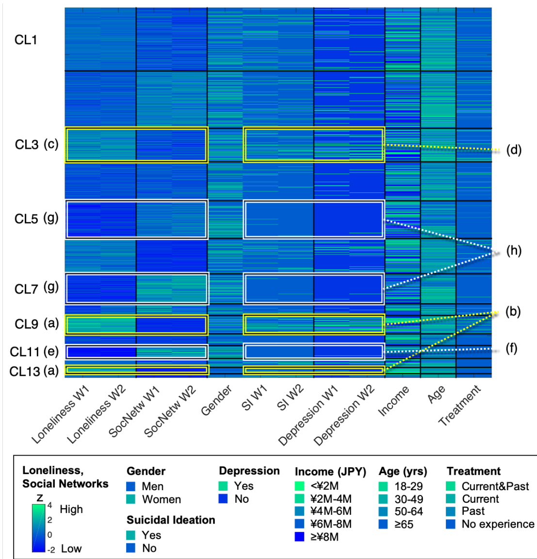
Figure 4. Visualization of an exhaustive interaction structure of factors associated with depression.
