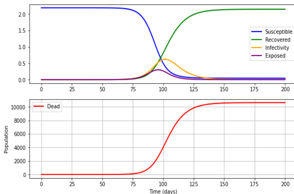
Figure 2. Predictions based on the SEIRD model R_0 = 4 without any preventive strategies
