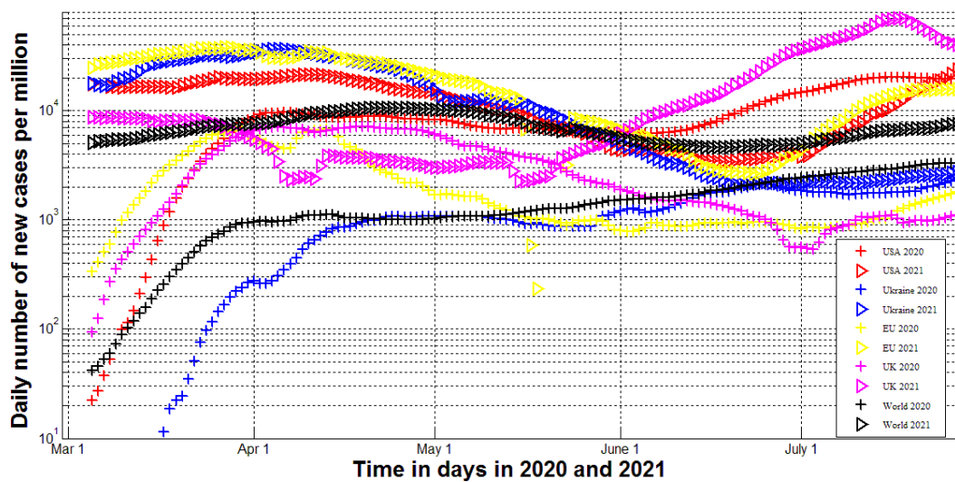
Fig. 1. Averaged daily number of new cases for northern region in March-July, 2020 and 2021. “Crosses” correspond to the DCC values calculated for 2020 with the use of eqs. (1), (2) and Table 1. “Triangles” correspond to the DCC values calculated for 2021 with the use of eqs. (1), (2) and Table 2.
