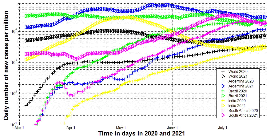
Fig. 2. Averaged daily number of new cases for southern region in March-July, 2020 and 2021. “Crosses” correspond to the DCC values calculated for 2020 with the use of eqs. (1), (2) and Table 1. “Triangles” correspond to the DCC values calculated for 2021 with the use of eqs. (1), (2) and Table 2.
