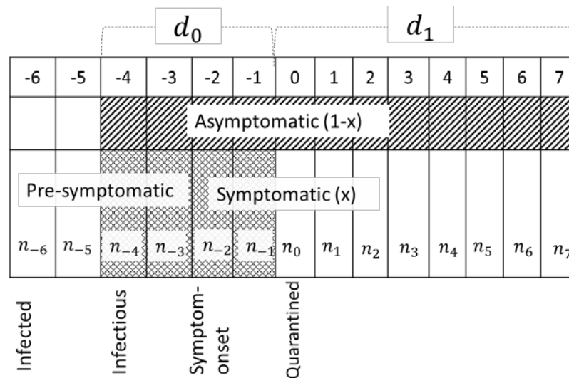
Fig.1. Break down of COVID-19 patients into asymptomatic, pre-symptomatic and symptomatic patients. Patients in the shaded area are infectious. The hatched region represents infectious asymptomatic patients who produce untraceable patients and the cross-hatched region corresponds to infectious pre-symptomatic and symptomatic patients who produce traceable patients.
