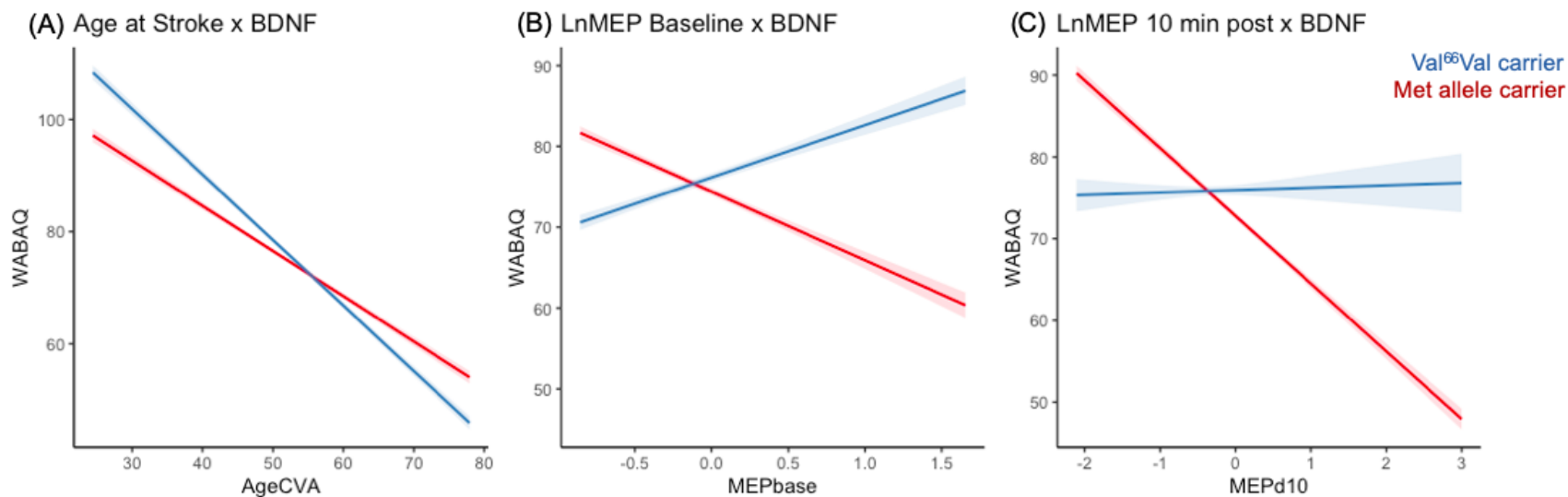
Figure 3. BDNF Interactions Predict WAB-AQ.
