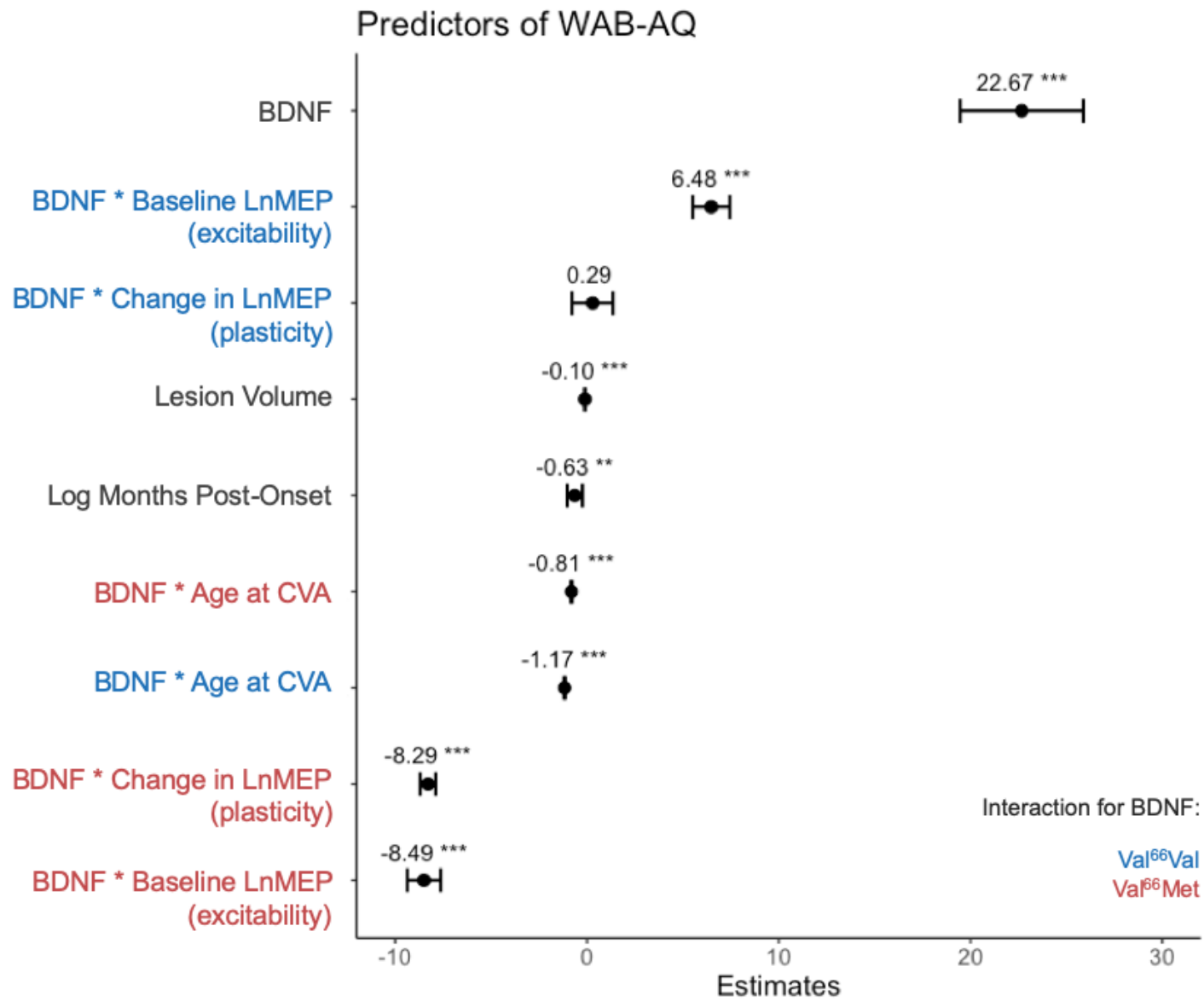
Figure 2. Estimates (Fixed Effects) of Regression Model.
