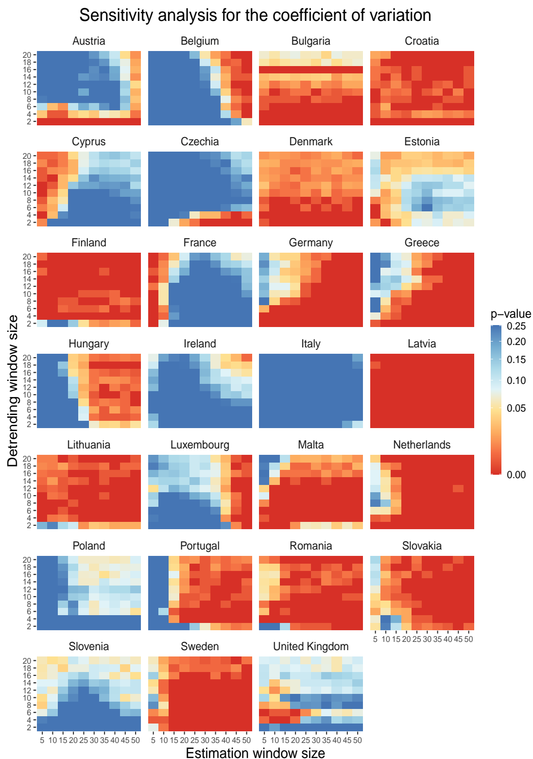
Figure 15: Shows bootstrapped p -values indicating whether the observed Kendall's \tau in the coefficient of variation is significantly larger than expected under the null across rolling window sizes. Note that p = 0.25 in the legend means p \geq 0.25 .
