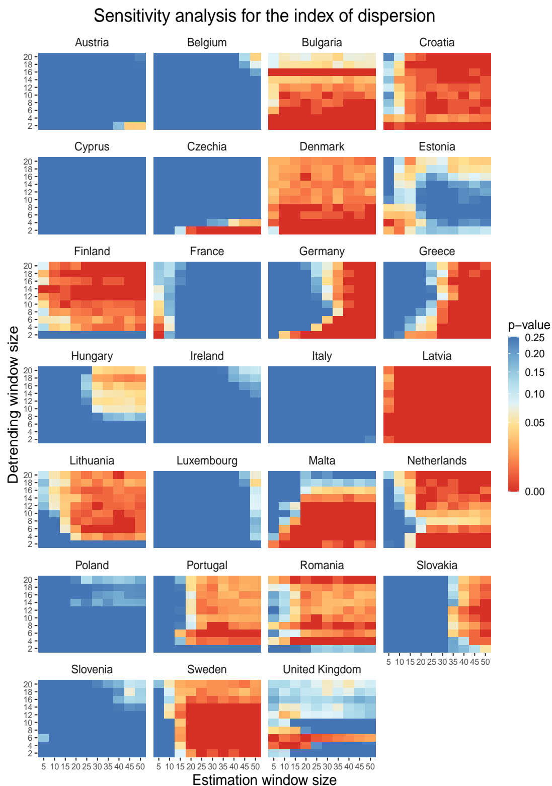
Figure 16: Shows bootstrapped p -values indicating whether the observed Kendall's \tau in the index of dispersion is significantly value than expected under the null across rolling window sizes. Note that p = 0.25 in the legend means p \geq 0.25 .
