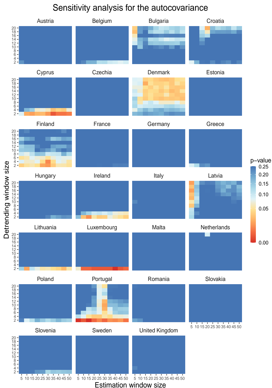
Figure 17: Shows bootstrapped p -values indicating whether the observed Kendall's \tau in the autocovariance is significantly larger than expected under the null across rolling window sizes. Note that p = 0.25 in the legend means p \geq 0.25 .
