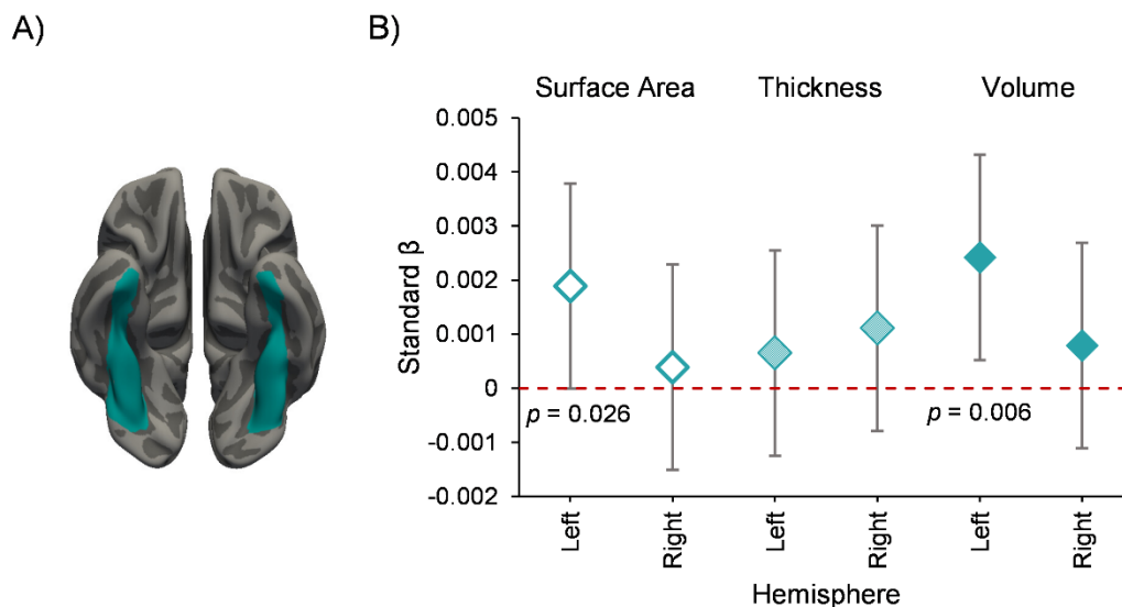
699 Figure 2. Effects of schizophrenia polygenic resilience scores ( PRS_{Resilience} ) on fusiform gyrus 700 (FFG) anatomical metrics in the UK Biobank sample. A) Shows Desikan-Killiany (33) 701 FFG parcels, B) depicts PRS_{Resilience} effects for anatomical metrics, which were significant 702 for cortical volume and surface area in the left FFG. Error bars indicate 95% confidence 703 intervals.
