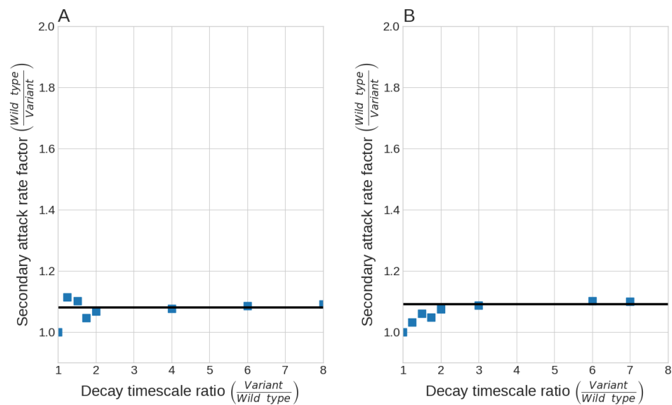
Figure 2. The effect of genetic variant with higher environment stability on the hSAR. (A) Factor 1 - The decay rates on surfaces ( \alpha_{furniture} , \alpha_{fomite} , and \alpha_{hand} ) on the hSAR ; (B) Factor 2 - The decay rate in the air ( \alpha_{air} )
