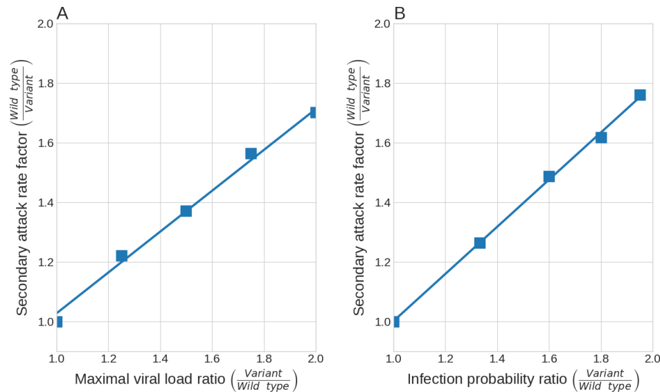
Figure 3. (A) The effect of the maximal viral load on the SAR. (B) The effect of infection probability on the SAR.
