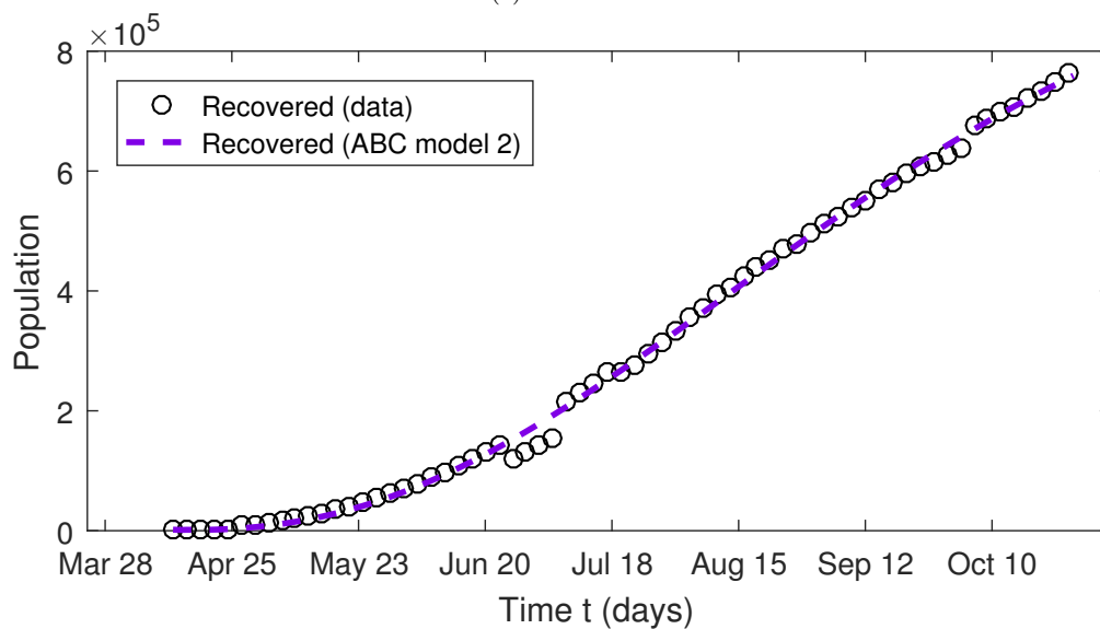
(b) Recovered cases.
