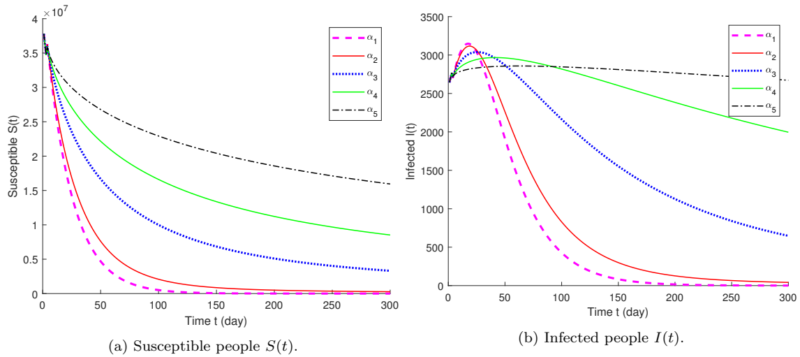
Figure 5: The representation of the numerical solution of the fractional model obtained for S(t) and I(t) for five arbitrary values of fractional multi-order. These results are obtained using the parameters presented in Table 3 except \Lambda and \delta are chosen to be zero. We have chosen \alpha_1 = (1, 1, 1, 1) , \alpha_2 = (0.95, 0.95, 0.95, 0.95) , \alpha_3 = (0.8, 0.8, 0.8, 0.8) , \alpha_4 = (0.7, 0.65, 0.6, 0.5) and \alpha_5 = (0.4, 0.2, 0.3, 0.1) .
