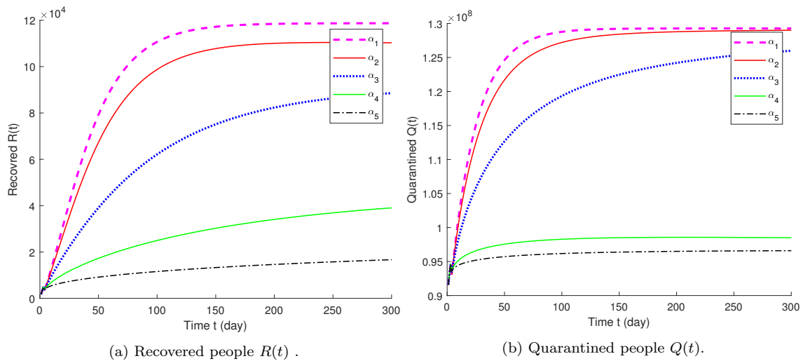
Figure 6: The representation of the numerical solution of the incommensurate fractional model obtained for R(t) and Q(t) for five arbitrary values of fractional multi-order. These results are obtained using the parameters presented in Table 3 except \Lambda and \delta are chosen to be zero. We have chosen \alpha_1 = (1, 1, 1, 1) , \alpha_2 = (0.95, 0.95, 0.95, 0.95) , \alpha_3 = (0.8, 0.8, 0.8, 0.8) , \alpha_4 = (0.7, 0.65, 0.6, 0.5) and \alpha_5 = (0.6, 0.5, 0.45, 0.4) .
