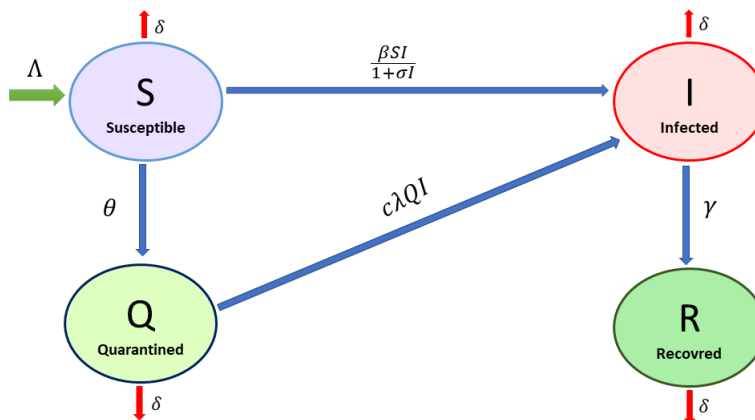
Figure 1: Schematic diagram of 2019-nCoV model and parameters.
