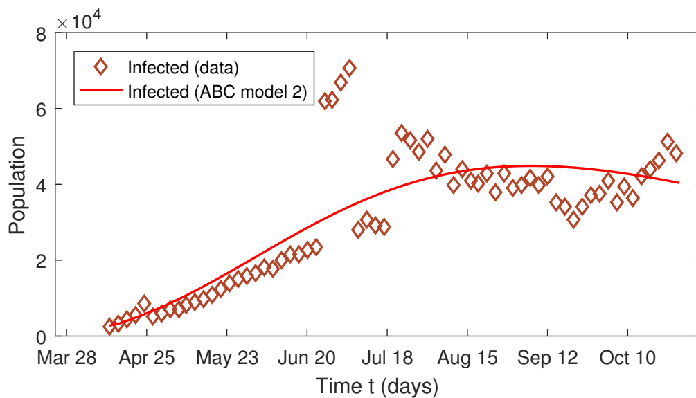
(a) Infected active cases.
