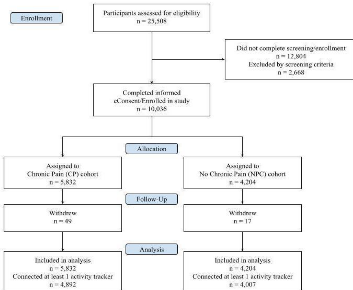
Figure 1. CONSORT diagram
