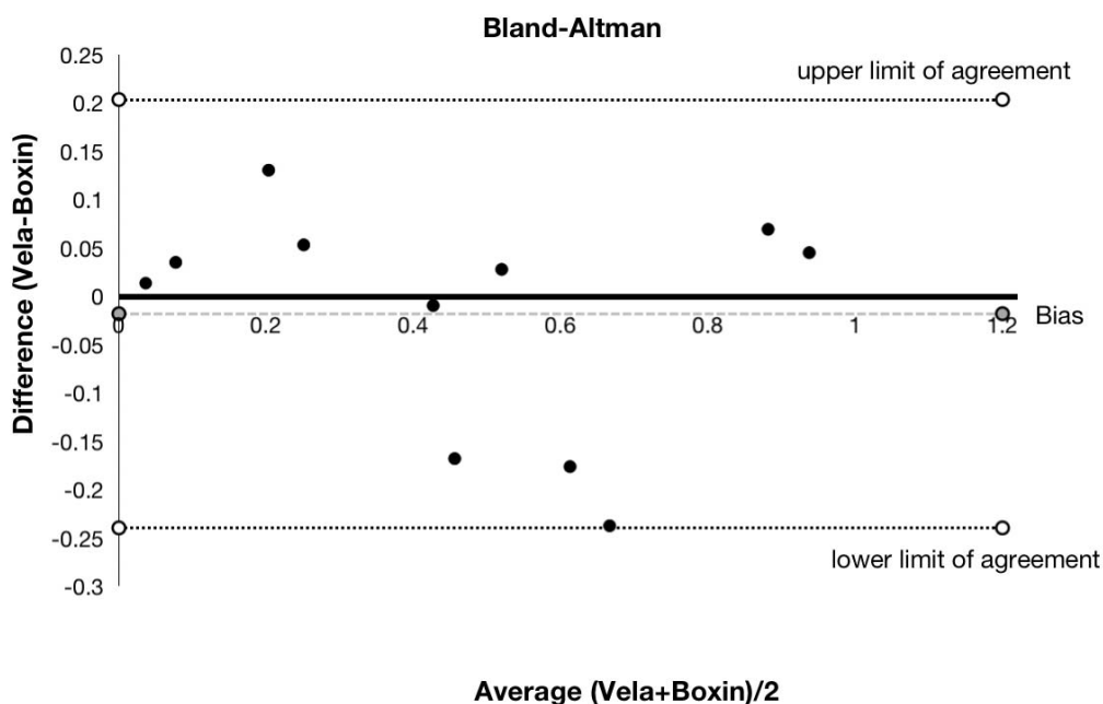
Figure 2. The Bland-Altman plot. Comparison of Boxin and Vela NGS methods in quantifying drug-resistance associated mutations. The y-axis represented the variant frequency difference detected by Boxin and Vela NGS. The x-axis represented the average variant frequency detected by Boxin and Vela NGS.
