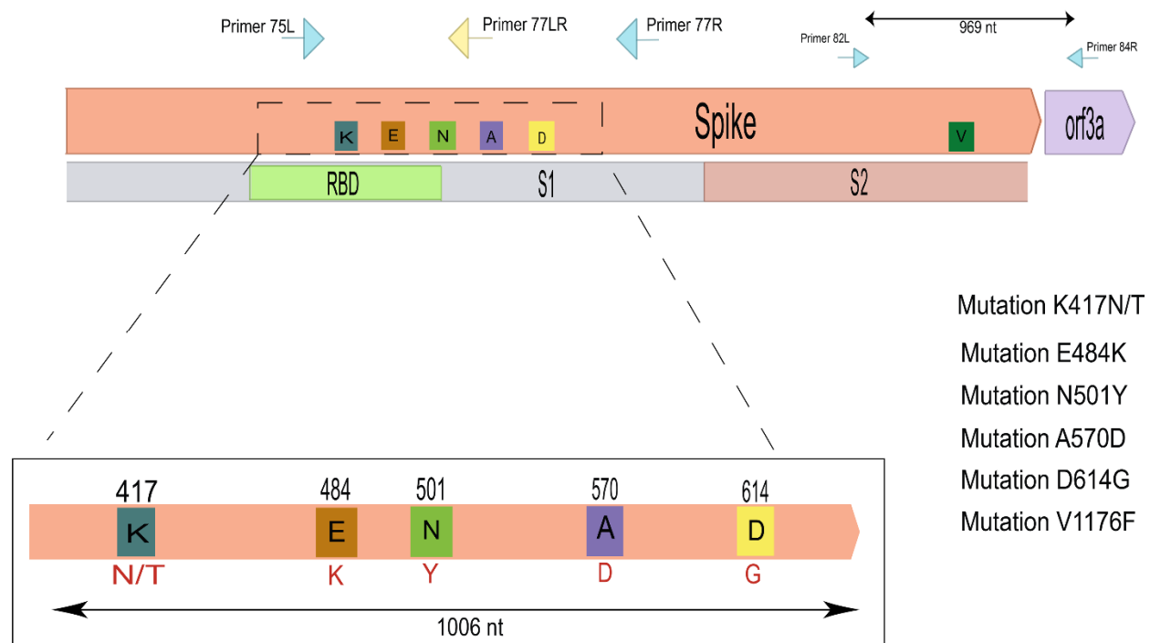
Figure 1 - Schematic representations of the Spike protein and the 1006 bp amplicon. PCR amplifications were performed with primers that were used both for PCR and Sanger sequencing (blue arrows). Yellow arrows indicate primers used only for sequencing. Colored rectangles represent changes in amino acids found in different VOI and VOC's and their respective positions in the SARS-CoV-2 genome, Lysine (K) blue, Glutamic acid (E) orange, Asparagine (N) green, Alanine (A) purple, Aspartic acid (D) yellow, Valine (V) dark green. It is also represented the 969 bp PCR amplicon generated with primers annealing within
