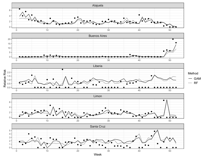
Figure 2: Model comparison over the prediction period [9]. Lines: predicted relative risk. Points: observed relative risk.
