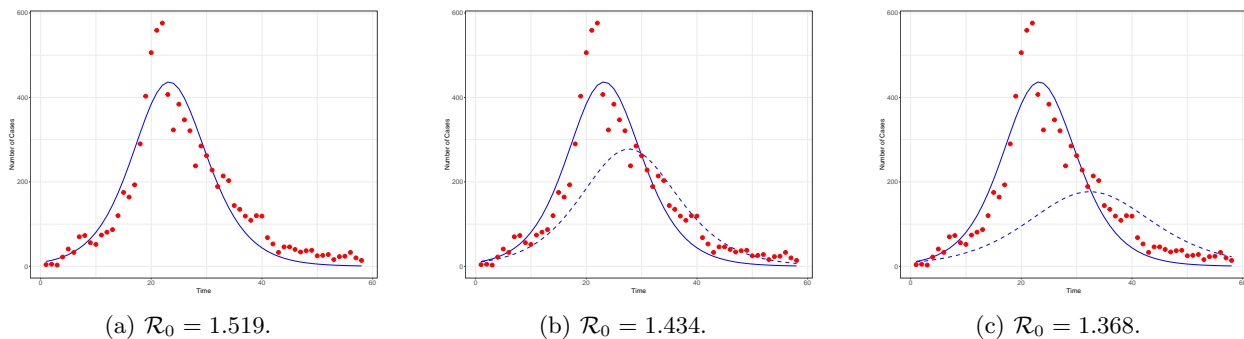
Figure 1: Number of reported Zika cases (red dots) from the 2016-2017 ZIKV outbreak in Costa Rica and model solutions. The solid blue line represents the best fit and the dotted line represents a lower percentage of individuals that stay indoors, therefore reducing the number of secondary infections [8].
