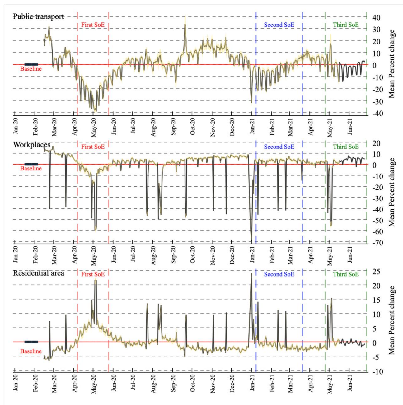
Figure 2. Descriptive changes in mobility: Public transport, workplaces, and residential area
