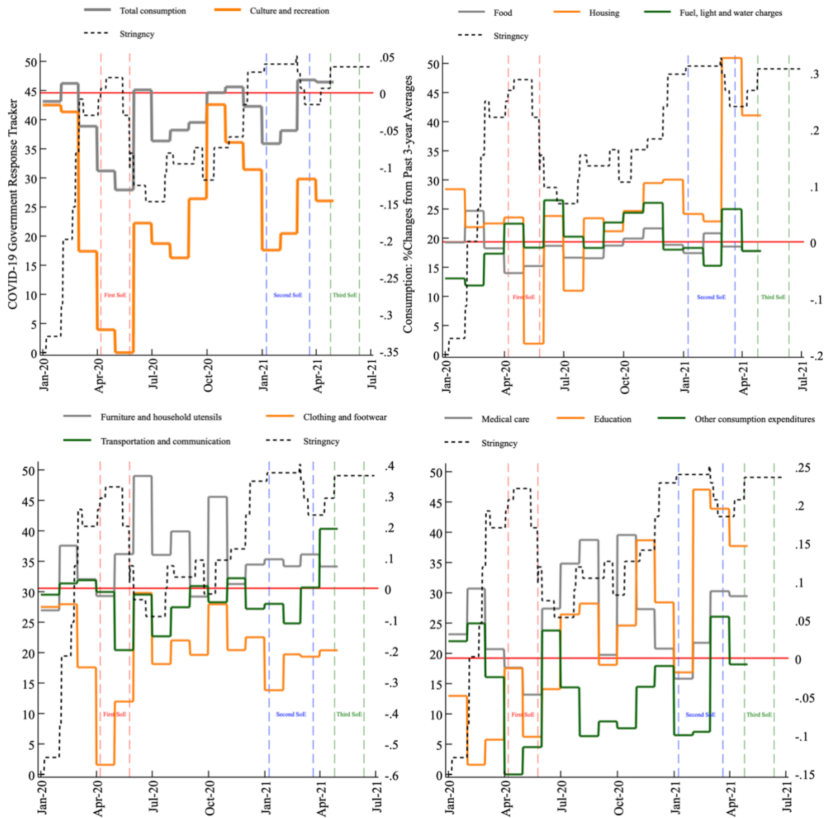
Figure 3. Stringency and consumption
