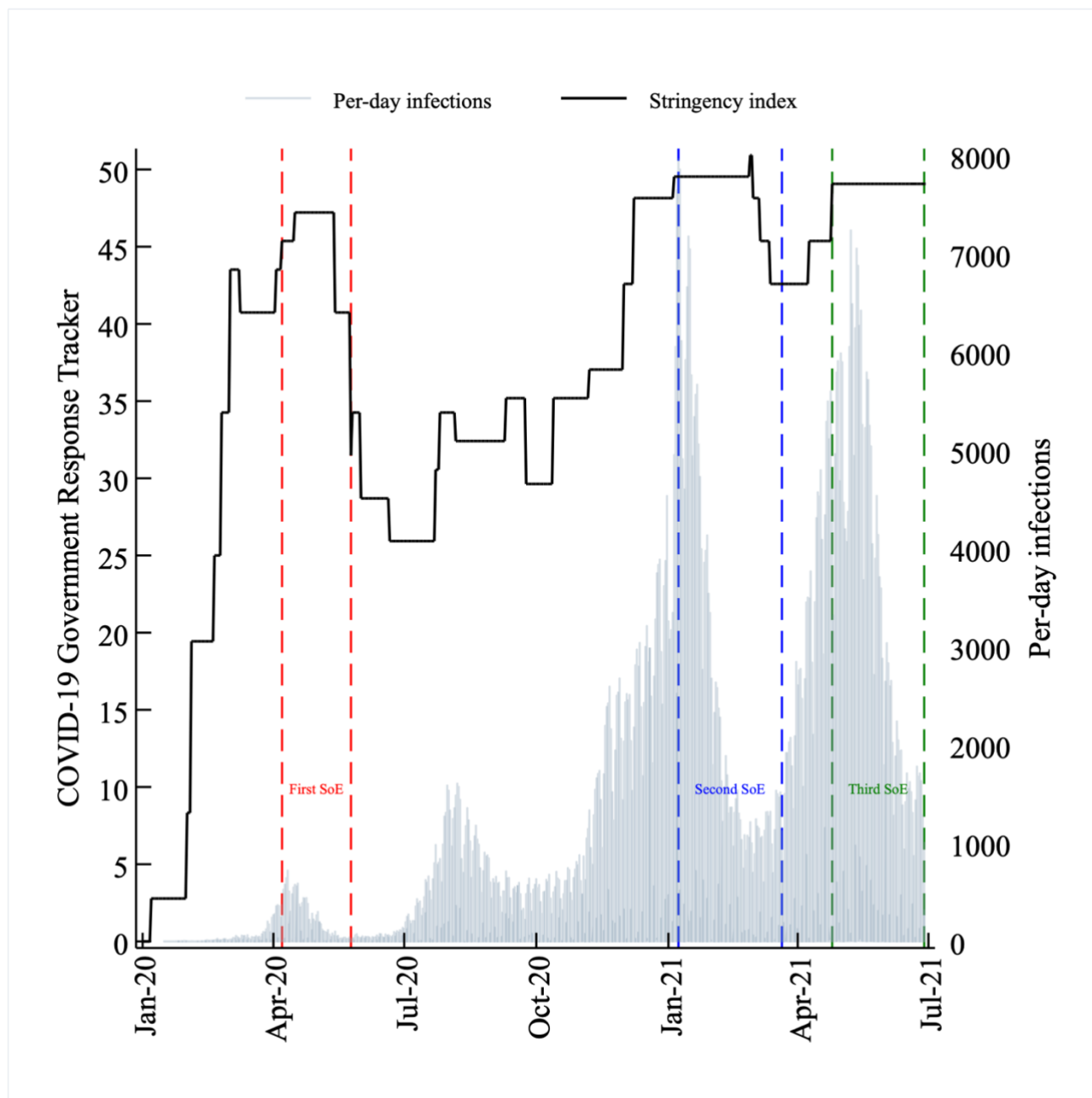
Appendix Figure 1. The number of confirmed COVID-19 infections, the state of emergency, and stringency index of the government responses to the pandemic
