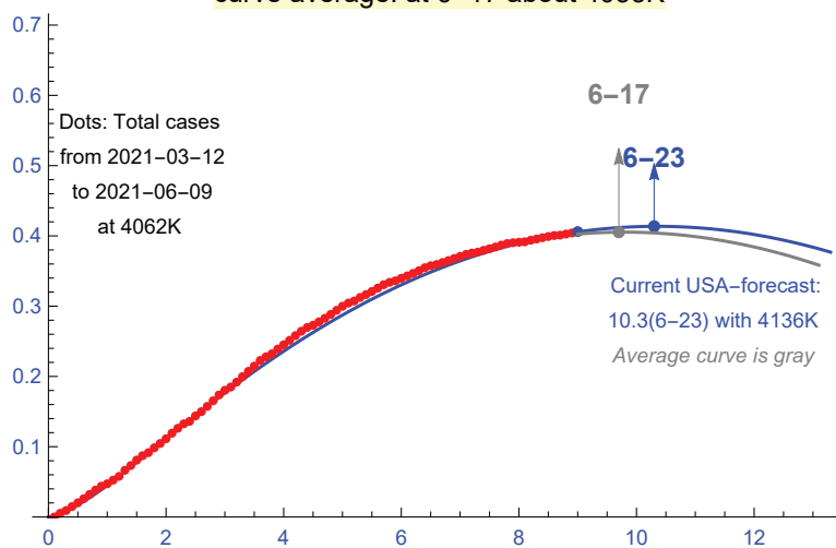
FIGURE 24. A sample forecast in the USA: 06/09/2021.
