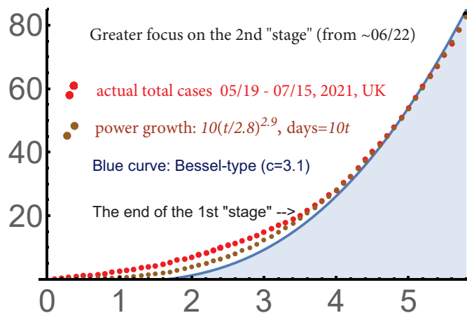
FIGURE 21. UK: 05/19-07/15, the power approximation.
