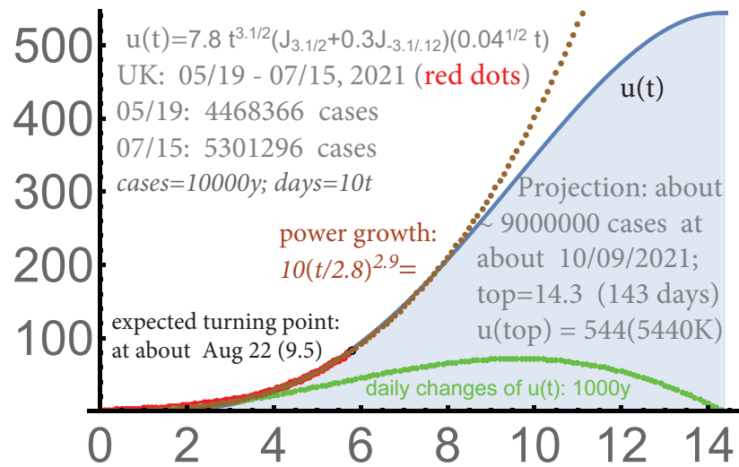
FIGURE 20. UK: 05/19-07/15, focus on the 2nd stage.
