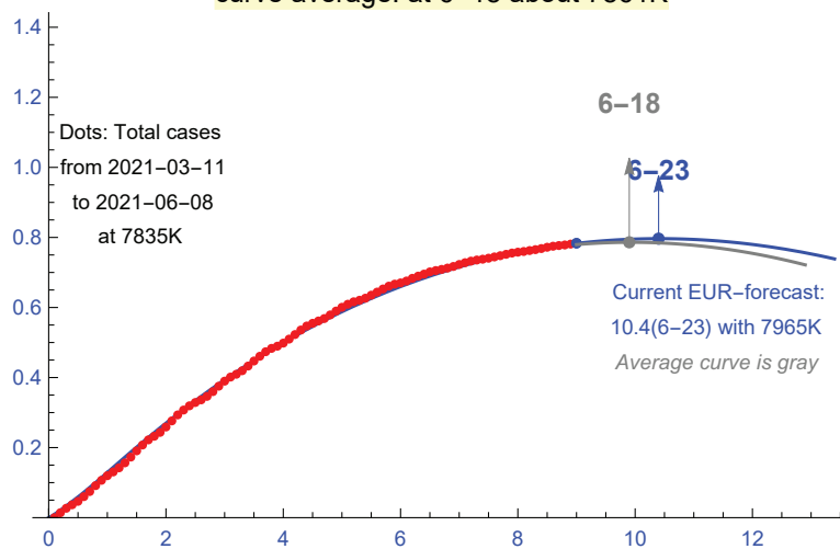
FIGURE 25. A sample forecast in Europe: 06/08/2021.
