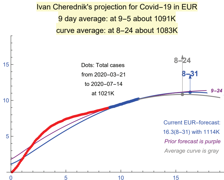
FIGURE 23. An auto-forecast for Europe as of 7/14 (2020)
