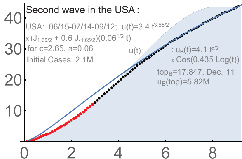
FIGURE 12. 2-phase solution for the 2nd wave in the USA.
