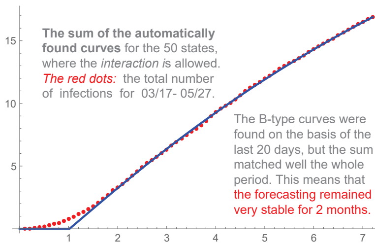
FIGURE 22. USA, the sum of the curves for individual states.
