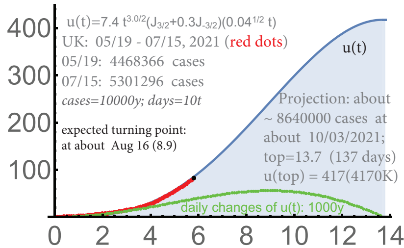
FIGURE 19. UK: 05/19-07/15, a possible upper bound.
