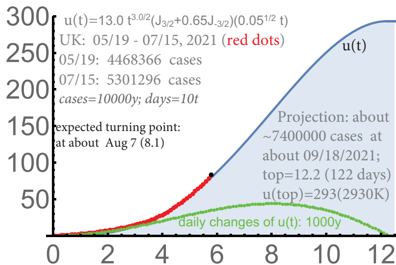
FIGURE 18. UK: 05/19-07/15, a possible lower bound.
