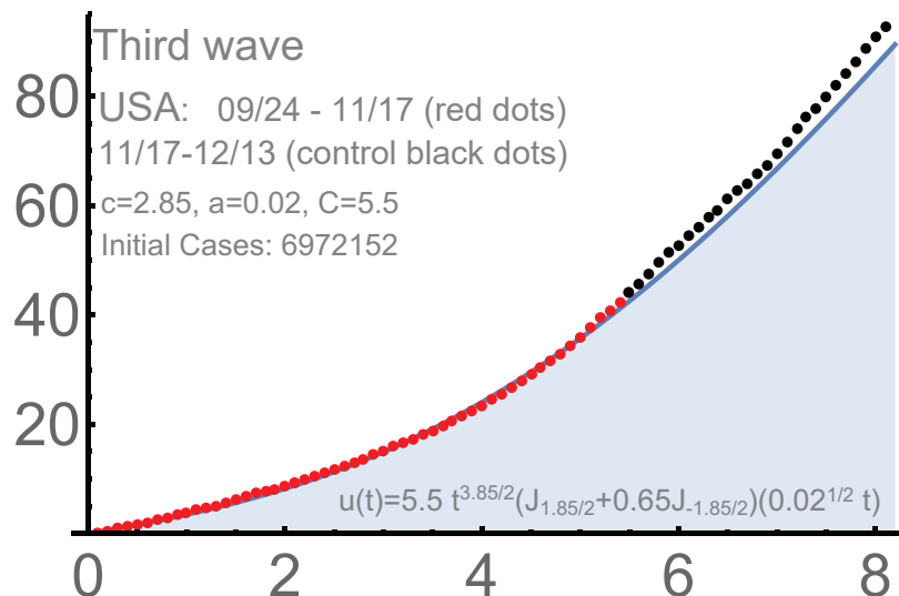
FIGURE 13. The 3rd wave in the USA.
