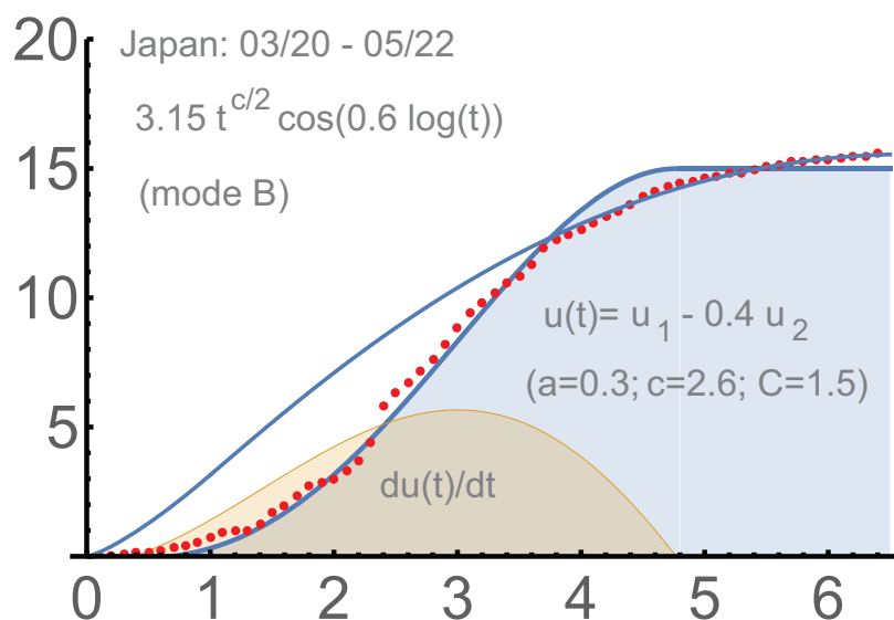
FIGURE 4. Japan: u = 1.5t^{1.8}(J_{0.8} - 0.4J_{-0.8})(t\sqrt{0.3}) .
