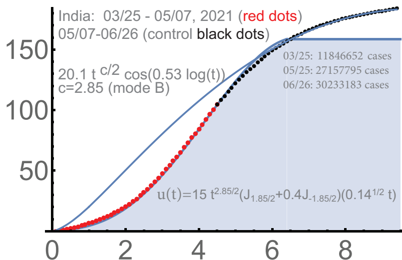
FIGURE 11. India: 2-phase solution until 06/26/2021
