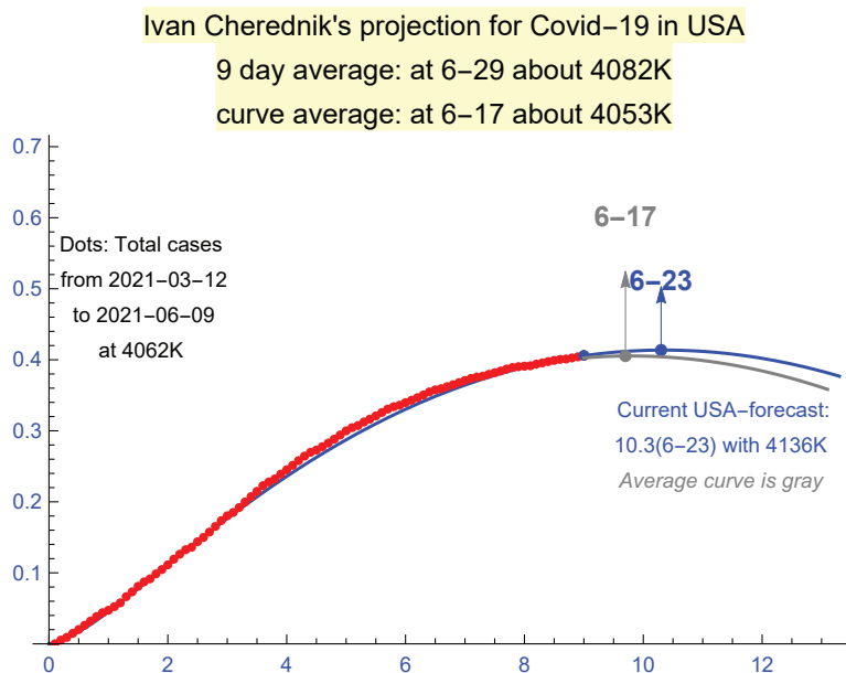
FIGURE 22. A sample forecast in the USA: 06/09/2021.
