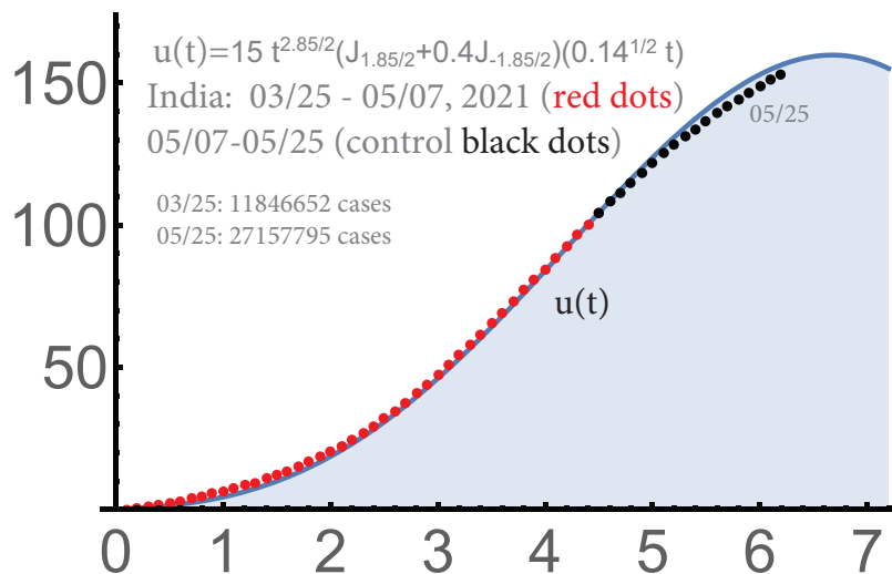
FIGURE 10. India: 2nd wave, c=2.85 , a=0.14 , C=15 .
