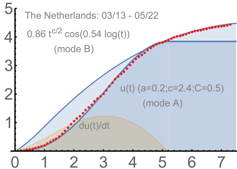
FIGURE 6. The Netherlands: u = 0.5t^{1.7}J_{0.7}(t\sqrt{0.2}) .
