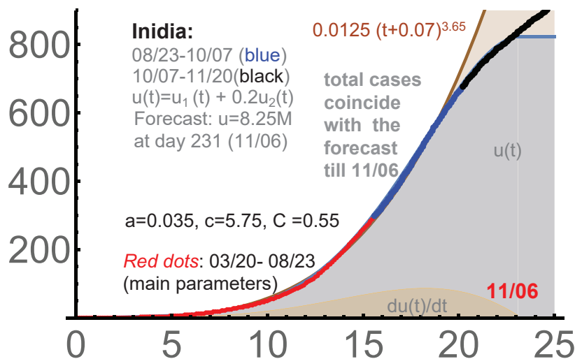
FIGURE 9. India: 3/20-10/7, c=5.75 , a=0.035 , C=0.55 .
