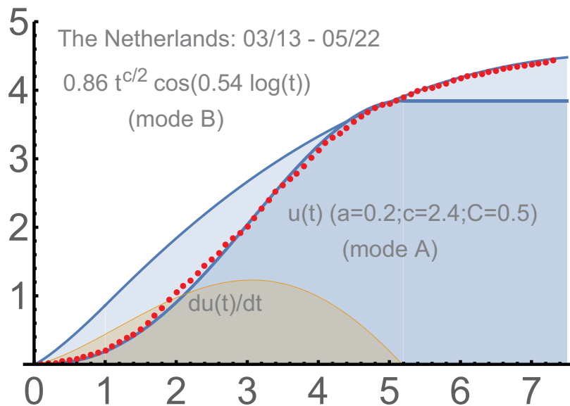
FIGURE 6. The Netherlands: u = 0.5t^{1.7} J_{0.7}(t\sqrt{0.2}) .
