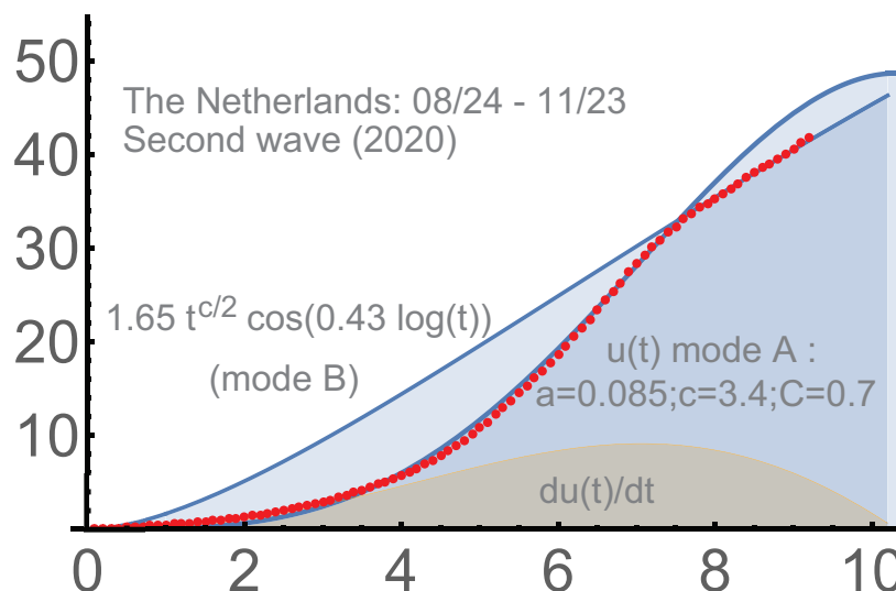
FIGURE 7. The 2nd wave in the Netherlands.
