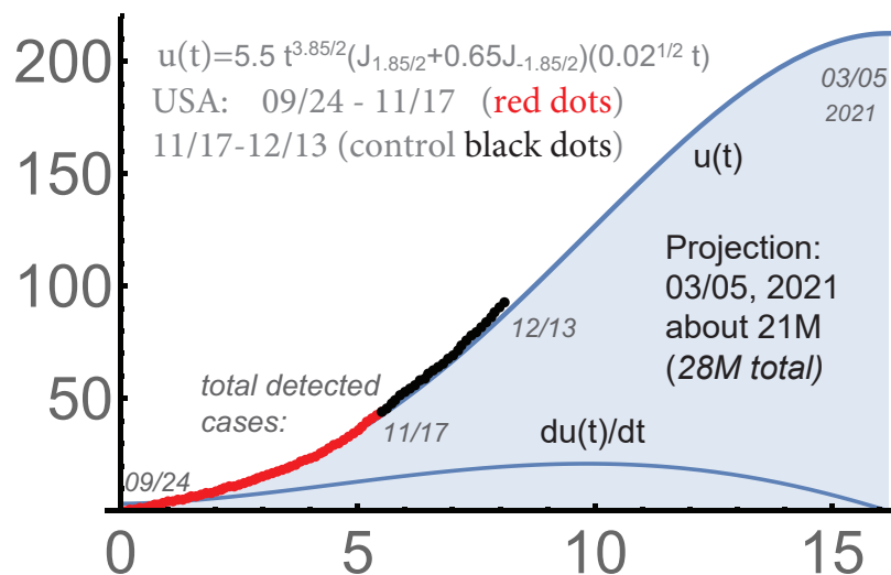
FIGURE 14. The 3rd wave in the USA.
