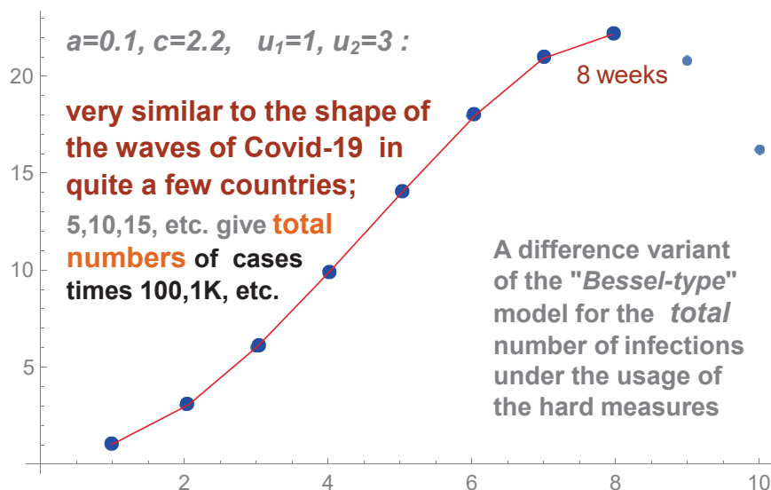
FIGURE 1. Discrete modeling the number of infections.
