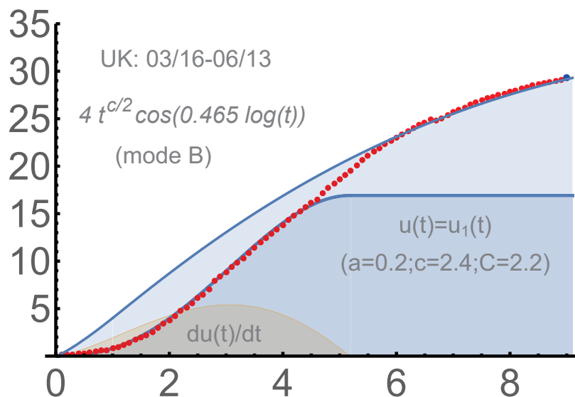
FIGURE 5. UK: u = 2.2t^{1.7} J_{0.7}(t\sqrt{0.2}) .
