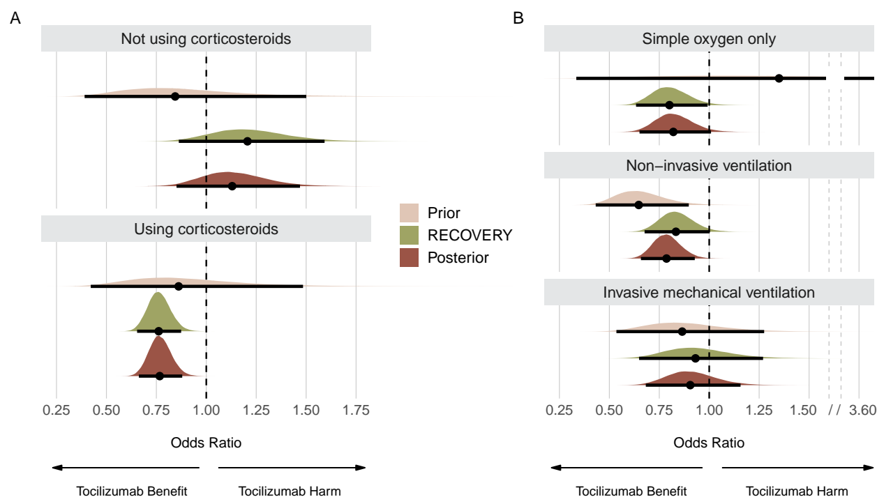
Figure 1. Prior, RECOVERY, and posterior distributions for each subgroup on the mortality outcome. Panel A shows results for subgroups regarding use of corticosteroids. Panel B shows results for subgroups regarding respiratory support. Point estimates depict the median and interval bars depict 95% highest density intervals. Using conjugate normal analyses, these distributions were originally combined in the log-odds ratio scale (Methods section). They were transformed into the odds ratio scale for this figure to aid visual interpretation.
