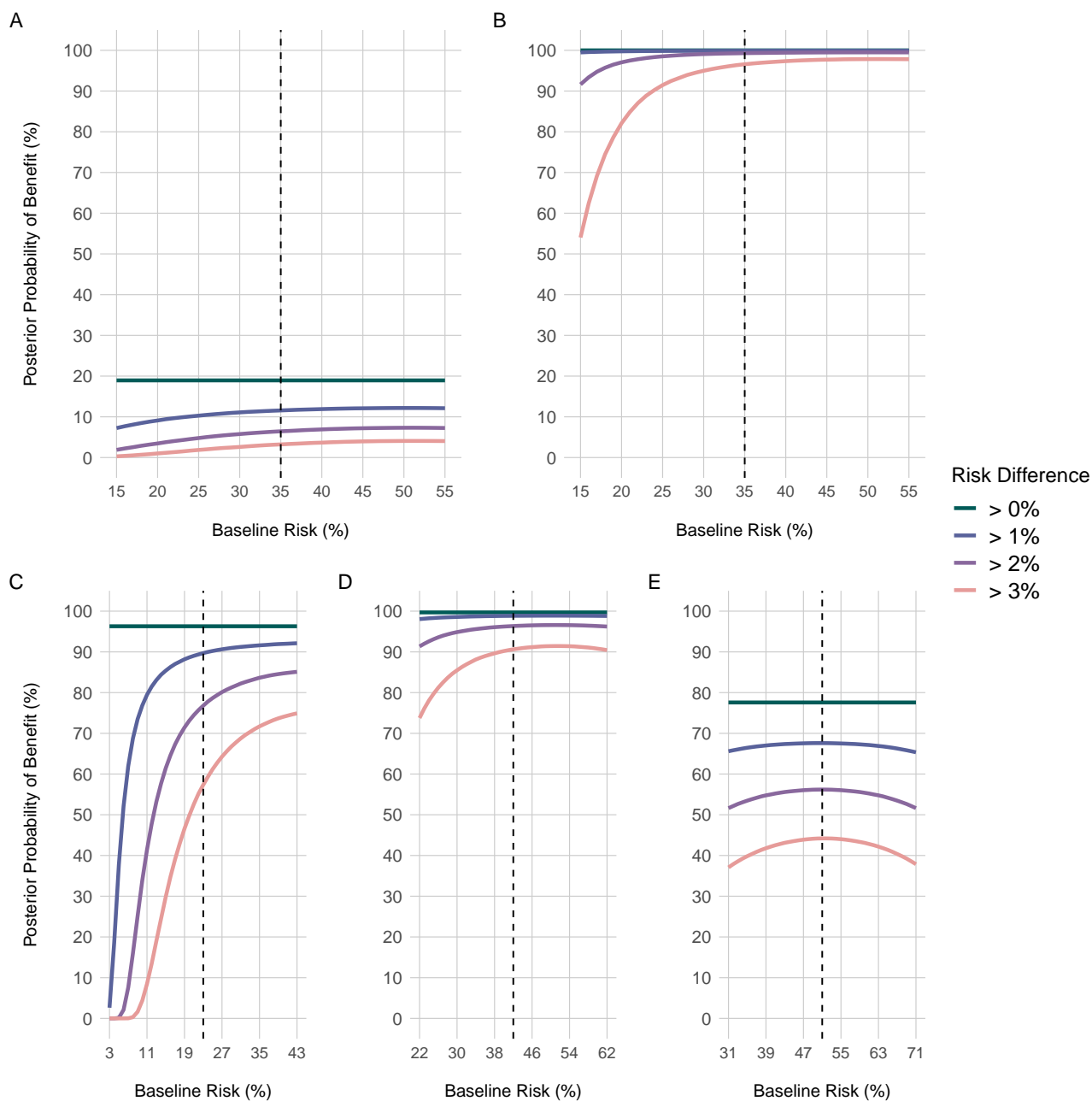
Figure 4. Posterior probabilities from sensitivity analyses using multiple different baseline risks on the mortality outcome. Panel A shows results for patients not using corticosteroids; Panel B shows results for patients using corticosteroids. Panel C shows results for simple oxygen only; Panel D shows results for non-invasive ventilation; Panel E shows results for invasive mechanical ventilation. Each line represents the posterior probability of benefit for a specific cutoff, such as risk difference lower to 0%, 1%, 2% and 3%. Vertical black dashed lines represent the respective baseline risk underlying other analyses (Figure 2), i.e., risk in the control group in the RECOVERY trial for each subgroup (Table 1).
