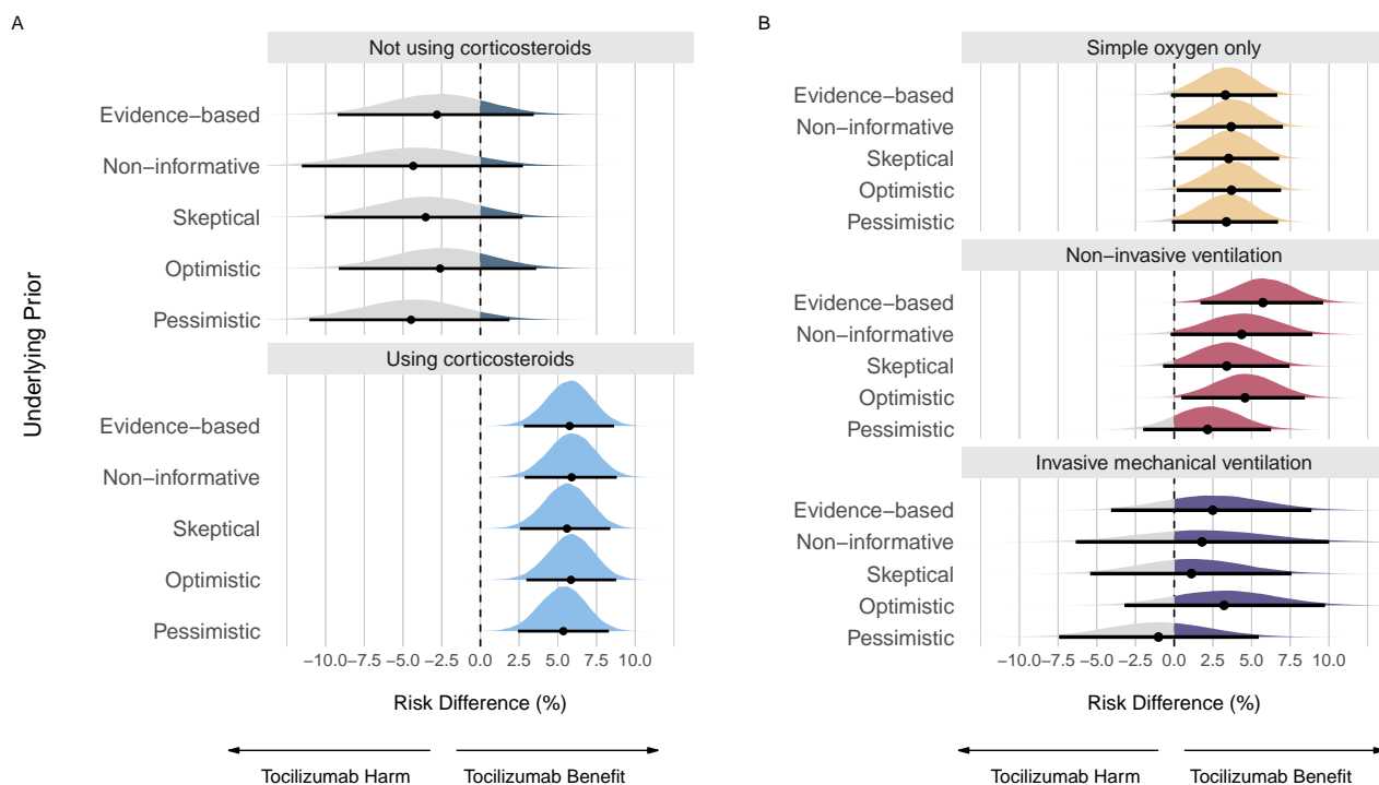
Figure 3. Posterior distributions from sensitivity analyses using different priors on the mortality outcome. Panel A shows posterior distributions on subgroups regarding use of corticosteroids. Panel B shows posterior distributions on subgroups regarding respiratory support. Point estimates depict the median and interval bars depict the 95% highest density intervals.
