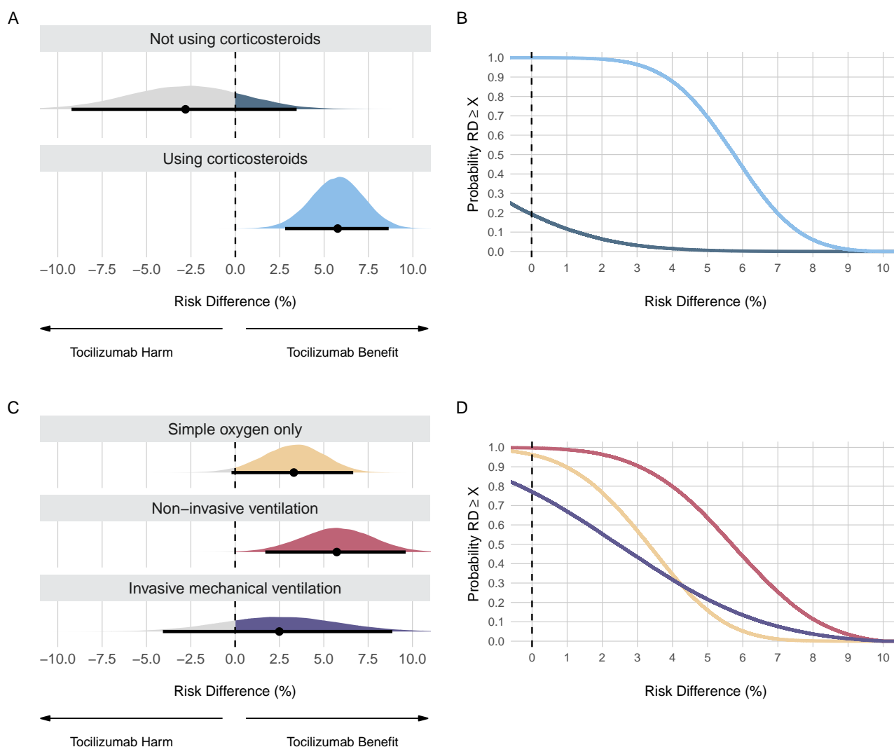
Figure 2. Posterior distributions and probabilities using evidence-based priors on the mortality outcome. Panel A shows the posterior distributions and Panel B shows the cumulative posterior probabilities on subgroups regarding use of corticosteroids. Panel C shows the posterior distributions and Panel D shows the cumulative posterior probabilities on subgroups regarding respiratory support. Panels A and C: Point estimates depict the median and interval bars depict the 95% highest density intervals. Panels B and D: Cumulative posterior distributions correspond to the probabilities that the risk difference (RD) is lower than or equal to the effect size on the X-axis. The colors in Panels B and D match the ones used in Panels A and C.
