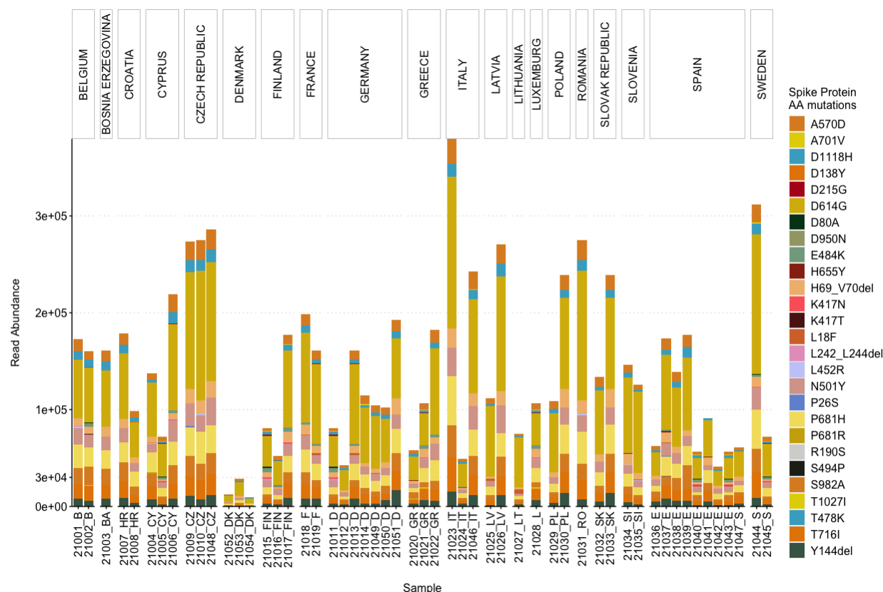
9 Fig 3: Abundance of the reads associated with Spike protein AA mutations used by the 10 ECDC for the characterization of the VOCs.
