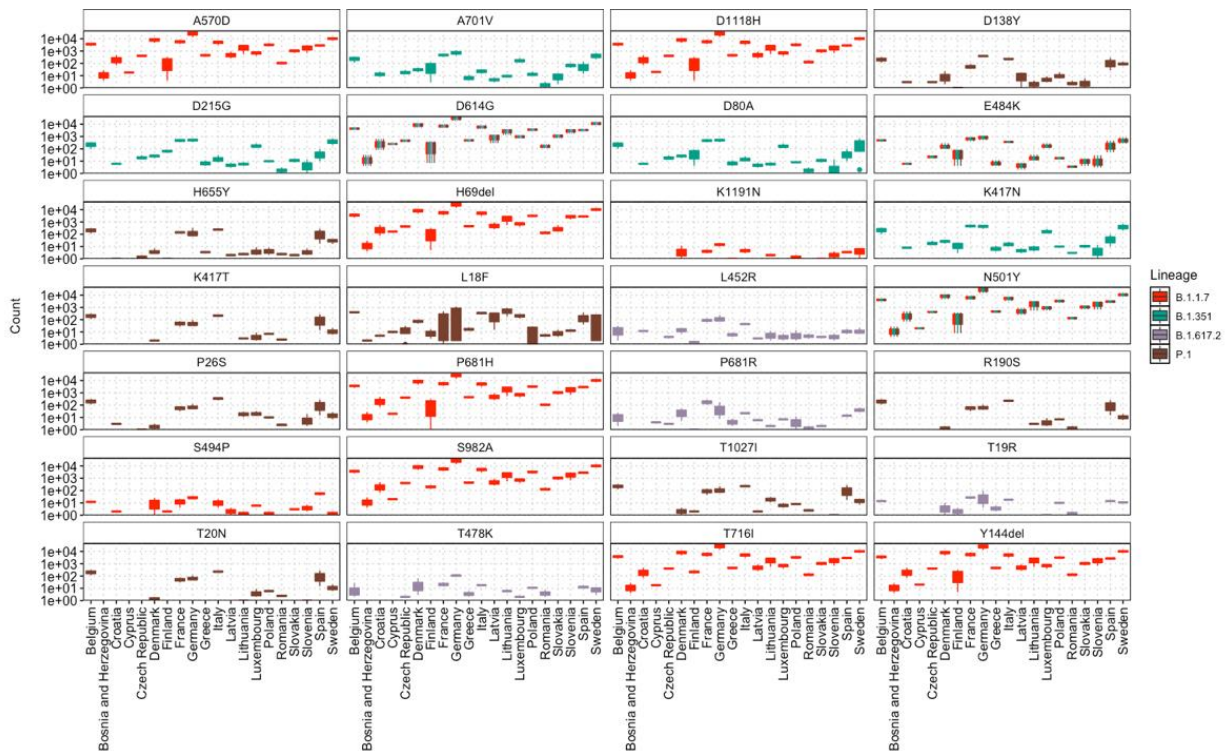
S.fig. 1: Count (occurrence of mutation in number of genome sequences submitted in GISAID) of spike protein mutations, which are considered for characterization of VOC by ECDC (5,6), found in the variant surveillance data for clinical samples of GISAID dated 31 st May 2021. The counts are presented in log 10 scale.
