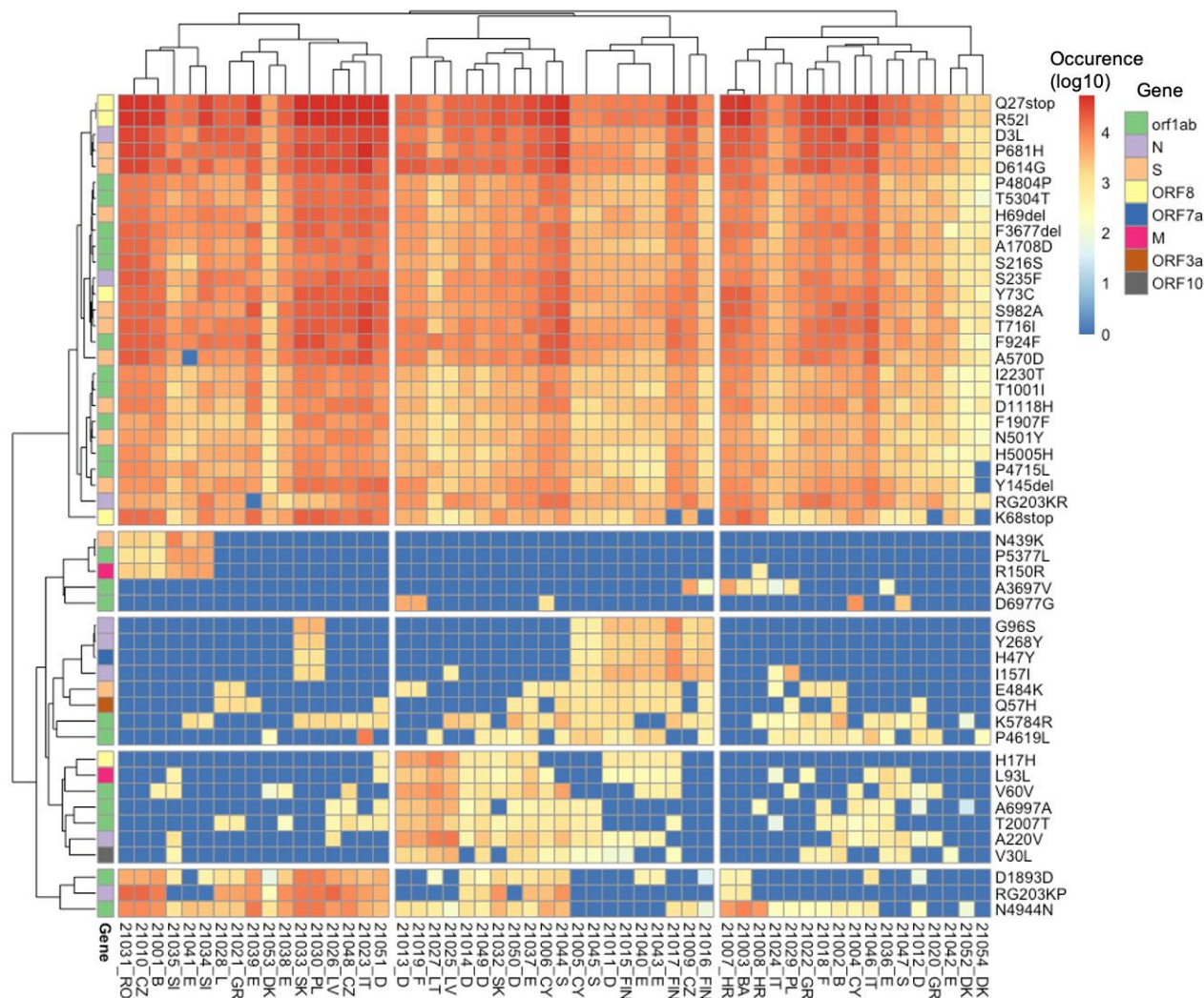
3 Fig 4: Heatmap showing the read abundance of the top 50 AA mutations found across all the 4 samples.
