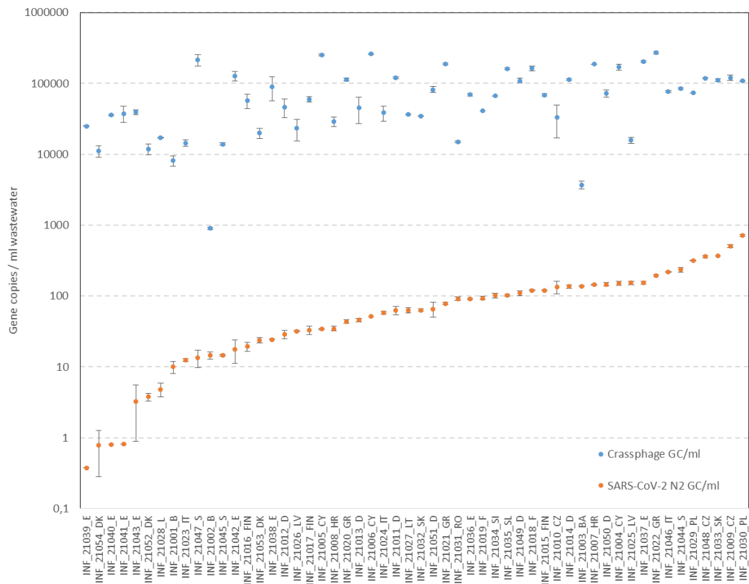
S.fig. 3: qPCR based analysis showing the concentration of SARS-CoV-2 N2 gene copies detected in each sample.
