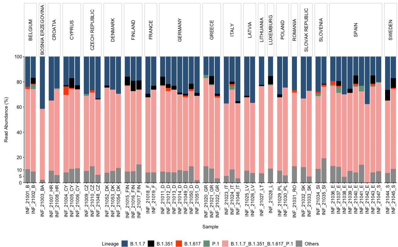
S.fig. 5: Relative abundance of the variants of concern (VOC) and other variants, based on the abundance of the reads associated with each SNP, respectively. AA mutations shared among different SARS-CoV-2 VOCs are represented as “B.1.1.7_B.1.351_B.1.617_P.1”.
