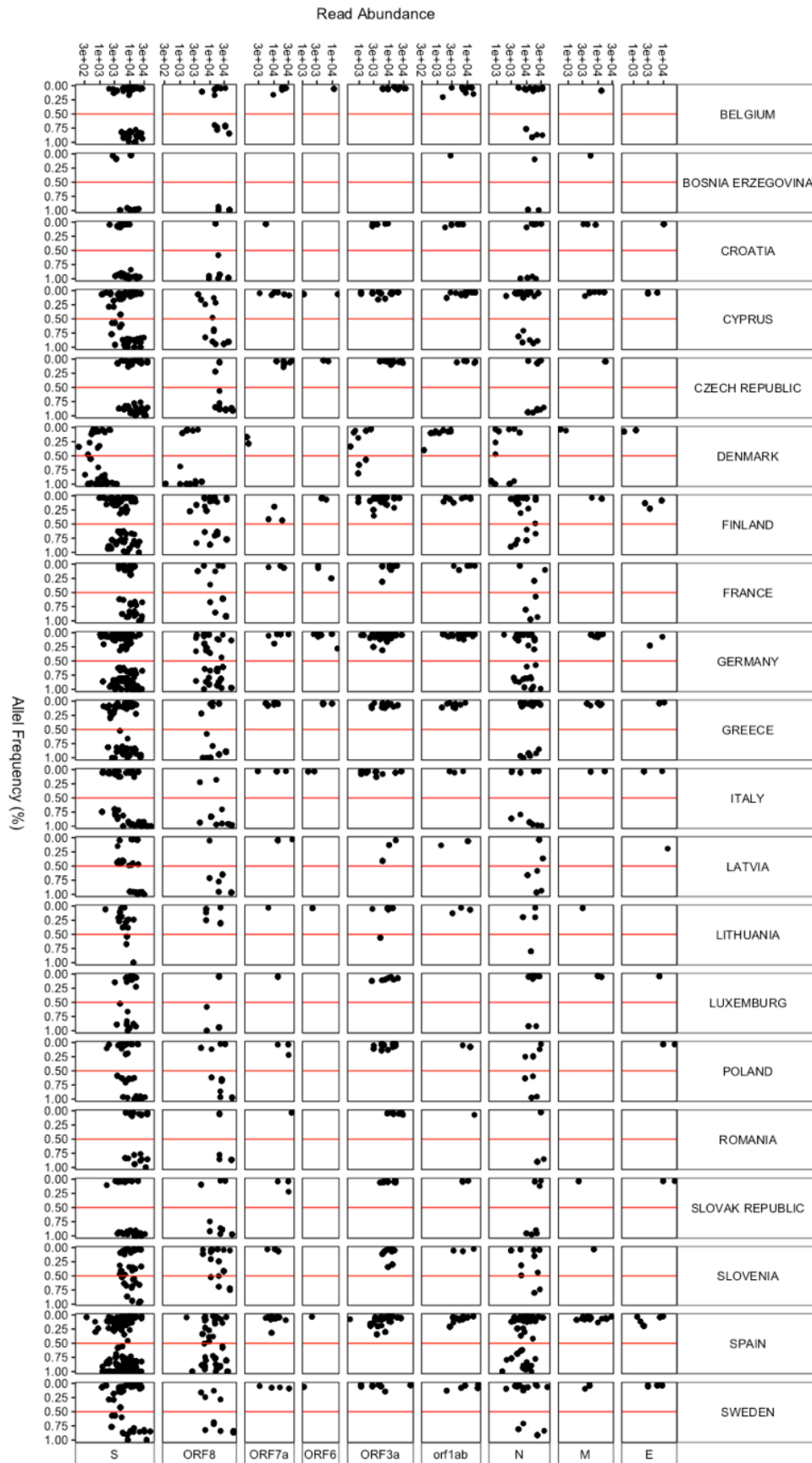
S.fig. 4: Scatter plot showing the distribution of the read abundance of each mutation against the allele frequency of each mutation.
