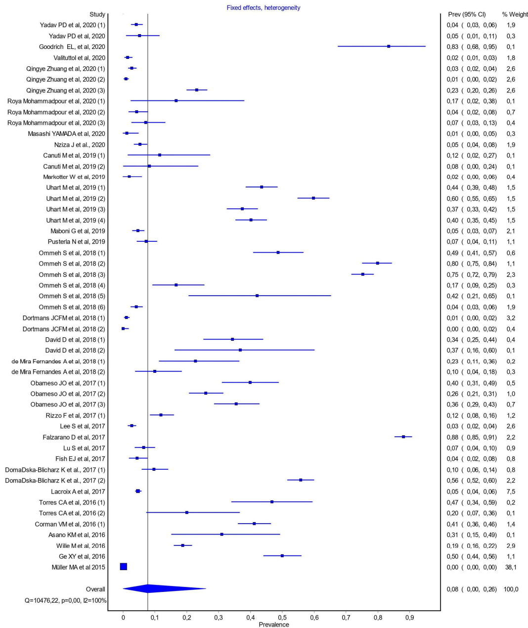
Figure 3. Results of metanalysis, Fixed effects, heterogeneity, Q = 10476.22 , p=0.00 and I^2=100\% .
