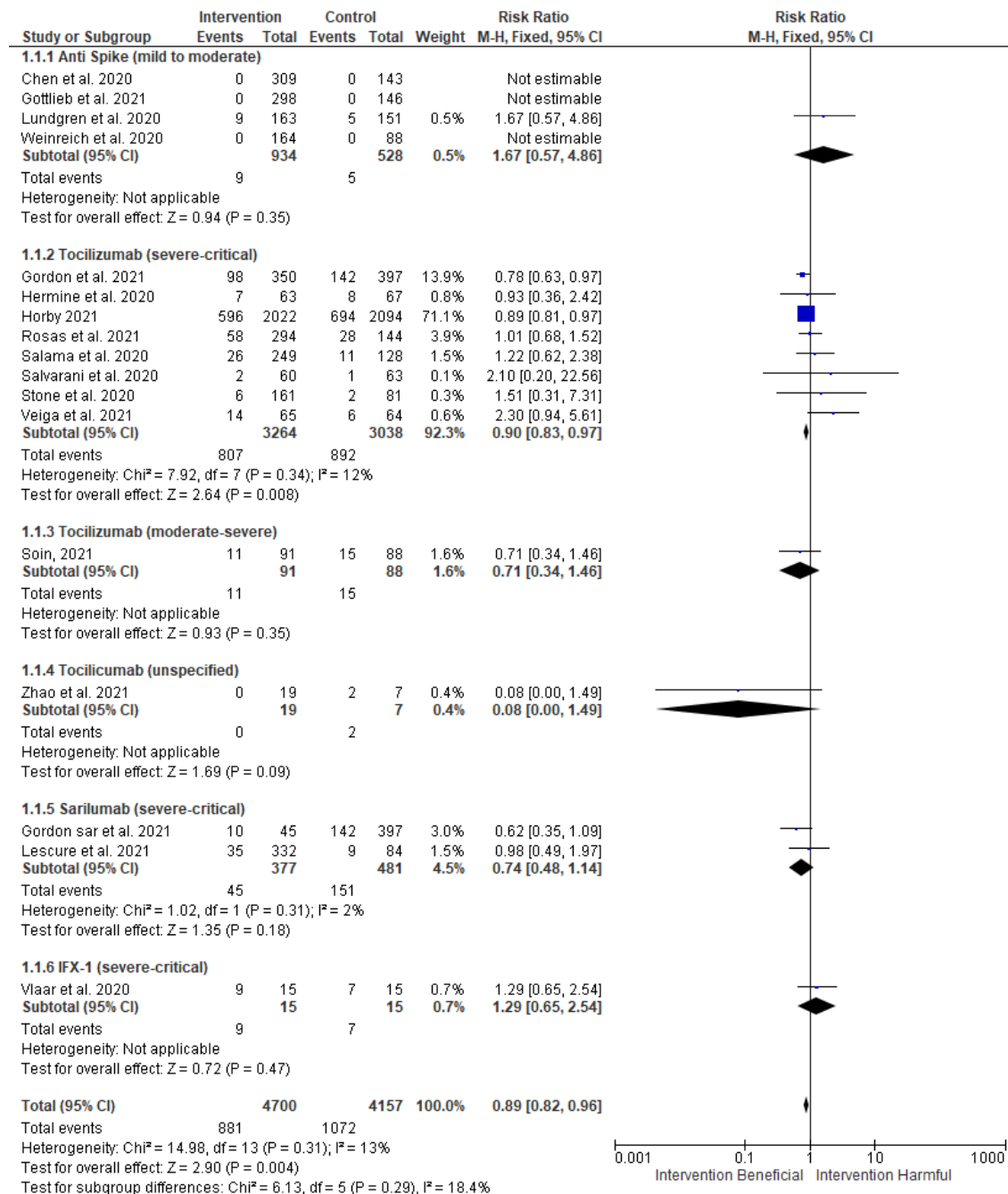
Figure 2 Subgroup analysis between types of monoclonal antibody and mortality among COVID-19 patients
