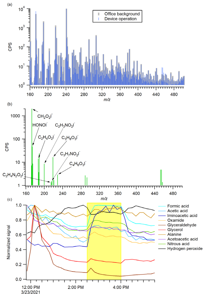
445 446 Figure 1. HR-ToF-CIMS results showing (a) grey: office background mass spectrum / blue: mass spectrum during 447 hydroxyl generator operation, (b) the mass spectrum difference between before and during the operation of hydroxyl 448 generator, and (c) time evolution of selected species. The data are 10-min averaged data and are normalized by the 449 maximum signal of each species. The hydroxyl generator was in operation from 2:30 pm to 4:00 pm (highlighted in 450 yellow). Glyceraldehyde ( m/z 217, \text{C}_3\text{H}_6\text{O}_3\text{I}^- ) is not included in the mass spectrum in (b) due to its rapid decay after 451 the formation.
