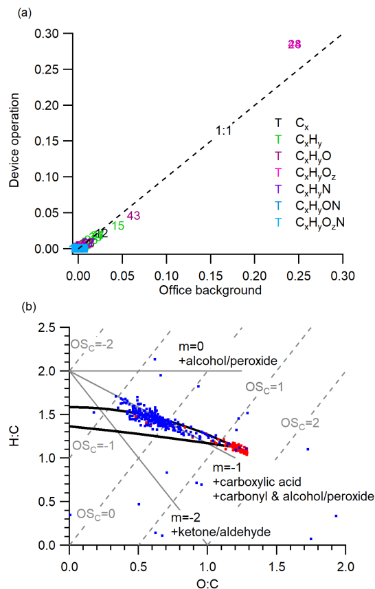
461 462 Figure 3. HR-ToF-AMS results showing (a) organic mass spectra comparison between during device operation and 463 office background and (b) VK-triangle diagram of organics. The black lines encompass the triangular space occupied 464 by ambient SOA. 44 The carbon oxidation states (OS C ) are shown with grey dotted lines. The blue data points 465 correspond to office background and the red data points correspond to device operation. 466 467
