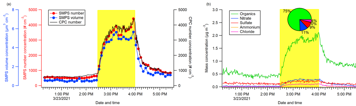
453 Figure 2. Time series of (a) particle number (CPC and SMPS) and volume concentrations (SMPS) and (b) non- 454 refractory species concentrations (HR-ToF-AMS). The mass fraction of different non-refractory species during the 455 hydroxyl generator operation is shown in the pie chart. The hydroxyl generator was in operation from 2:30 pm to 4:00 456 pm (highlighted in yellow).
