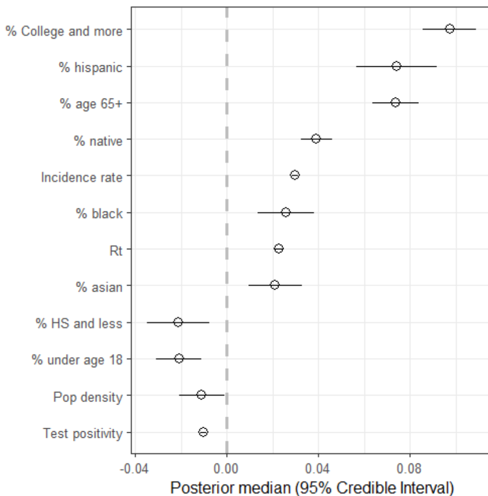
Figure 2. Estimated coefficients of time-fixed and time-varying US county effects from the selected spatio-temporal Beta regression model with a probit link, sorted by absolute magnitude. All covariates were centered and scaled prior to analysis. Vaccination data cover February 21, 2021 through May 16, 2021.
