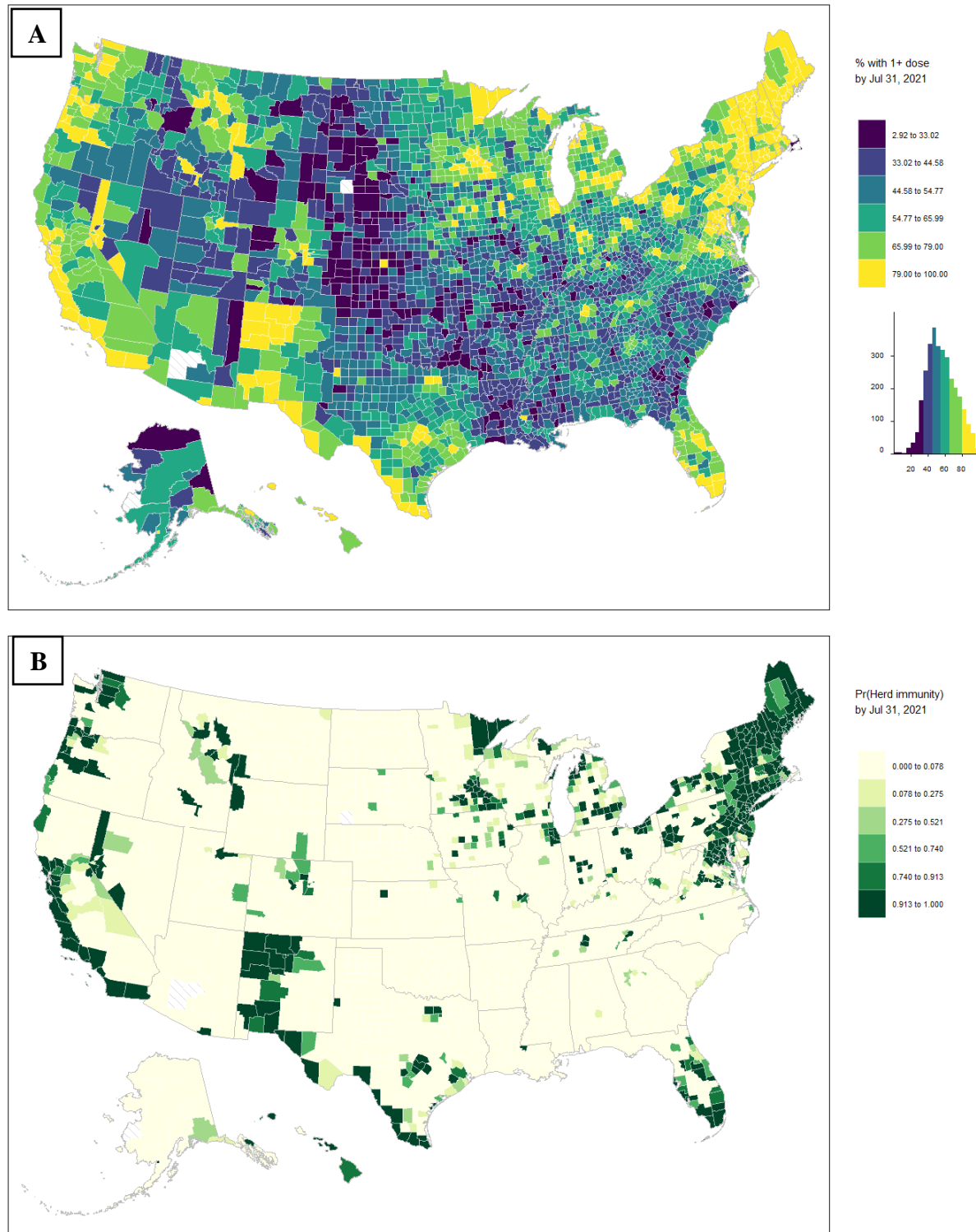
Figure 5. Forecasted percentage of residents with at least one dose by US county for the week ending on July 31 (July 25 – 31) (A) and estimated probability of local herd immunity, i.e. \Pr(\text{prediction} > 70\%) (B). Diagonal hatch pattern indicates missing data, which occurs in Alaska, Arizona, and South Dakota. Forecast is based on data from February 21, 2021 through May 16, 2021.
