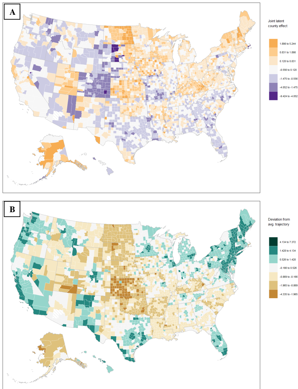
Figure 3. Standardized time-averaged joint (spatial + unstructured) county effects (A) and standardized deviations from the typical trajectory (B). Values > 0 indicate a county is over-performing its known characteristics; values < 0 indicate a county is under-performing its known characteristics. Diagonal hatch pattern indicates missing data, which occurs in Alaska, Arizona, and South Dakota. Vaccination data cover February 21, 2021 through May 16, 2021.
