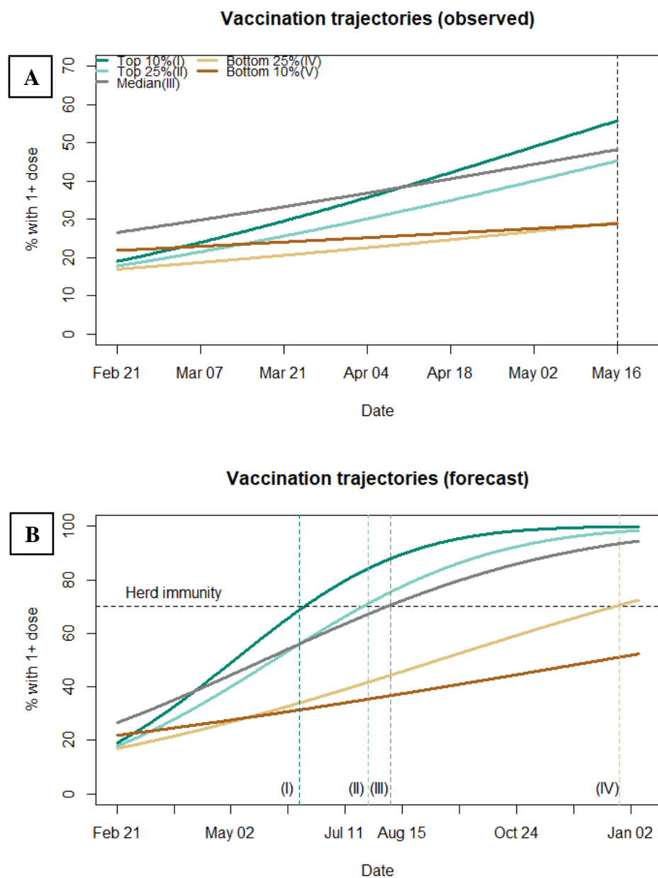
Figure 4. Fitted and forecasted trajectories for representative counties in the top 10%, top 25%, median, bottom 25%, and bottom 10% of estimated trajectories. Vaccination rates for the previous 13 weeks of data as of May 16, 2021 (A) and forecasted vaccination rates (B) are shown. Dashed horizontal line indicates the herd immunity threshold of 70%. Counties in the top 10% of estimated trajectories are expected to reach herd immunity by the week of Jun 13–19 (I); top 25% by the week of Jul 25–31 (II); median county by the week of Aug 8–14 (III); bottom 25% by the week of Dec 26, 2021 – Jan 1, 2022 (IV); bottom 10% not until later in 2022.
